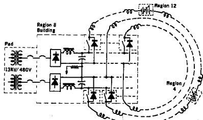
Fig. 1 PEP Chopper System Functional Schematic
