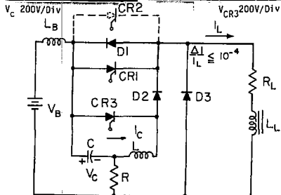
Fig. 5. Current-commutated Chopper Circuit
