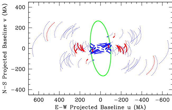
Figure 4. Detections of fringes as a function of position in the plane of baselines perpendicular to the line of sight. GBT-VLBA baselines are shown as red lines, VLBA-VLBA as blue. Detections are solid lines, non-detections dotted. The green ellipse shows the best-fitting average scattering disk, expressed as the baseline where correlated flux density reaches e^{-4} \approx 0.018 of maximum. Detections on shorter VLBA baselines, within the ellipse, show the large-scale scattering disk. Detections on long GBT-VLBA baselines indicate substructure within the disk.
