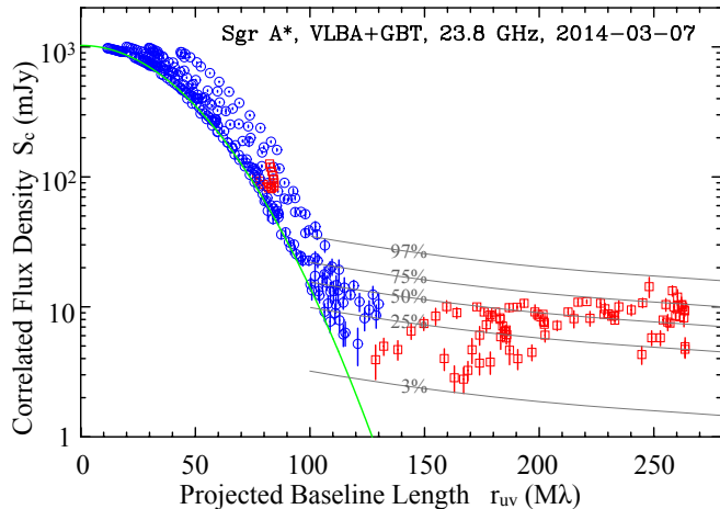
Figure 2. Correlated flux density of Sgr A* at \lambda = 1.3 cm plotted against baseline length. Squares show the sensitive GBT-VLBA baselines, circles VLBA-VLBA baselines. Each point represents a 15-min vector average for one baseline after self-calibration; error bars show statistical \pm 1\sigma . The green curve shows the correlated flux density of the average scattering disk for an East-West baseline, as described in Sec. 2. The gray curves show quantiles of the predicted distribution of correlated flux density from substructure, with source and scattering parameters from Bower et al. (2006, 2014b), as described in Sec. 3 below.
