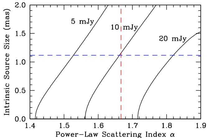
Figure 5. Expected root-mean-square level of refractive noise, S_{\text{rms}} , on a 3000-km E-W baseline ( 230 G\lambda ) as a function of the power-law index of the spectrum of density fluctuations, \alpha , and the intrinsic size (FWHM) of the source \theta_{\text{src}} along the baseline direction. Each of the three curves is calculated assuming that the diffractive scale and anisotropy are determined by extrapolating longer-wavelength measurements; the scattering geometry determined by Bower et al. (2014a) is assumed. The horizontal dashed line shows the intrinsic size inferred from deconvolution (Bower et al. 2006); the dashed vertical line shows the index \alpha expected for a Kolmogorov spectrum. Samples on other baselines, or at another frequency, would break the degeneracy between \alpha and \theta_{\text{src}} . Note that, because the amplitude of refractive noise is drawn from a Rayleigh distribution, its mean amplitude is (\sqrt{\pi}/2)S_{\text{rms}} \approx 0.89S_{\text{rms}} and its median amplitude is \sqrt{\ln 2}S_{\text{rms}} \approx 0.83S_{\text{rms}} .
