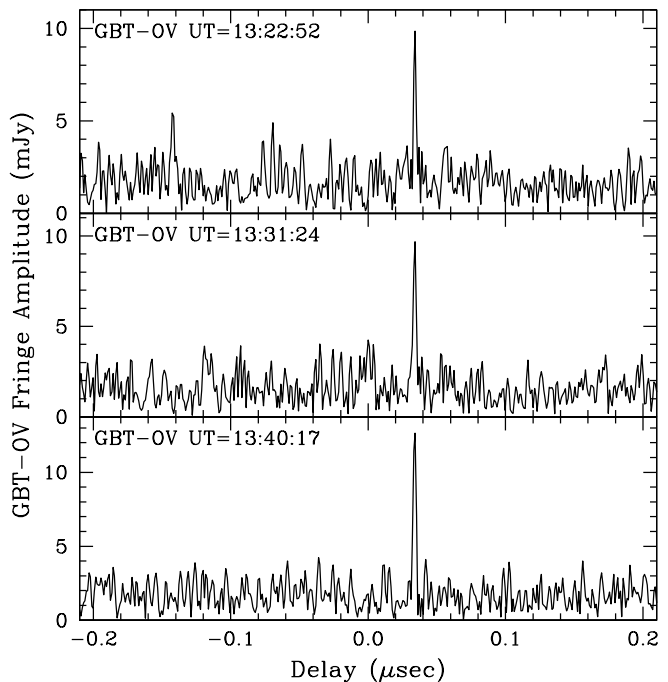
Figure 3. Fringes on Sgr A* on the 3000-km GBT-Owens Valley baseline. To make this plot, we Fourier transformed the data from the correlator, expressed as the complex visibility function as a function of frequency channel and time, to the domain of delay and fringe rate. We located the highest peaks in that domain for each interval, and display them here as a function of delay. The average scattering disk has correlated flux density, of < 10^{-6} mJy on this baseline. The probability of false detection is < 10^{-9} for each of the 3 peaks.
