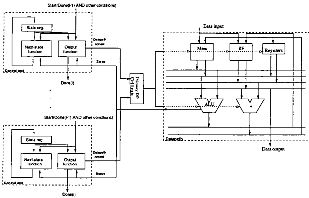
Figure 52: A FSM implementation with a decomposed-CU
