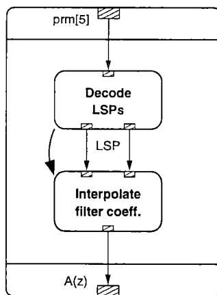
Figure 66: LSP decoding
