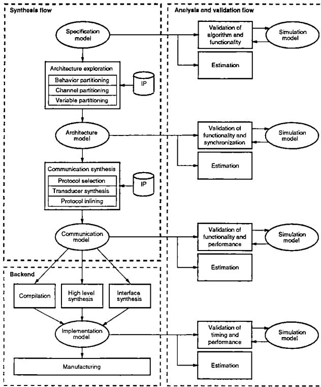
Figure 2: SpecC methodology.
