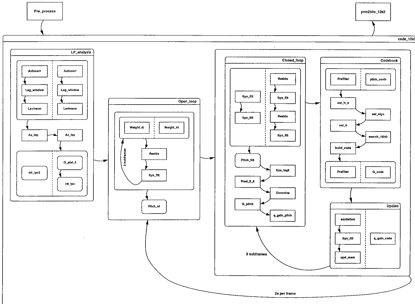
Figure 64: Coder block diagram.
