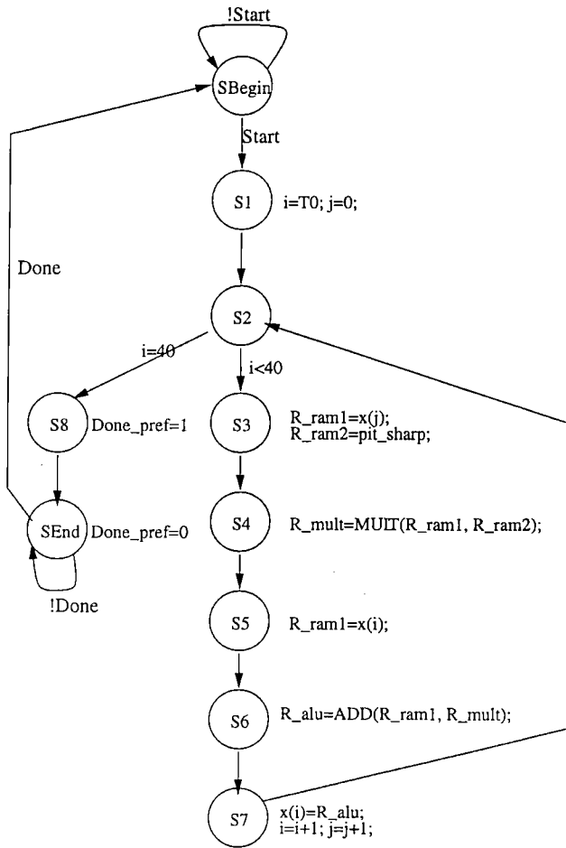
Figure 50: Behavior prefilter FSM.
