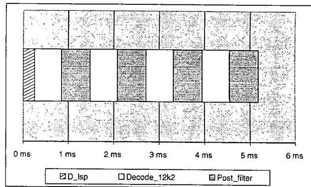
Figure 17: Initial decoder delay.
