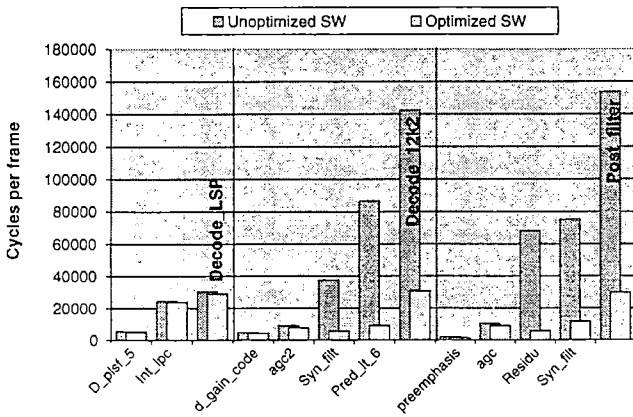
Figure 30: Breakdown of decoder delays after exploration.
