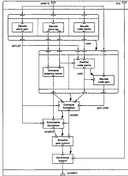
Figure 67: Subframe decoding
