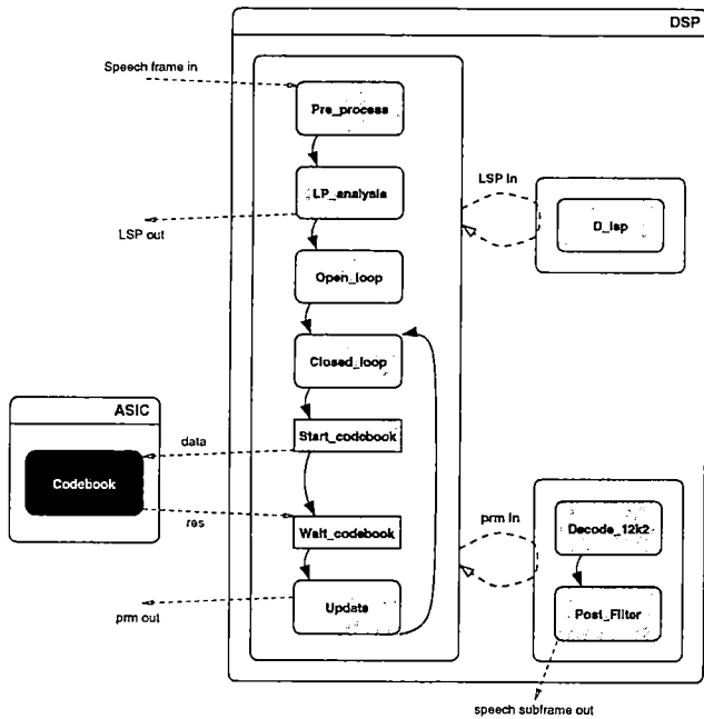
Figure 28: Final dynamic scheduling of vocoder tasks.
