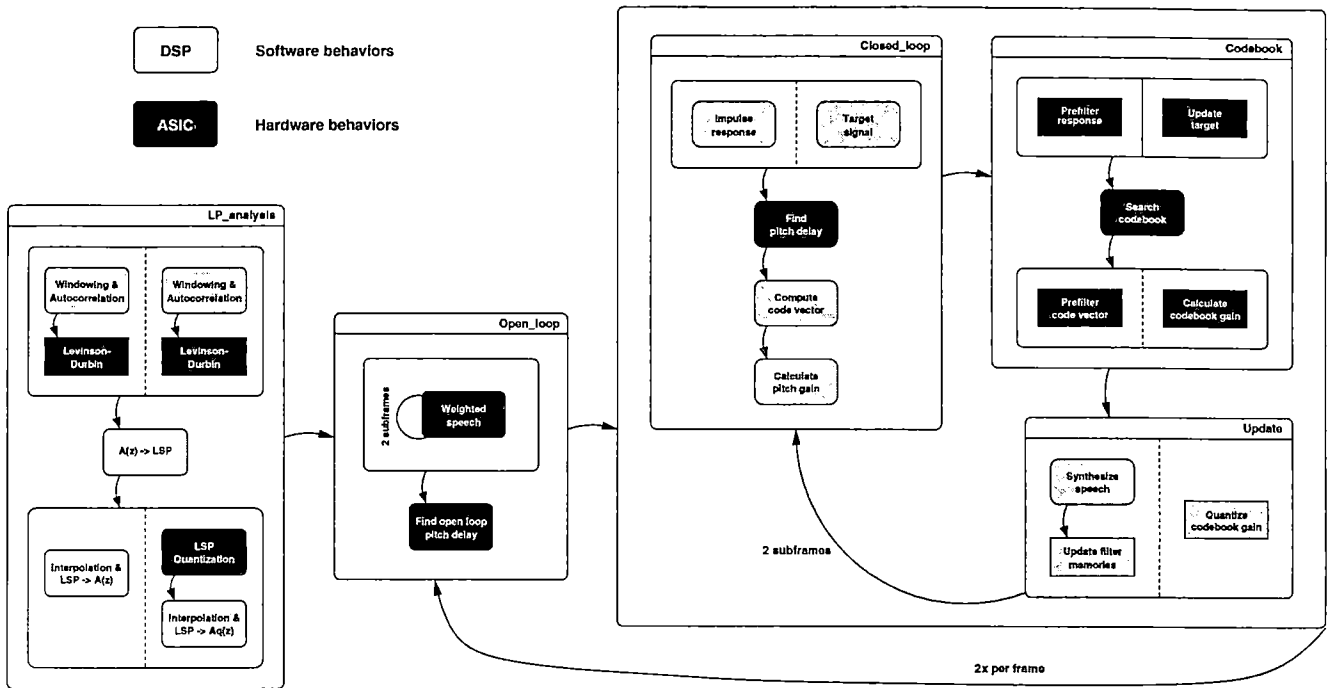
Figure 22: Example of an encoder partitioning.
