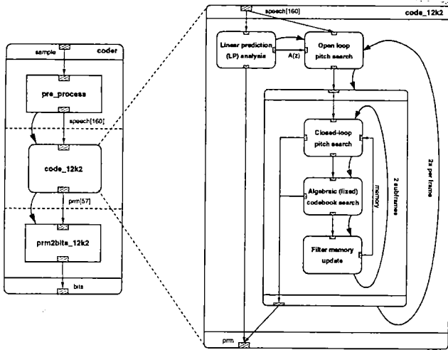
Figure 4: Coder.
