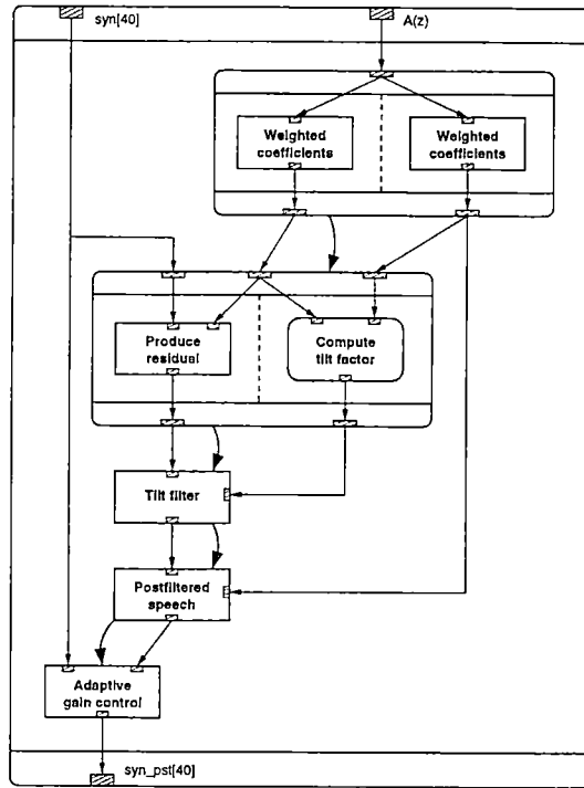
Figure 68: Post filtering
