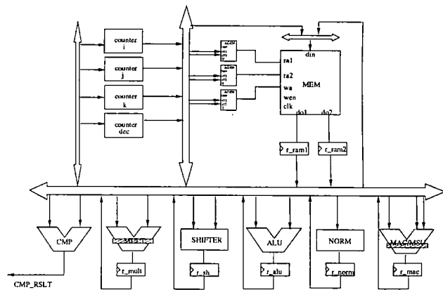
Figure 51: Datapath diagram.
