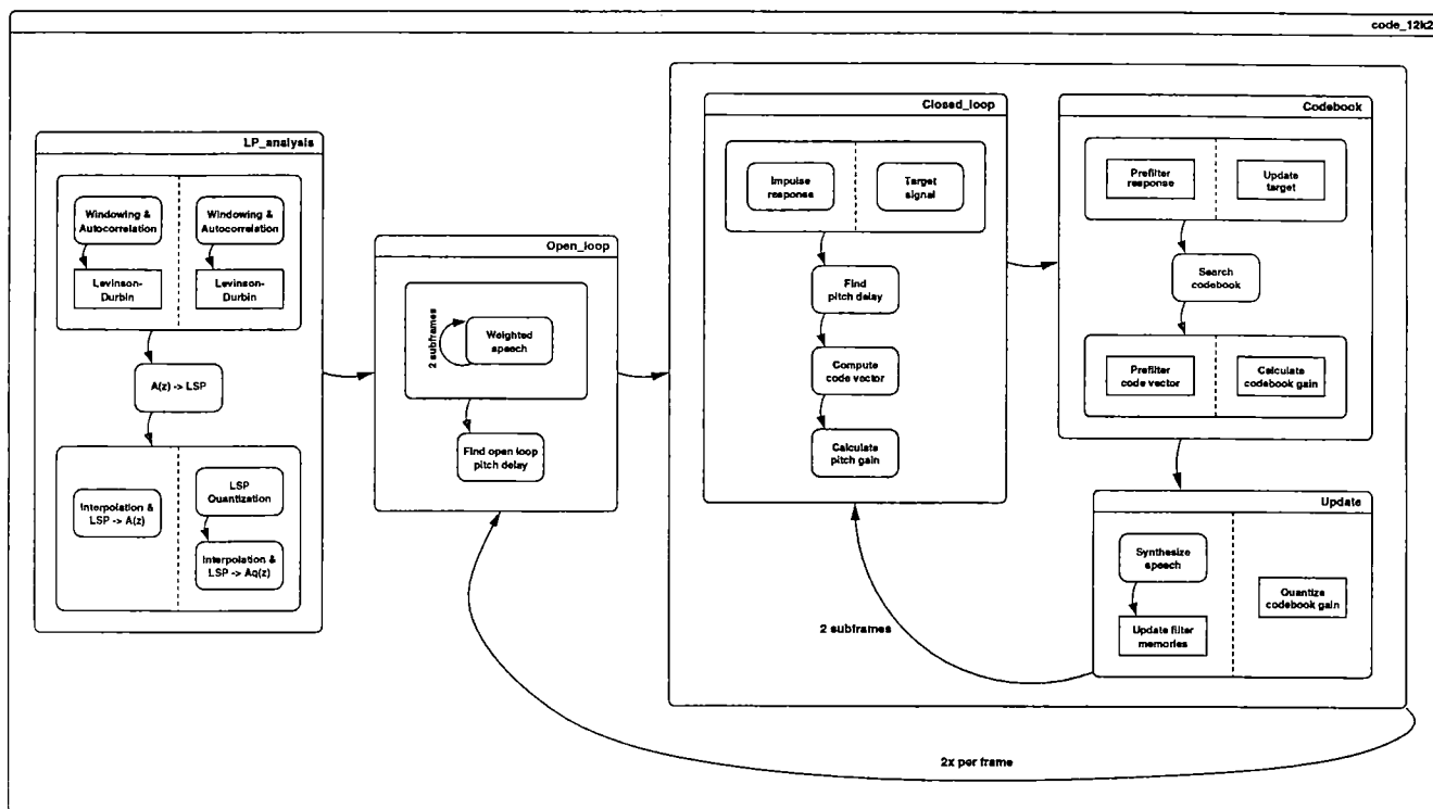
Figure 5: Encoding.
