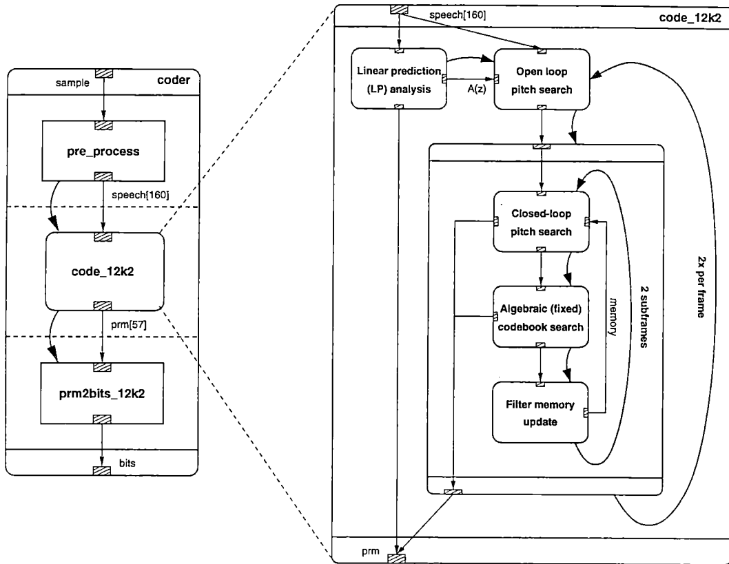
Figure 58: Coder
