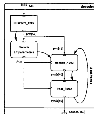
Figure 6: Decoder.
