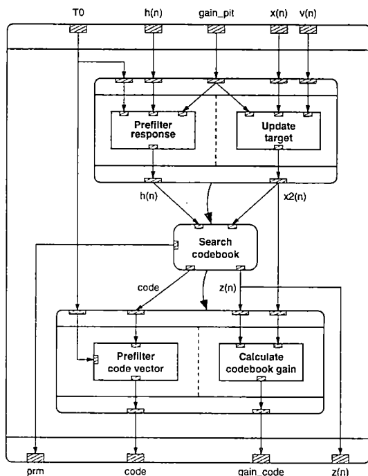
Figure 62: Algebraic (fixed) codebook search
