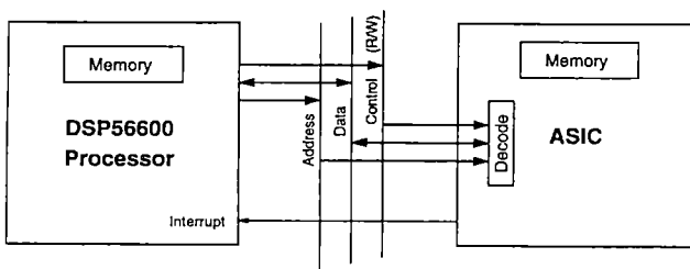
Figure 37: Vocoder hardware/software interfacing model.
