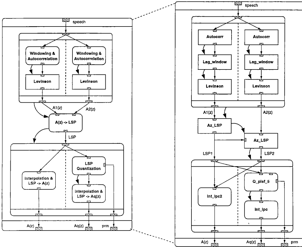
Figure 59: LP Analysis
