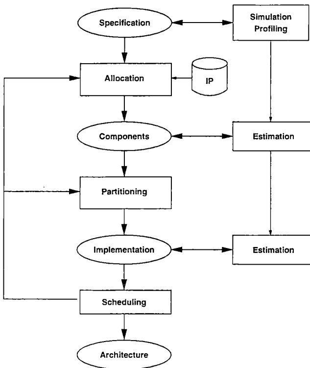
Figure 10: Architectural exploration flow.
