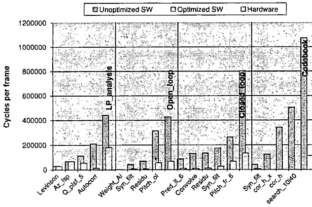
Figure 29: Breakdown of coder delays after exploration.
