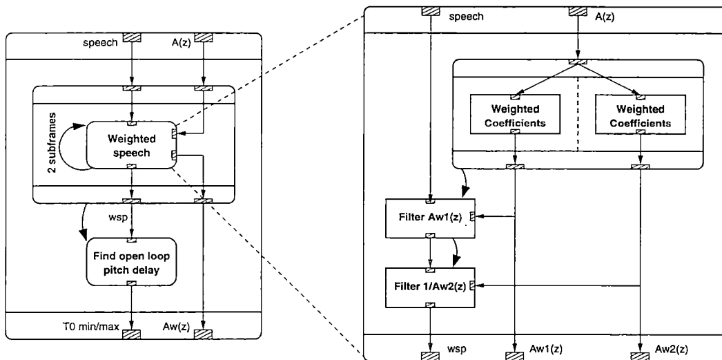
Figure 60: Open-loop pitch analysis
