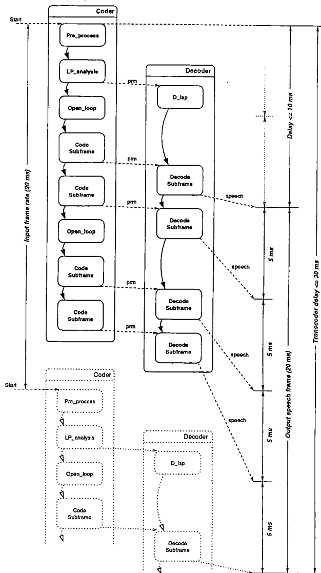
Figure 7: Timing constraints.
