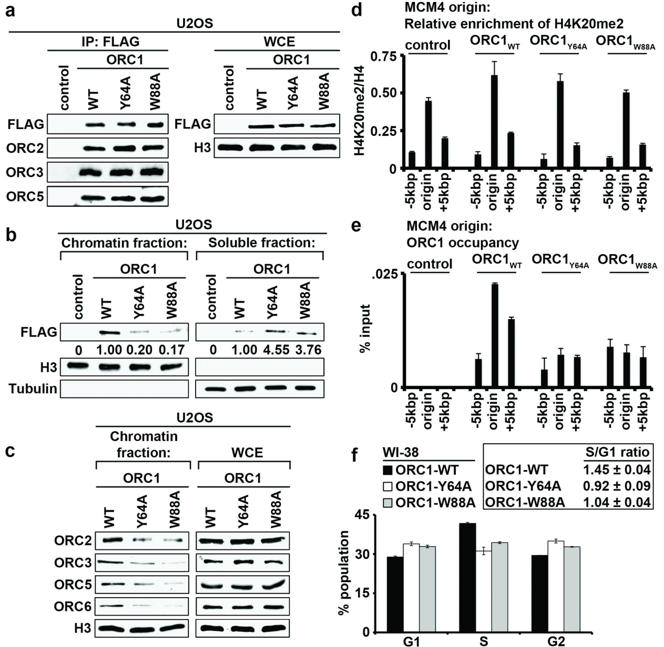
Figure 3. ORC1-H4K20me2 interaction regulates ORC chromatin association and cell cycle progression
