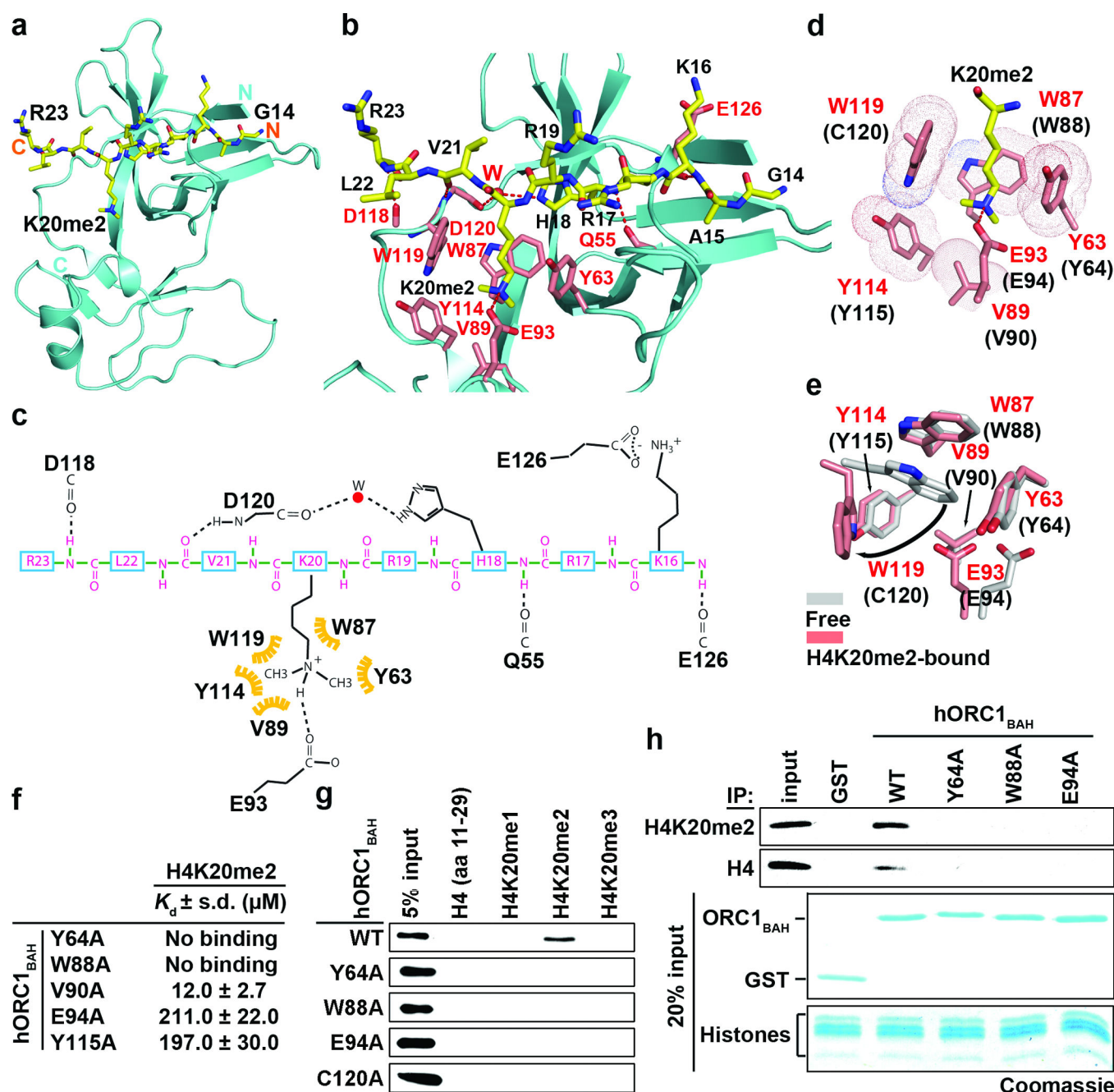
Figure 2. The molecular basis of H4K20me2 recognition by ORC1 BAH a–c , 1.95 Å crystal structure of murine ORC1 BAH aa 9–170 (mORC1 BAH ) complexed with H4(14–25)K20me2 peptide. a , Ribbon representation of mORC1 BAH bound to H4K20me2 peptide. The mORC1 BAH (cyan) and the bound H4K20me2 peptide (yellow) are shown in ribbon and stick representations, respectively. b , Details of intermolecular contacts in the mORC1 BAH -H4K20me2 complex. mORC1 BAH and H4K20me2 peptide residues are colored in pink and yellow, respectively, with hydrogen bonds depicted as red dashed lines, and a water molecular as a red sphere. c , Schematic representation of intermolecular contacts in the mORC1 BAH -H4K20me2 complex. The residues from the H4K20me2 peptide
