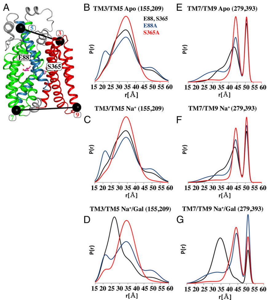
Fig. 7. Nonfunctional mutants display impaired formation of the \text{Na}^+ /Gal state. DEER analysis for TM3/TM5 and TM7/TM9 was performed on the background of the active constructs (black), a \text{Na}^+ site inactivating mutation, S365A (red), and a sugar site inactivation mutant, E88A (blue). A cartoon representation of the labeling sites (black spheres connected by black lines), galactose (in sticks), \text{Na}^+ (pink sphere), and the two side chains involved in ligand and sodium binding (sticks) are shown in A. Ligand-dependent distance distributions under the Apo, \text{Na}^+ , and \text{Na}^+ /galactose conditions are shown for TM3/TM5 (B–D), respectively, and for TM7/TM9 (E–G). Disruption of the \text{Na}^+ or sugar binding sites alters the conformational distributions sampled by vSGLT in all solution states and prevents the formation of the \text{Na}^+ /galactose-bound conformation sampled by the active protein.
