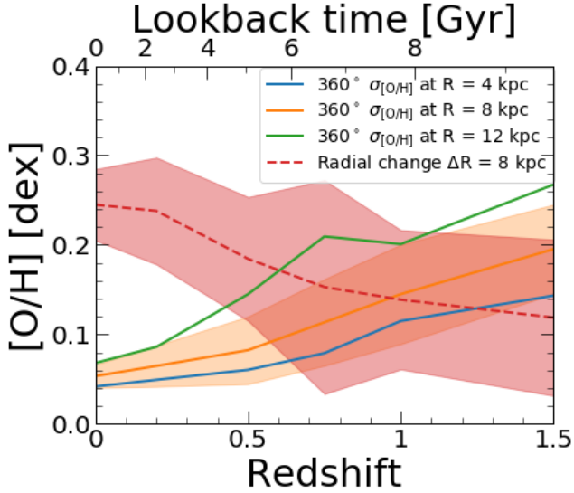
Figure 9. The evolution of variations in [O/H] in gas, both radially and azimuthally. (We do not show [Fe/H] , its trends are consistent with [O/H] to \lesssim 0.01 dex.) The solid lines show the mean scatter, across our 11 galaxies, for the full ( 360^\circ ) annulus of gas at R = 4 kpc (blue), R = 8 kpc (yellow), and R = 12 kpc (green). The red dashed line shows the mean radial change in [O/H] across a radial distance of 8 kpc. The shaded regions show the 1-\sigma scatter. While the radial gradient dominates the spatial variations at late cosmic times, azimuthal variations were more significant than the radial gradient at earlier cosmic times ( z \gtrsim 0.9 , or t_{\text{lookback}} \gtrsim 7.4 Gyr, at R = 8 kpc). Larger radii transition to radially dominated abundance variations at later times (see also Fig. 10). Thus, elemental evolution models should not assume azimuthal homogeneity of abundances at early times; instead, azimuthal variations are the primary source of spatial information for chemical tagging of stars forming at early times.
