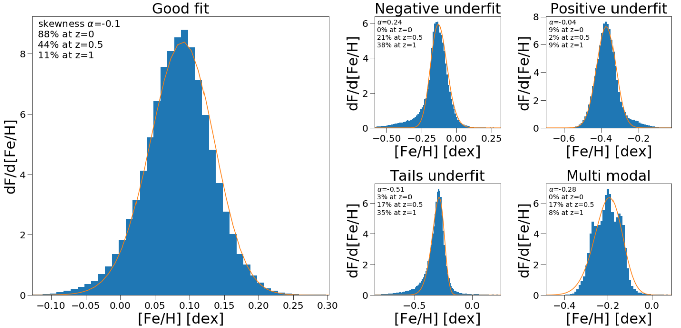
Figure 13. Example distributions of [\text{Fe}/\text{H}] from our 11 galaxies. Each panel shows the elemental distribution for a single simulation at a single radius. For each distribution, we stack 3 consecutive snapshots ( \Delta t \approx 50 Myr) and measure all gas within \pm 0.2 kpc of 3 radii ( R = 4, 8, and 12 kpc) and within a height \pm 1 kpc of the disk. The solid line shows a skew normal fit to the distribution. The left panel shows a well fit skew normal distribution. The right panel shows typical failure modes of fitting a skew normal distribution: underfitting negative skewness, underfitting positive skewness, underfitting the tails of the distribution, and multi modal distributions. Each panel shows the fitted skewness for the example distribution along with the percentage of fits that fall into the category at each redshift across all radii and for both [\text{O}/\text{H}] and [\text{Fe}/\text{H}] . In general, the simulations are well fit by a skew normal at z = 0 , but it provides a worse fit at higher redshift, when the (negative) tails are preferentially underfitted. In general, the fit to the distribution of [\text{O}/\text{H}] and [\text{Fe}/\text{H}] for the same R and redshift fall into the same category.
