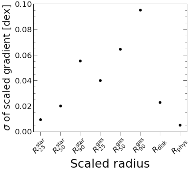
Figure A1. The 1\text{-}\sigma host-to-host scatter of the scaled radial gradients for different scale radii at z = 0 . We define R_{25} , R_{50} , and R_{90} for the gas and stars in Table 1. R_{\text{disk}} is the exponential scale length of the stellar disk determined via a 2-component fit to the surface density, and R_{\text{phys}} is the physical radial coordinates of the disk, i.e. unscaled coordinates. For each scale radius, we measure the gradient of all galaxies across an equal radial range that corresponds to 4 – 12 kpc physical for the galaxy with the median scale length. The 1\text{-}\sigma host-to-host scatter is smallest when measuring the gradients in physical space, which motivates our choice for our analysis in this paper.
