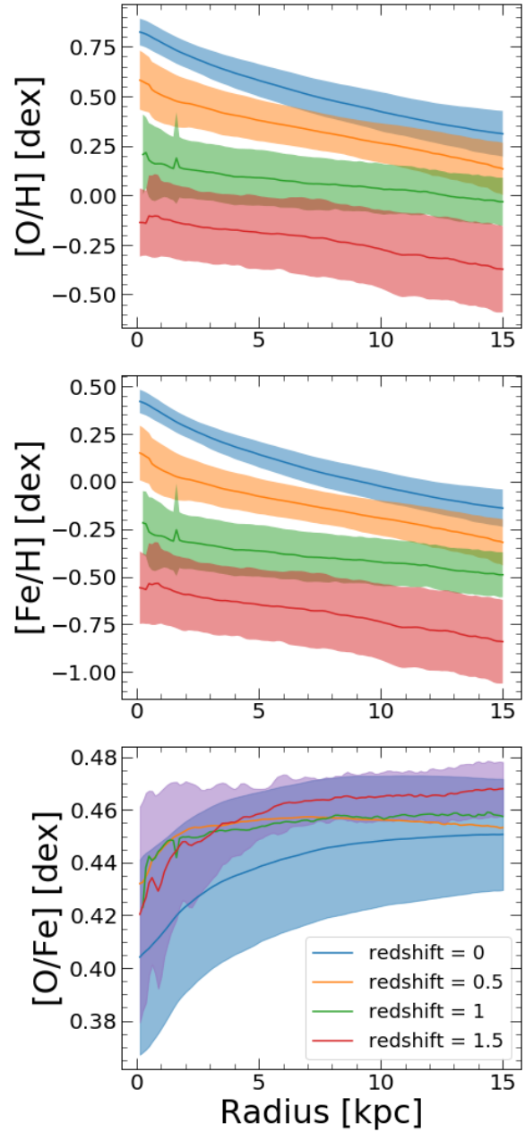
Figure 4. Radial profiles of gas-phase elemental abundances in our simulations at different redshifts. The solid lines show the mean and the shaded regions show the 1\text{-}\sigma scatter across our 11 galaxies. The top and middle panels show steepening radial profiles of [O/H] and [Fe/H] with time, as the gas disk becomes more rotation dominated, with less radial turbulence, thus sustaining stronger radial gradients. The bottom panel shows that the innermost regions of the gas disk have lower [O/Fe] than the outer disk, this indicates that the inner disk is more evolved, that is, has had more Ia supernovae that produce more Fe than \alpha -elements (like O), than the outer disk.
