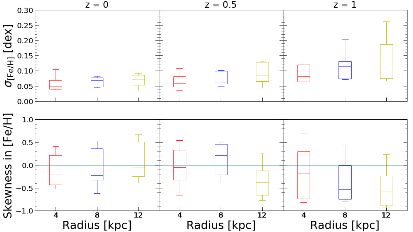
Figure 14. Top: standard deviation of the fitted elemental distribution of gas [\text{Fe}/\text{H}] at 3 radii, for increasing redshift (left to right). For each distribution, we stack 3 consecutive snapshots ( \Delta t \approx 50 Myr) and measure all gas within \pm 0.2 kpc of each radius and within a height \pm 1 kpc of the disk. Each box shows the 68th percentile of the distribution and the whiskers show the full distribution of standard deviations. The standard deviation increases with radius and decreases with time. Bottom: skewness of the fitted elemental distributions of gas [\text{Fe}/\text{H}] . At earlier times, the gas disk had stronger negative skewness, but the disk relaxes to near zero skewness at z = 0 . The skewness shows a slight radial dependence at both z = 1 ( t_{\text{lookback}} = 7.8 Gyr) and z = 0 . At z = 1 the distributions at larger radii were more negatively skewed, whereas at z = 0 the distributions at smaller radii are more negatively skewed.
