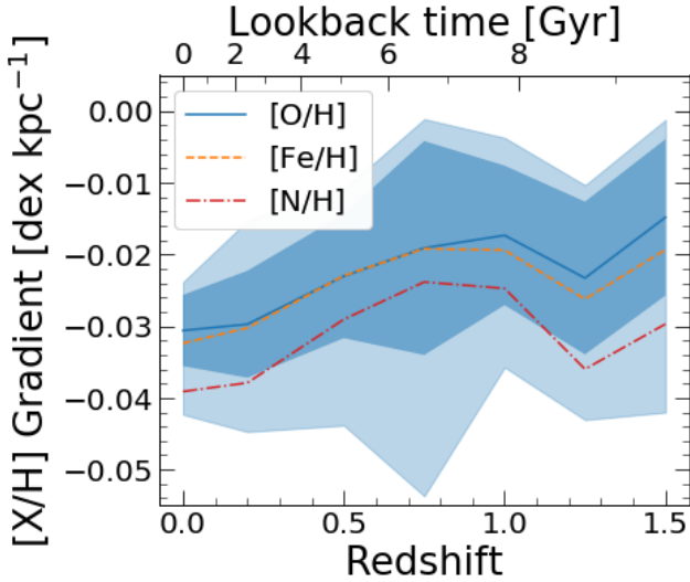
Figure 5. Evolution of radial gradients in gas elemental abundances. The lines show the means for [O/H], [Fe/H], and [N/H]. The dark shaded region shows the 1\text{-}\sigma scatter and the light shaded region shows the total scatter in [O/H] across our 11 galaxies. At each redshift we calculate the gradient via a linear fit across a redshift-dependent radial range: 4 < R < 12 kpc for z < 1 ( t_{\text{lookback}} < 7.8 Gyr) and 0 < R < 8 kpc for z \geq 1 . The gradient is flattest ( \approx -0.015 dex kpc ^{-1} ) at z = 1.5 ( t_{\text{lookback}} = 9.4 Gyr), likely because high merger rates drive large scale radial turbulence, erasing the radial gradients of the disks. This leads to the azimuthally averaged metallicity at a given radius showing little radial dependence although stochastic enrichment/accretion events may lead to locally over or under-enriched regions. Shallow gradients persist until z \approx 1 . At lower redshifts, the gas disk becomes more rotationally supported and is capable of sustaining stronger radial gradients, becoming steepest ( \approx -0.03 dex kpc ^{-1} ) at z = 0 . The gradients of [O/H] and [Fe/H] are almost identical, despite being sourced primarily by core-collapse and Ia supernovae, respectively. However, the [N/H] gradient, sourced primarily through stellar winds from massive stars, which have a metallicity dependent mass loss rate, is steeper at all times.
