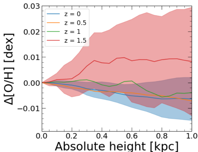
Figure 6. The vertical change in [O/H] relative to the midplane at various redshifts. We measure the vertical profile at R = 7 - 9 kpc. The solid lines show the mean while the shaded region shows the 1-\sigma standard deviation across 11 galaxies. [O/H] shows minimal variation with height: the mean deviation at 1 kpc above the midplane is \approx 0.008 dex at z = 1.5 ( t_{\text{lookback}} = 9.4 Gyr) and \approx -0.006 dex at z = 0 . The majority of stars form within a few hundred parsecs of the galactic midplane at low z and within \sim 1.5 kpc of the midplane at the highest redshift we examine. Close to the plane of the disk ( |Z| \leq 200 pc) the variation in [O/H] is even smaller at all times ( |\Delta[\text{O}/\text{H}]| \lesssim 0.001 dex at z = 1.5 and |\Delta[\text{O}/\text{H}]| \lesssim 0.002 dex at z = 0 ). At z < 1 ( t_{\text{lookback}} < 7.8 Gyr) we find a weak but systematically negative gradient. We conclude that vertical gradients are not measurably significant for chemical tagging at any redshift.
