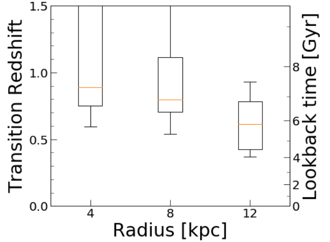
Figure 10. Following Fig. 9, the redshift below which radial variations in [O/H] dominate over azimuthal variations at 3 radii in our 11 simulations (the intersection of the dashed and solid lines). The horizontal line shows the median, the box shows the 68th percentile, and the whiskers show the full distribution. At R = 4 kpc two hosts have no transition redshift and at R = 8 kpc one hosts has no transition redshift, that is, the radial variation is always stronger than azimuthal scatter for the redshift range we observe. This transition redshift is the last time the azimuthal variation is stronger than the radial variation. This transition occurs earlier at smaller radii, where azimuthal variations are smaller (Fig. 7), given the shorter timescale for mixing at smaller radii. Before these transition redshifts, any model of chemical tagging should account for azimuthal variations as the primary source of spatial variation.
