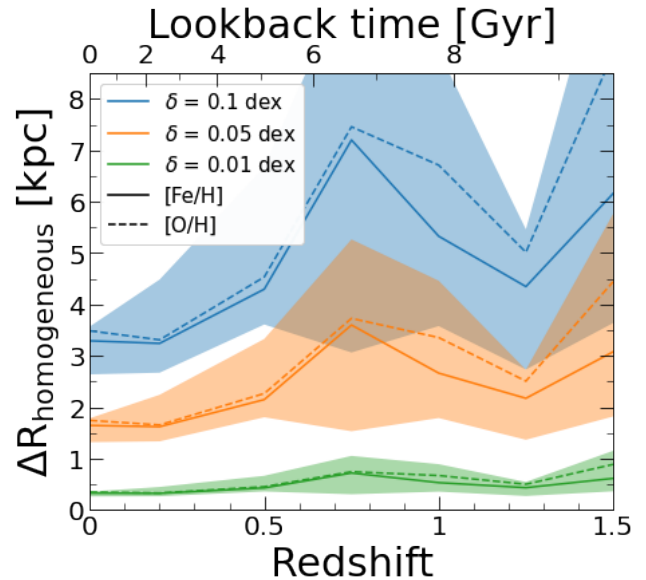
Figure 12. Assuming a given measurement uncertainty in an elemental abundance, \Delta R_{\text{homogeneous}} is the ratio of this measurement uncertainty to the radial gradient in that abundance; it is the characteristic radial scale below which the gas disk is effectively radially homogeneous in a measurable sense. We show \Delta R_{\text{homogeneous}} versus redshift, for 3 measurement uncertainties, motivated by observational surveys of stellar abundances. The lines show the median across our 11 galaxies for [Fe/H] (solid) and [O/H] (dashed), and the shaded regions show the 68th percentiles for [Fe/H]. At z = 1.5 ( t_{\text{lookback}} = 9.4 Gyr) the gas disk is measurably homogeneous (for \delta = 0.05 dex) across significant radial scales, \Delta r \lesssim 3 kpc, though this decreases to \lesssim 1.6 kpc at z = 0 . For high-precision abundance measurements ( \delta = 0.01 dex), the gas disk is measurably homogeneous at \Delta r \lesssim 0.6 kpc at z = 1.5 and \Delta r \lesssim 0.3 kpc at z = 0 . This highlights the limitations from just measurement uncertainties on chemical tagging to infer a star’s birth radius; it does not include the additional complications from azimuthal variations (Fig. 11), which can be more important.
