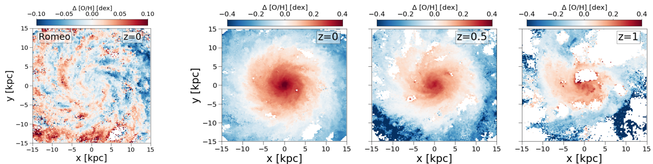
Figure 1. Face-on image of all gas within \pm 1 kpc of the galactic midplane of Romeo, one of FIRE-2 simulations that we analyze. We color-code gas by \Delta[\text{O}/\text{H}] , its deviation from the azimuthally averaged [\text{O}/\text{H}] . \Delta[\text{Fe}/\text{H}] (not shown) looks nearly identical to \Delta[\text{O}/\text{H}] , to within \lesssim 0.02 dex at all times. The left panel emphasizes azimuthal variations by showing the deviation from the azimuthally averaged [\text{O}/\text{H}] at each radius, that is, subtracting off the radial gradient, thus highlighting the enhanced enrichment correlated with spiral arms. The right 3 panels show the deviation from the mean [\text{O}/\text{H}] of all gas at R \leq 15 kpc at each redshift. White regions have highly diffuse gas in which we do not report a measured abundance. The radial gradient in [\text{O}/\text{H}] dominates over azimuthal variations at late times, but at early times the azimuthal variations are the most significant.
