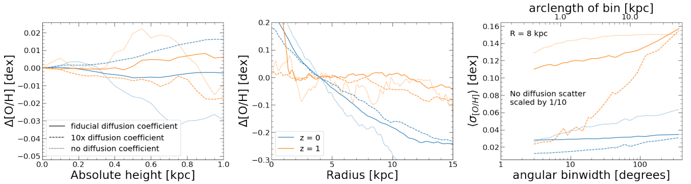
Figure C1. Vertical (left), radial (middle), and azimuthal variations (right) in [O/H] between our fiducial simulation of m12i, a version with no subgrid metal diffusion, and a re-simulation increasing the diffusion coefficient by 10 times. The vertical profiles show no clear systematic variations at a level important for our analysis. We normalize the radial profiles to 4 kpc (the approximate edge of the bulge) for clarity in comparison. The radial gradients (measured from 4 – 12 kpc for z = 0 , 2 – 8 kpc for z = 1 ) vary by no more than \approx 0.005 dex \text{kpc}^{-1} between our fiducial simulation and the simulation with 10 times higher metal diffusion, while the simulation with no metal diffusion has a \approx 0.13 dex \text{kpc}^{-1} steeper gradient at z = 0 . In the right panel, we scaled down the azimuthal scatter in the simulation with no metal diffusion by a factor of 10, for comparison. Thus, neglecting metal diffusion/mixing leads to 10 \times higher azimuthal scatter, and moreover, this scatter does not depend much on azimuthal scale. The enhanced metal diffusion re-simulation shows smaller azimuthal scatter at small azimuthal scales, given the enhanced mixing rate on these small scales. However, that simulation shows similar scatter at large azimuthal scales, indicating that disk-wide azimuthal scatter is not sensitive to the detailed choice of diffusion coefficient.
