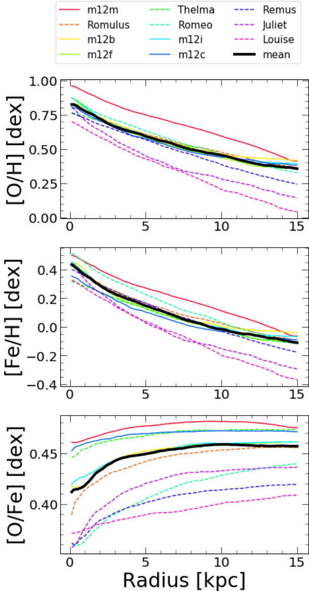
Figure 2. Radial profiles of gas-phase elemental abundances within the disks of our 11 galaxies at z = 0 , listed by decreasing stellar mass. Each simulation includes all gas, averaging across 3 snapshots ( \approx 50 Myr) within a disk height of \pm 1 kpc. The black line shows the mean across all hosts. The normalization of the radial abundances scales with the stellar mass of the galaxy (see Table: 1). For [\text{O}/\text{H}] and [\text{Fe}/\text{H}] , the profiles exhibit negative radial gradients, with a mean change across 0 - 15 kpc of \sim 0.51 dex for [\text{O}/\text{H}] and \sim 0.56 dex for [\text{Fe}/\text{H}] . The [\text{O}/\text{Fe}] profile is approximately flat at radii \gtrsim 4 kpc, indicating enrichment dominated by core-collapse supernovae, but it exhibits a small positive gradient in the inner galaxies, from the increasing importance of Fe from Ia supernovae.
