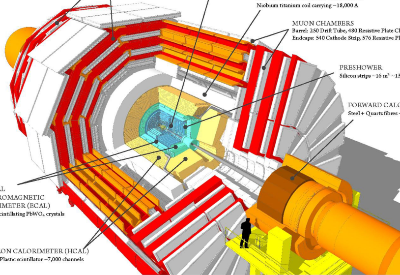
Extended Data Fig. 1 | The CMS detector at the CERN LHC. Schematic longitudinal cut-away view of the CMS detector, showing the different layers around the LHC beam axis, with the collision point in the centre.
