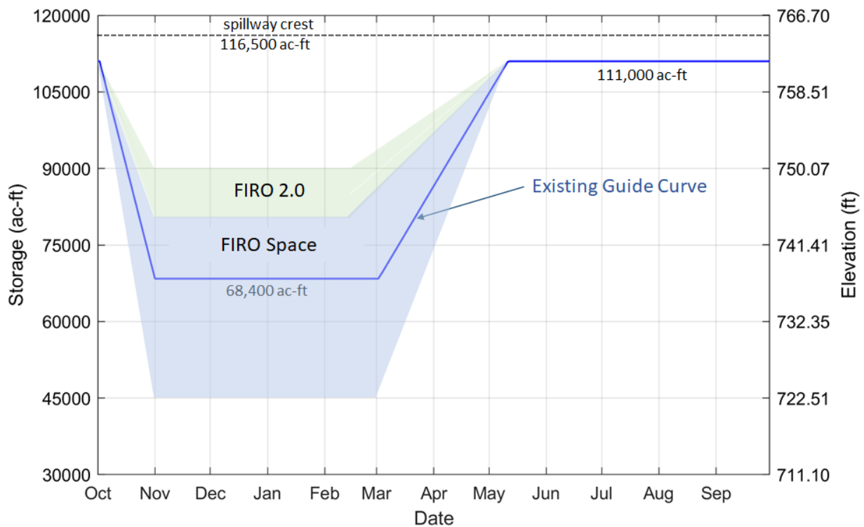
Figure 6.4. Conceptual FIRO Space for Lake Mendocino.
