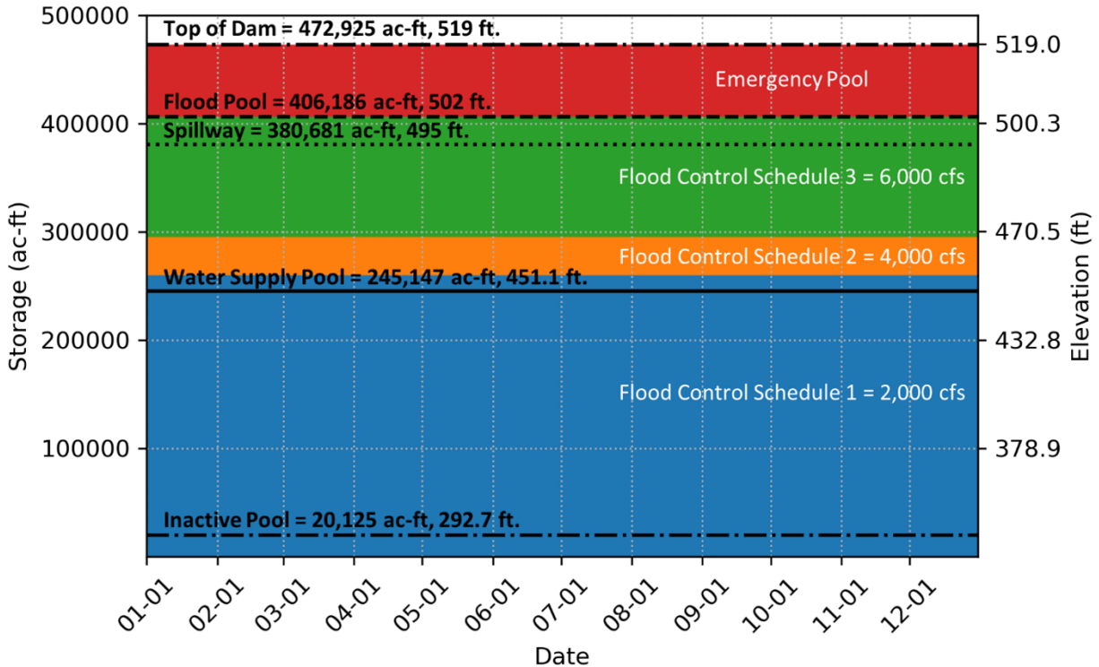
Figure 1.4. Lake Sonoma operations guide curve.
