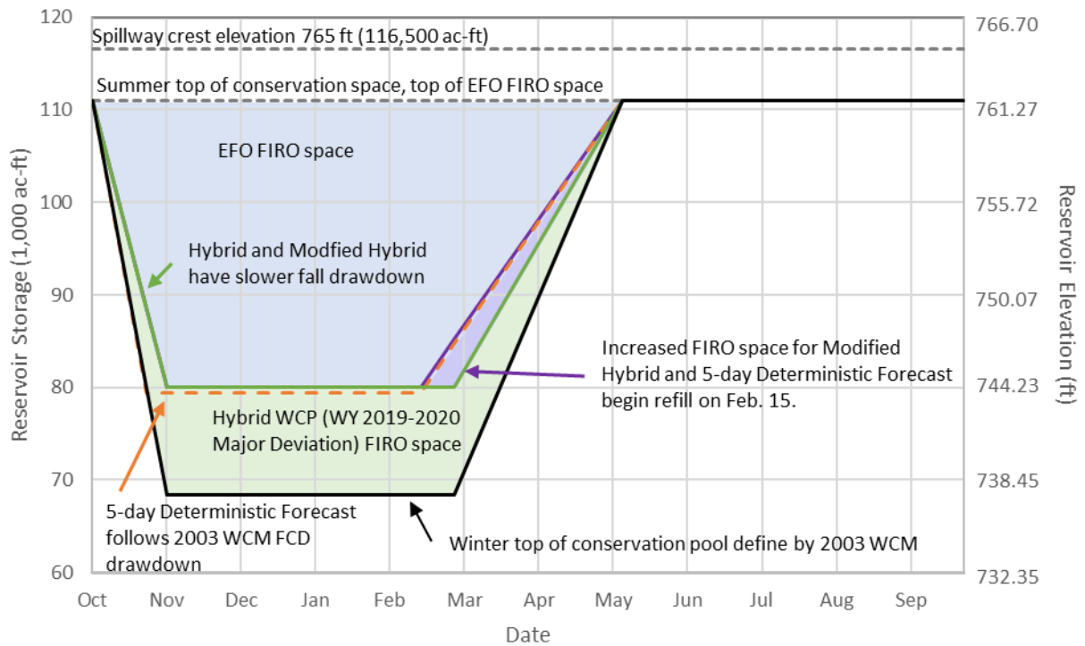
Figure 3.1. Lake Mendocino guide curves showing the baseline WCP (black line) and conditional storage spaces for the EFO (all shaded areas above black line), Hybrid (light green shaded area), and Modified Hybrid (light green plus light purple shaded areas) WCPs. The drawdown for the Five-Day Deterministic Forecast WCP is the same as the baseline WCP and roughly the same as the Modified Hybrid on the refill portion (dashed orange line).
