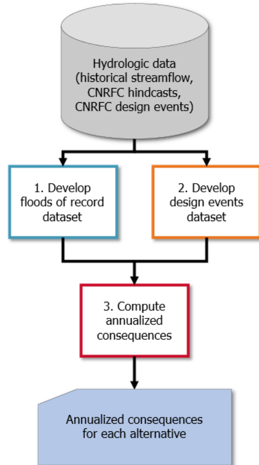
Figure 3.7. Overview of proposed consequence analysis methodology for Lake Mendocino FVA.
