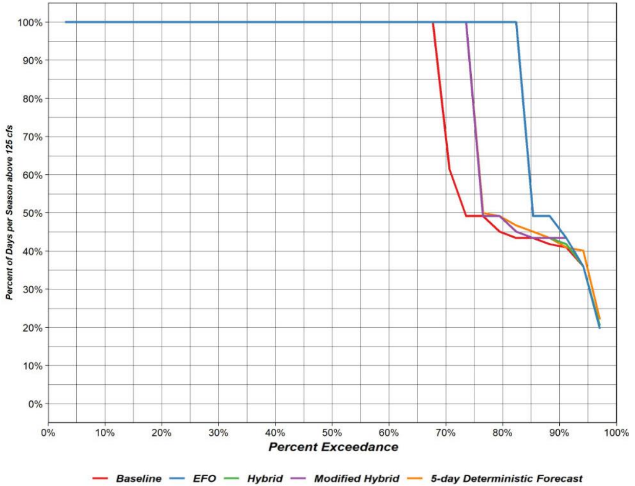
Figure 3.12. Percent of days per season, June through September, in which flows satisfy 125 cfs at Cloverdale. (Higher is better.) Hybrid, Modified Hybrid, and Five-Day Deterministic Forecast models are nearly identical through 76 percent exceedance.
