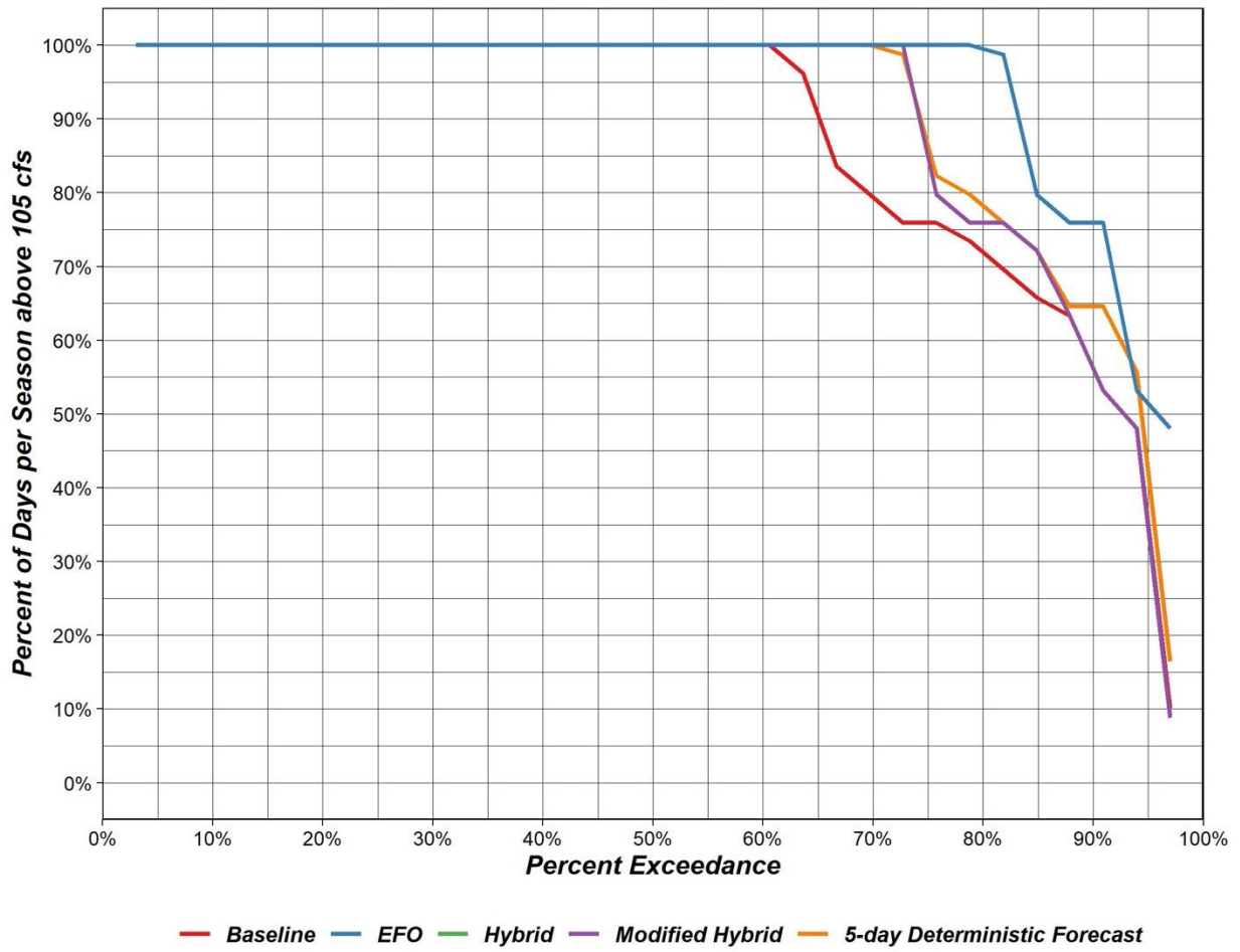
Figure 3.13. Percent of days per season, October 12 through January 1, in which flows satisfy 105 cfs at Healdsburg. (Higher is better.)
