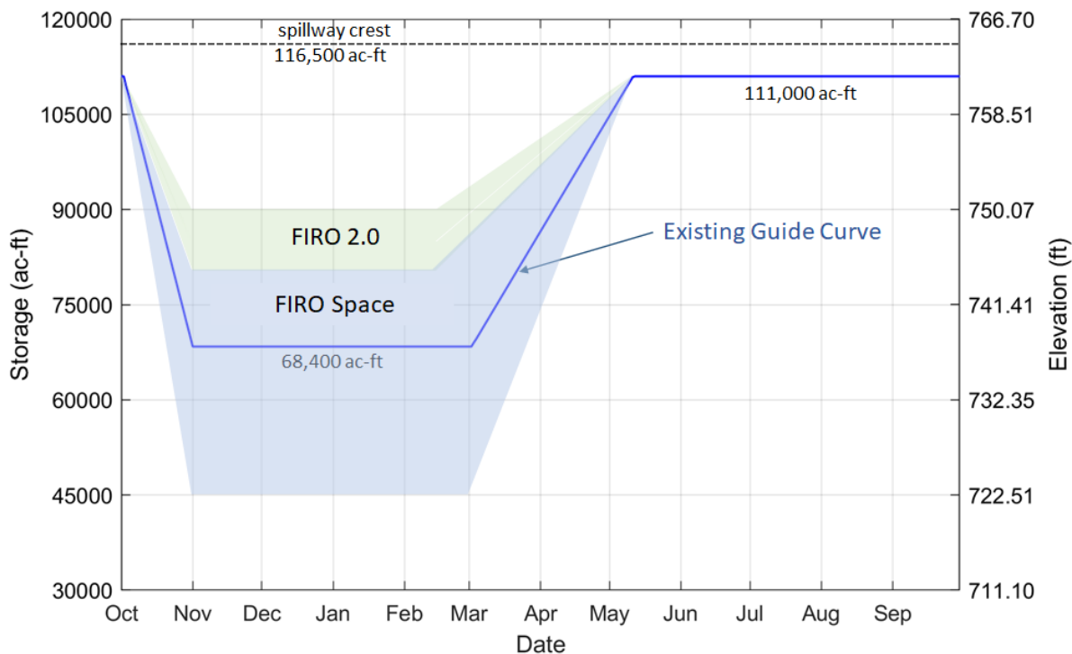
Figure E.4. Conceptual FIRO Space for Lake Mendocino.
