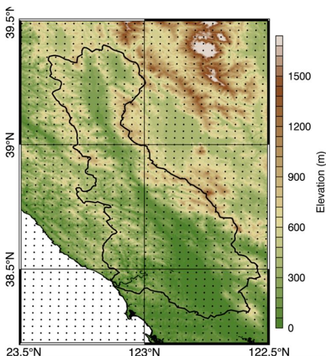
Figure 5.3. The Russian River watershed's topography (shading) with a 0.5° grid (solid lines) and 3km grid (dots) overlaid. The coarse resolution grid is unable to resolve regional characteristics of the watershed.
