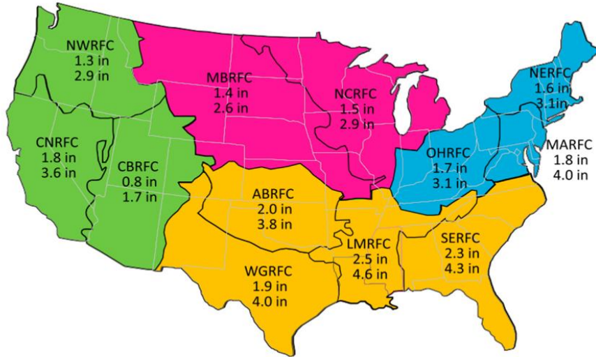
Figure 2.7. Map of NWS River Forecast Centers and regional thresholds for top 1 percent and 0.1 percent heaviest daily precipitation (from Sukovich et al. 2014).
