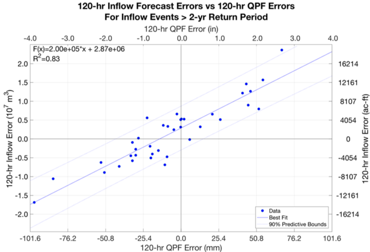
Figure 2.3. Relation of 120-hr forecasted inflow errors to their respective QPF errors for inflows with a return period greater than two years.
