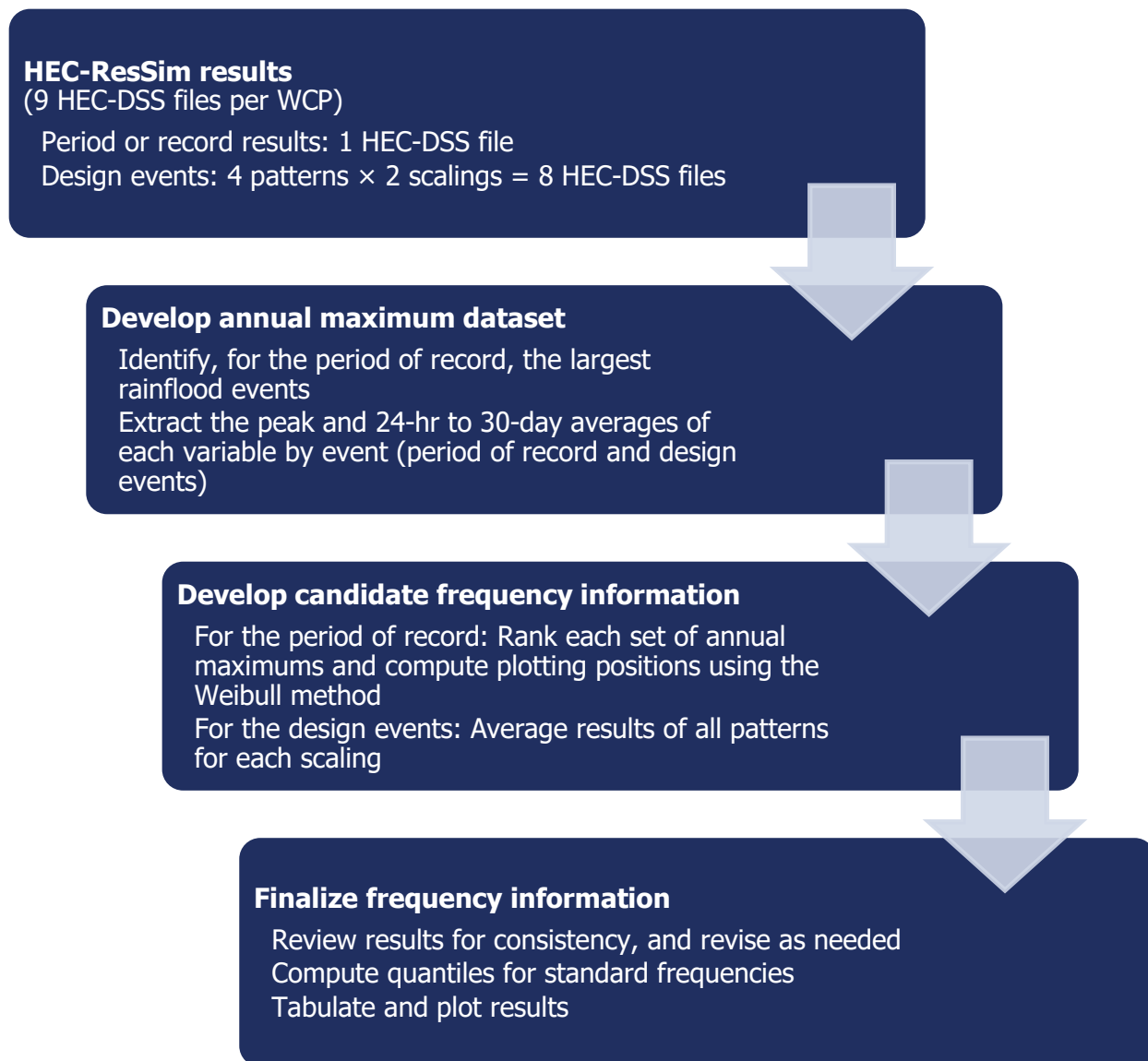
Figure 3.6. Procedure to calculate M1 through M7. Note that the procedure for calculating M10 through M16 is the same, with the exclusion of the design events.
