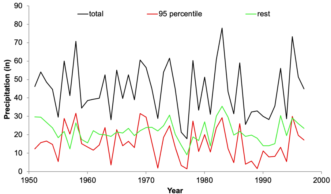
Figure 1.5. Annual precipitation variability and contribution of ARs for the Russian River above Hopland. From M. Dettinger, USGS.
