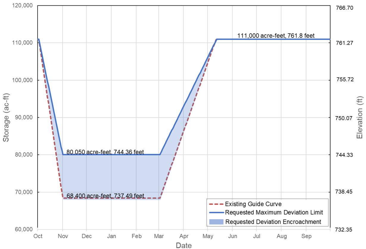
Figure 4.1. Changes to Lake Mendocino WCP proposed for the WY 2019 (and WY 2020) major deviation.
