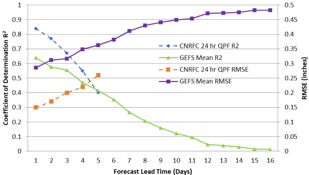
Figure 2.5. The 24-hr (daily total) QPF forecast skill metrics comparing CNRFC HAS with GEFSv10 ensemble mean.
