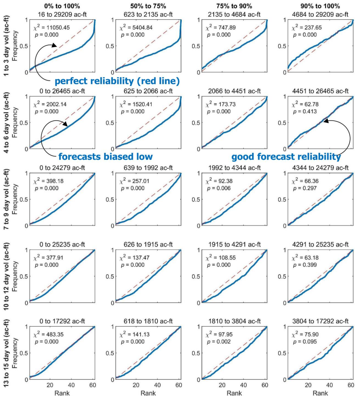
Figure 2.6. Cumulative rank histograms for three-day inflow forecasts to Lake Mendocino for five lead times and four stratified volume ranges.
