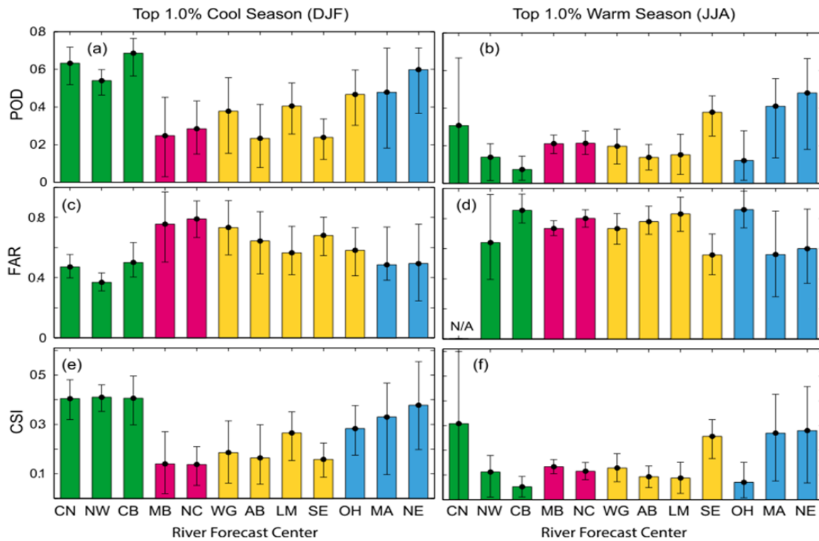
Figure 2.8. Variation of NCEP/WPC QPF verification metrics from 2007–2011 by River Forecast Center (from Sukovich et al. 2014).
