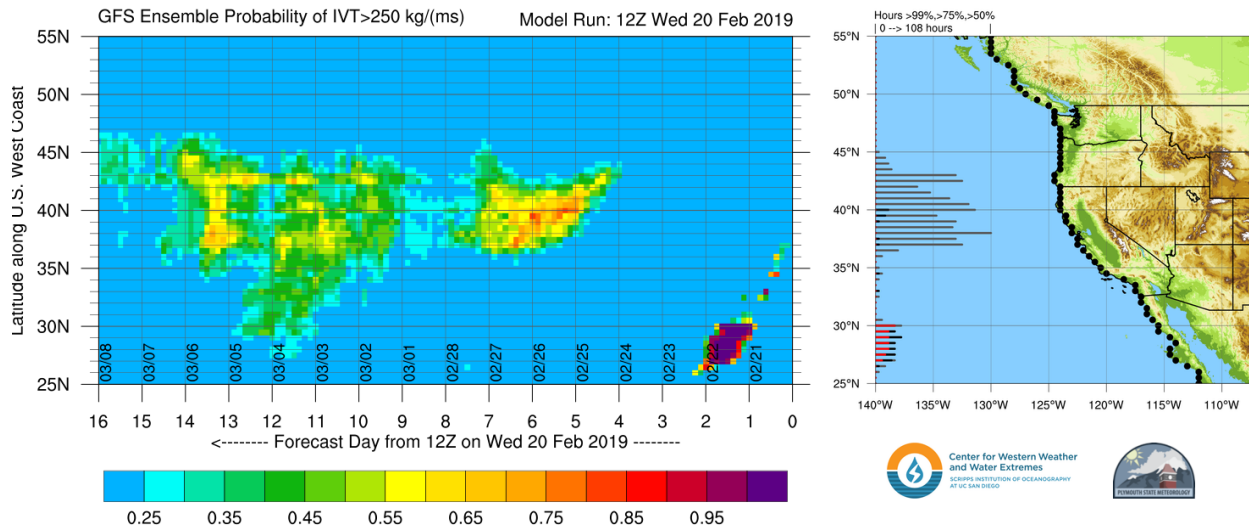
Figure 1.9. The AR Landfall Tool depicts the likelihood of an AR (shaded in colors) by latitude (y-axis) and forecast time (right to left on the x-axis) from February 20, 2019, providing forecast guidance 5 to 7 days in advance of the AR on February 25–27, 2019. The probability of AR conditions at a coastal point through time is displayed as the percentage of ensemble members with IVT > 250 (colorfill) (left). The duration of landfalling conditions according to ensemble probability thresholds of 99%, 75%, and 50% is plotted at half-degree latitude increments (right).
