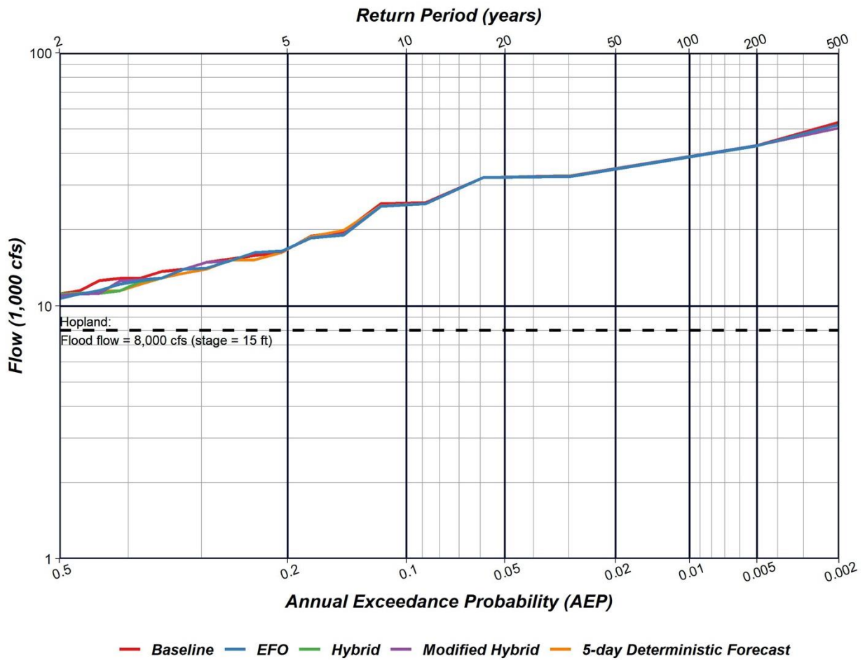
Figure 3.9. Annual maximum flow exceedance probability at Hopland.
