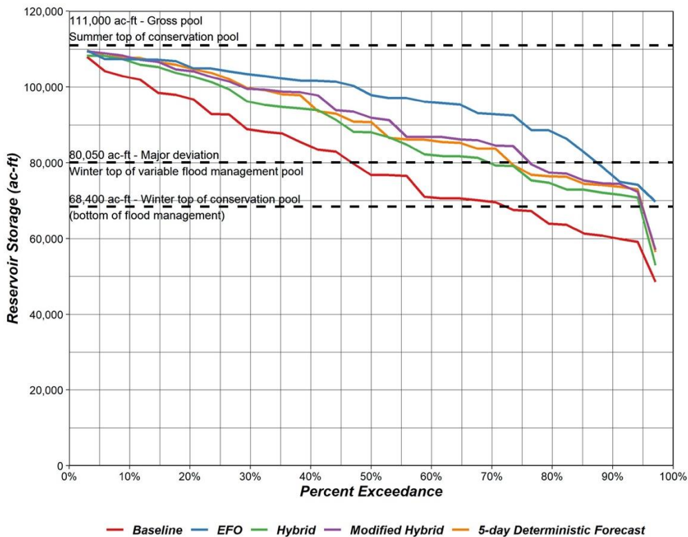
Figure 6.2. Improvements in water supply reliability as measured by metric 10, May 10 Lake Mendocino storage exceedance. Results from the evaluation are reported in Section 3.
