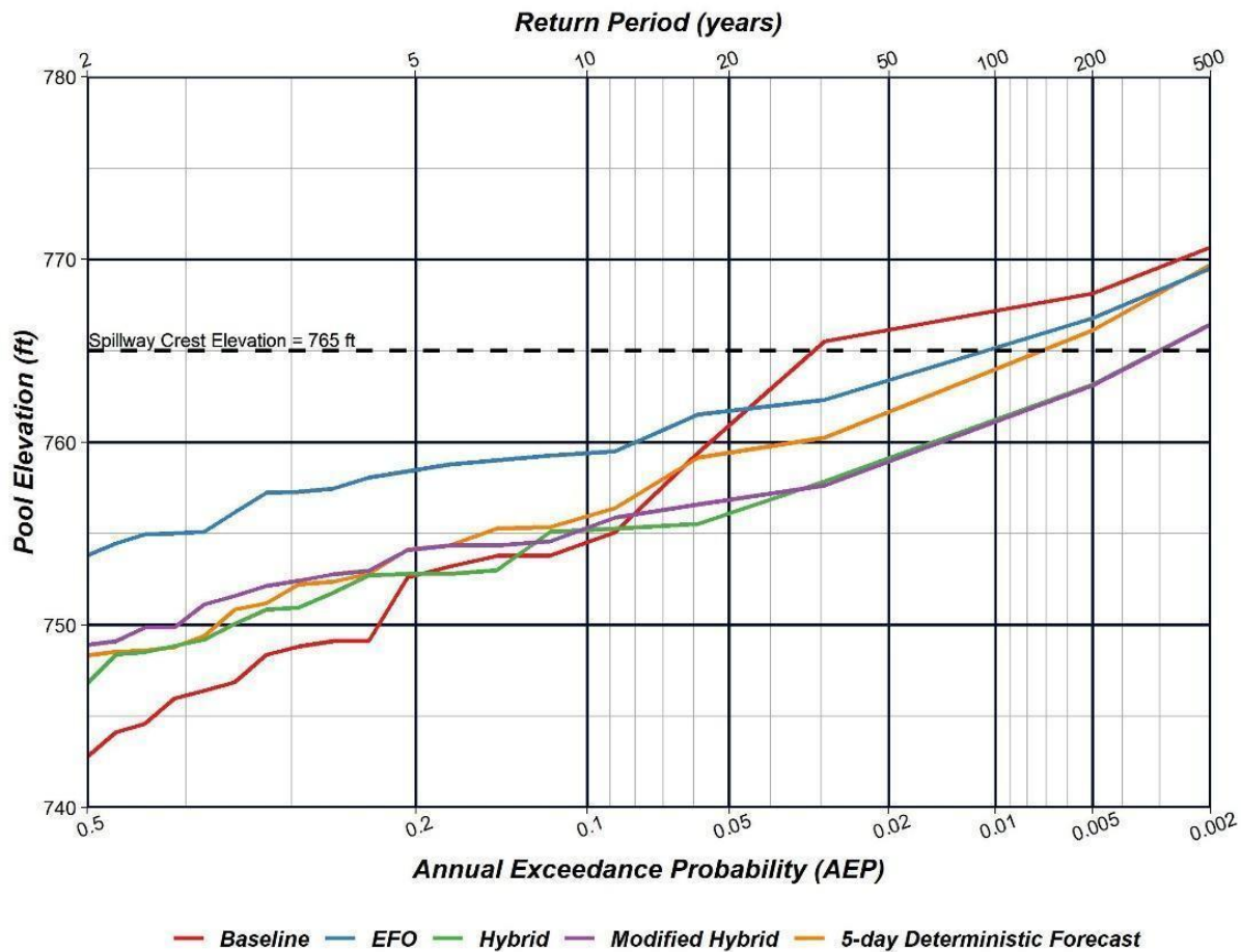
Figure 5.9. Annual maximum pool elevation frequency function for Lake Mendocino.
