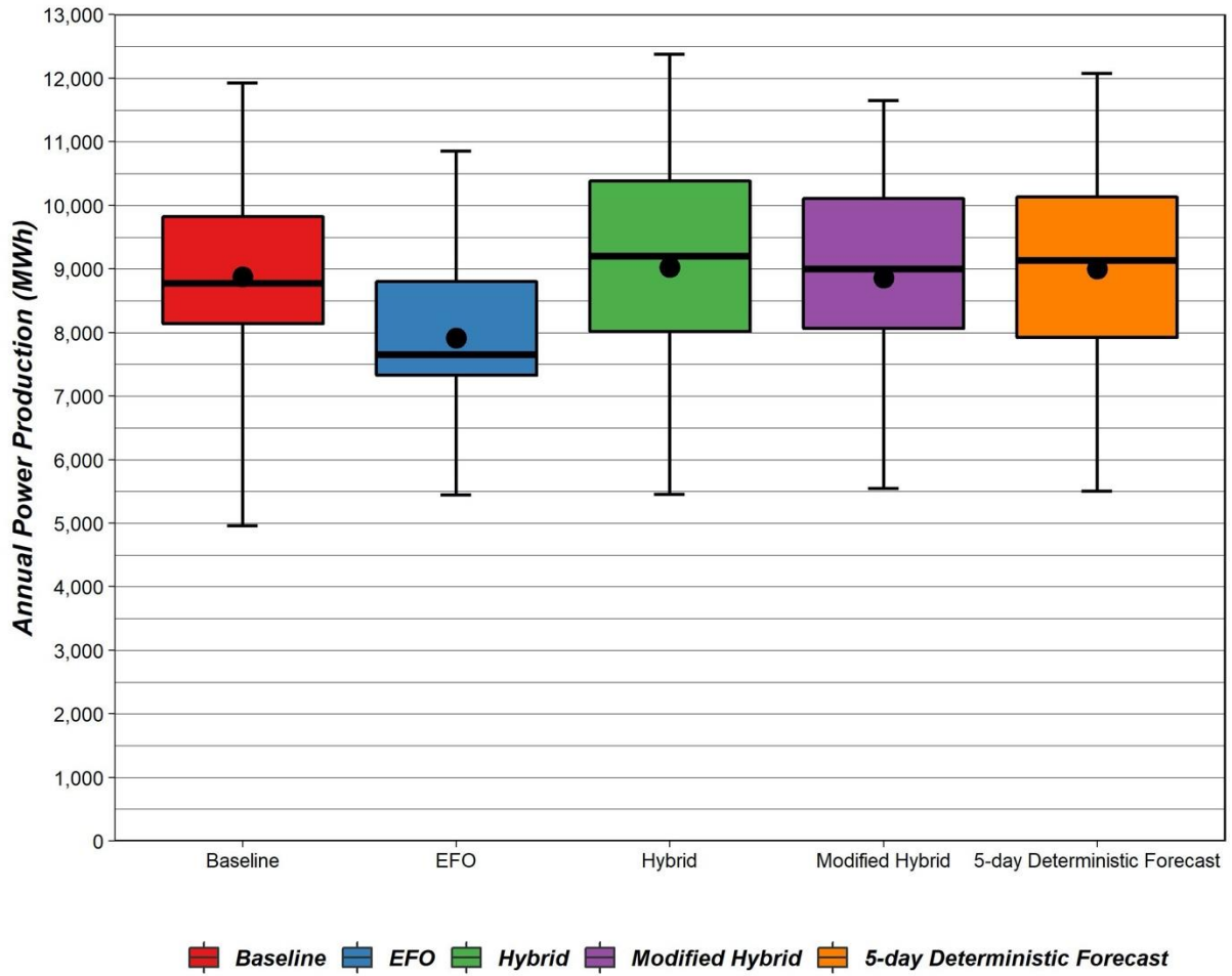
Figure 3.15. Annual (calendar year) power production for Lake Mendocino. (Higher is better.)
