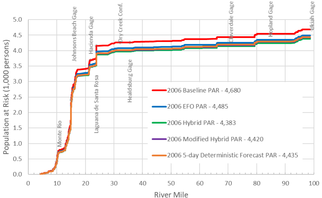
Figure 3.10. Damage and population at risk (PAR) values along the Russian River for each WCP alternative for the historical 2006 event.
