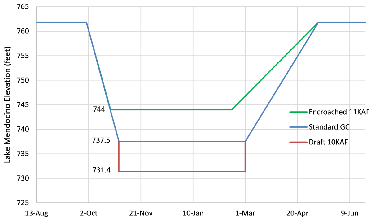
Figure 3.5. Lake Mendocino guide curves for the Five-Day Deterministic Forecast WCP. The blue line is the baseline WCP guide curve. The green line allows for up to 11,000 ac-ft of conditional encroachment and the red line provides up to a 10,000 ac-ft draft into the conservation space to allow for major events.
