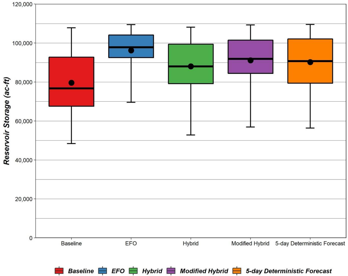
Figure 3.11. Lake Mendocino storage on May 10.
