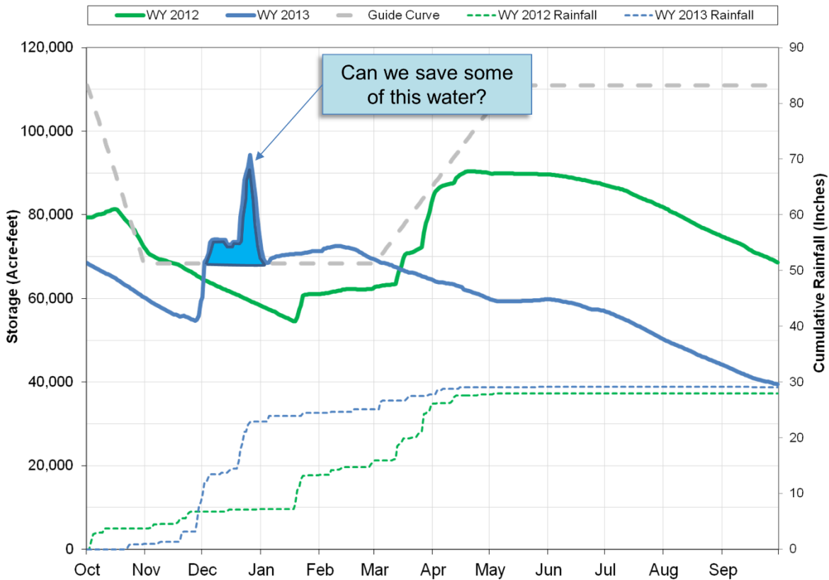
Figure 1.7. Storage (solid lines) and cumulative precipitation (dashed lines) for WYs 2012 (green) and 2013 (blue).
