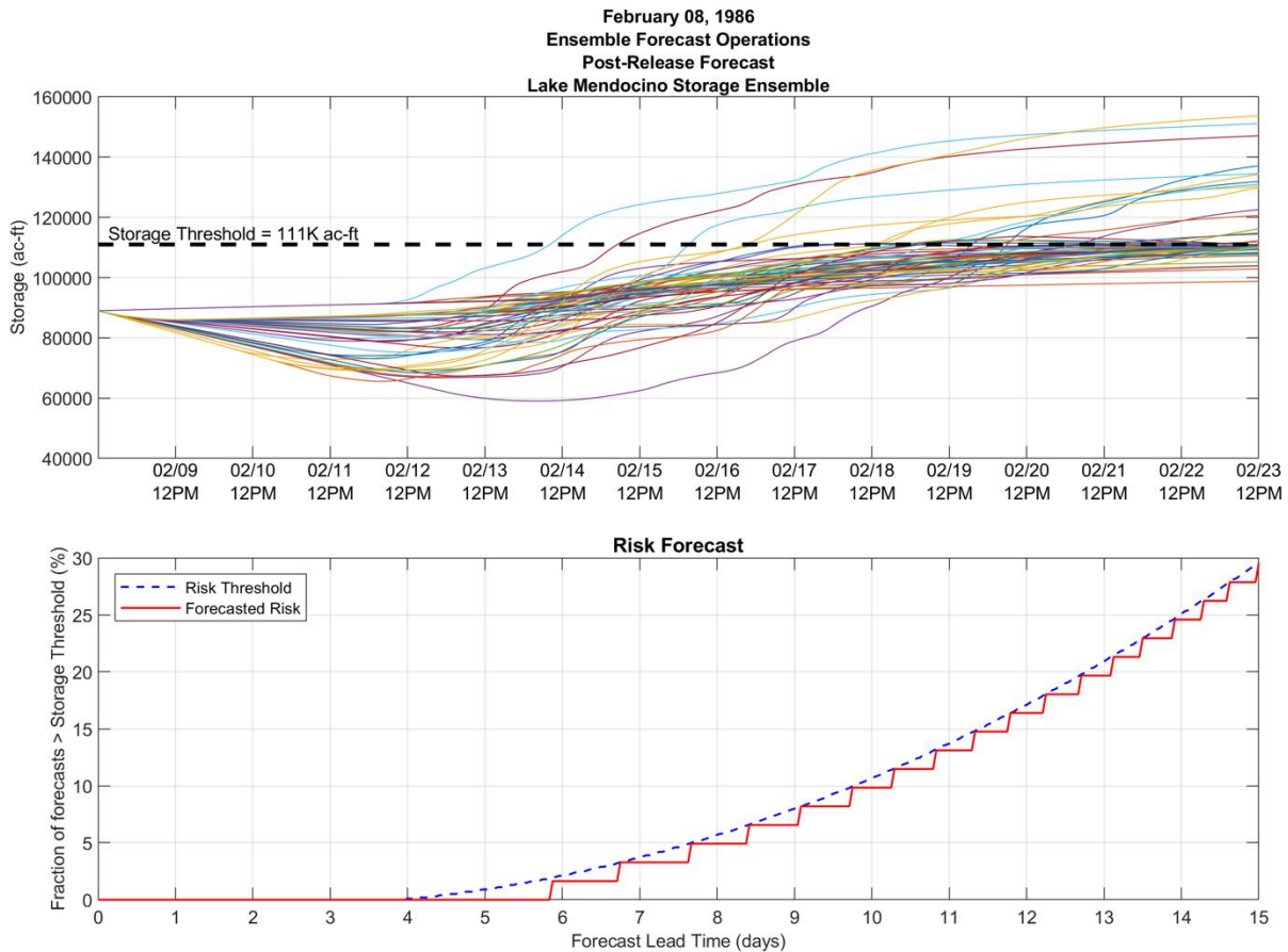
Figure 3.4. Forecast ensemble storage (top plot), risk curve (blue dashed line, bottom plot), and frequency of storage threshold exceedance (red line, bottom plot) with time after recommended release is identified and processed into storage ensemble members.
