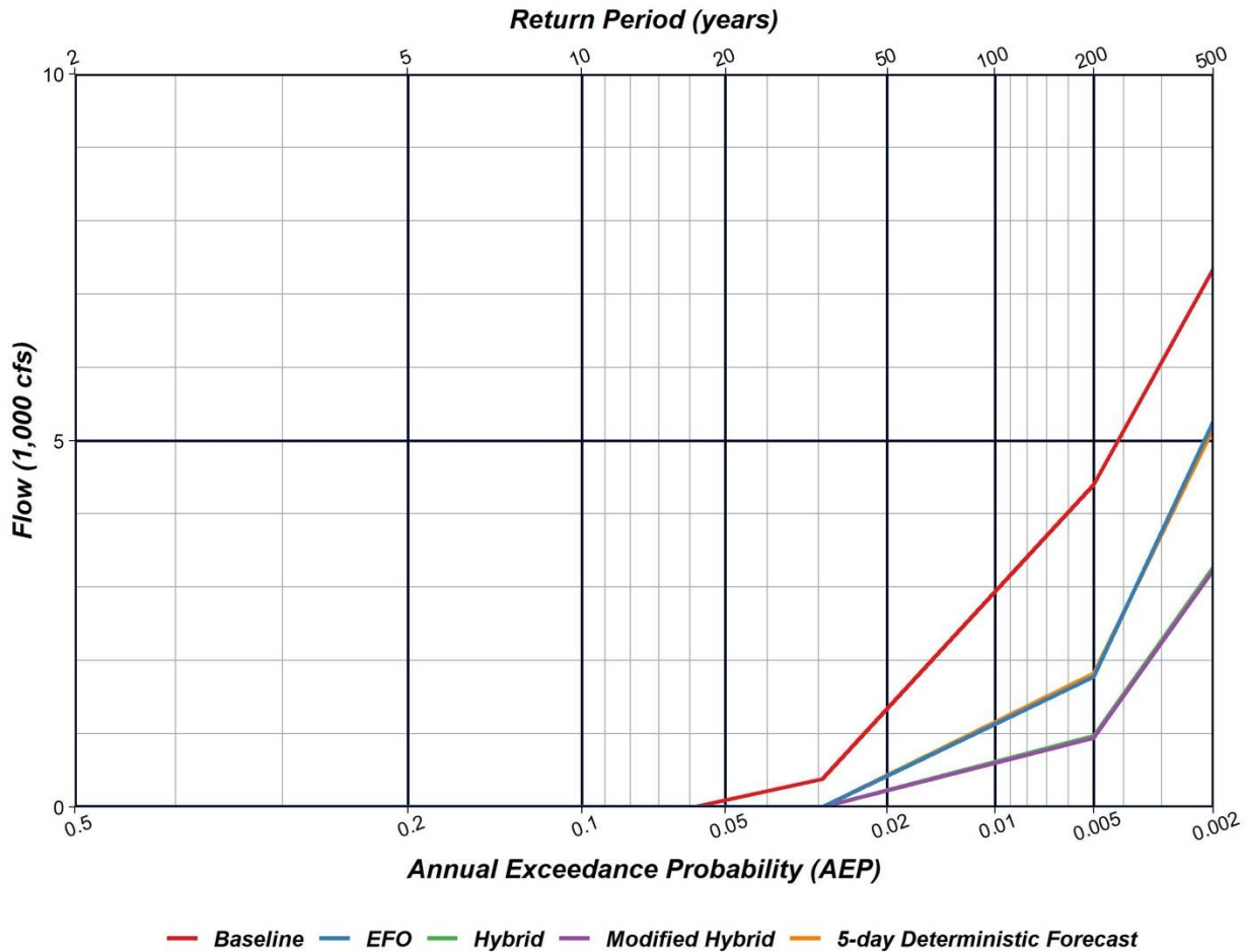
Figure 3.8. Annual maximum uncontrolled spill-frequency in Lake Mendocino. The Hybrid and Modified Hybrid results are nearly identical (lower lines) and the Five-Day Deterministic Forecast and EFO results are also nearly identical (middle lines).
