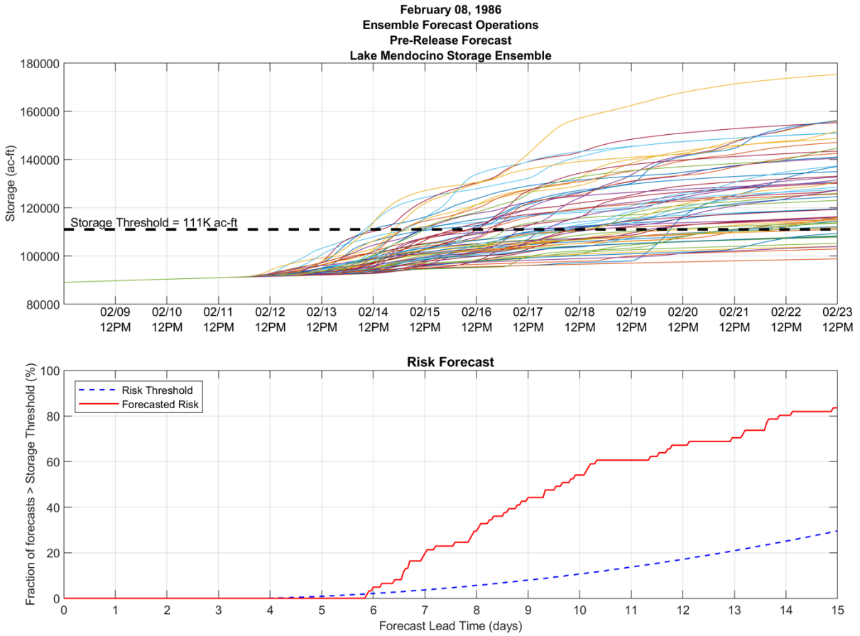
Figure 3.3. Forecast ensemble storage (top plot), risk curve (blue dashed line, bottom plot) and frequency of storage threshold exceedance (red line, bottom plot) with time before recommended release is identified and processed into storage ensemble members.
