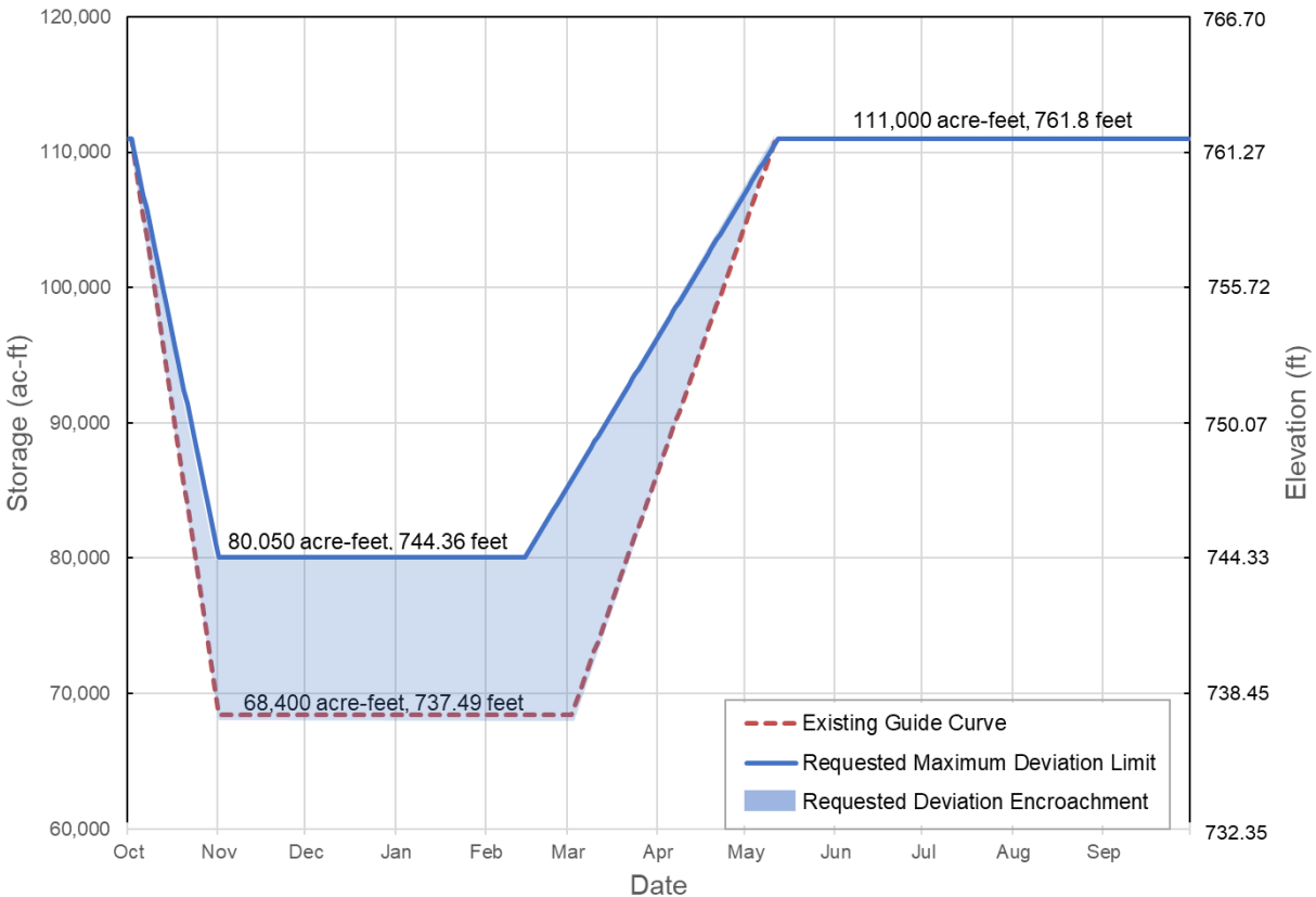
Figure 6.1. The existing guide curve (red dashed line) and the proposed maximum deviation limit of the flood space encroachment.
