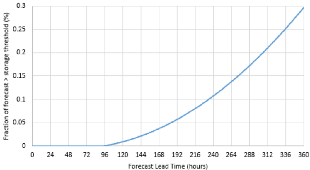
Figure 3.2. Sample risk curve for EFO-type WCPs. The blue line describes the maximum percentage of ensemble storage members that can exceed the 111,000 ac-ft threshold with time in hours.
