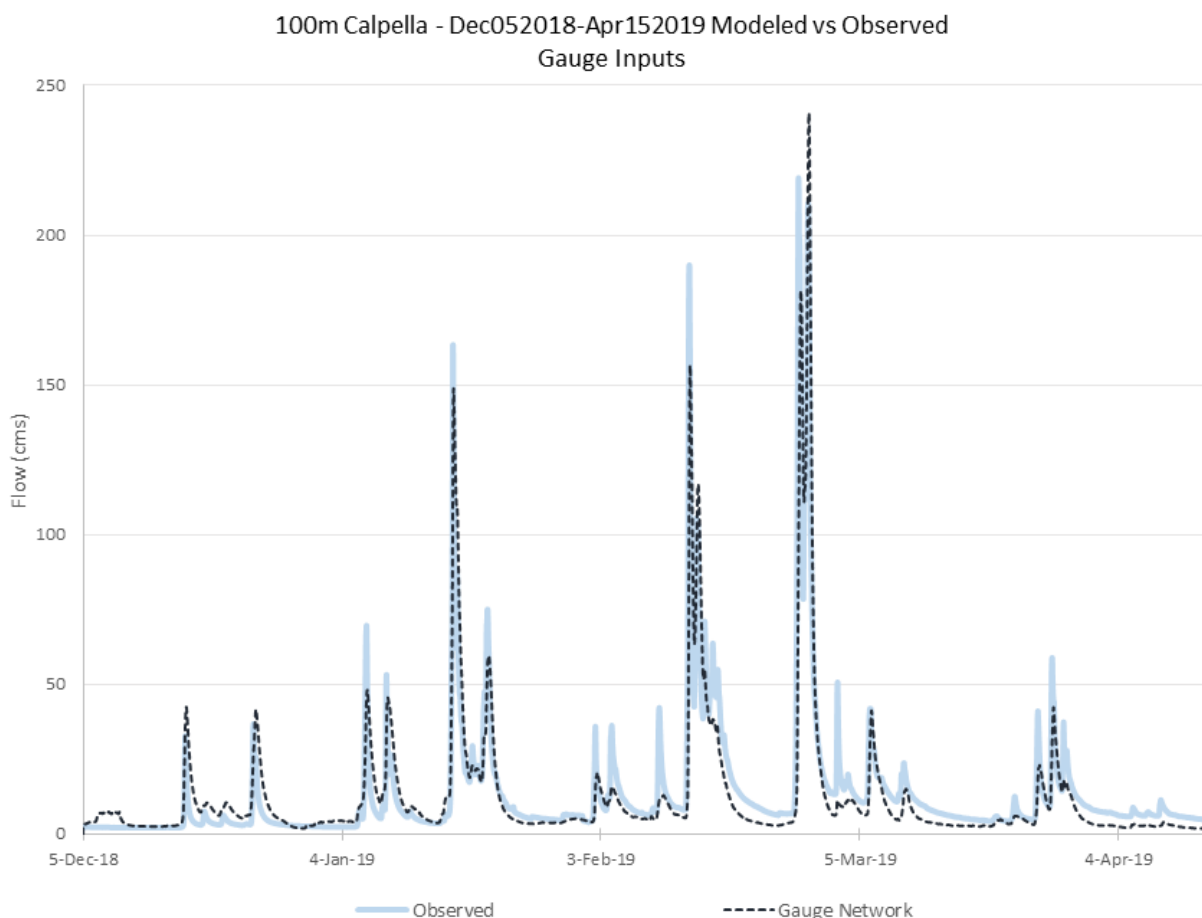
Figure 5.7. Comparison of GSSHA model simulated (black dashed line) and observed (blue solid line) flow using observed precipitation.
