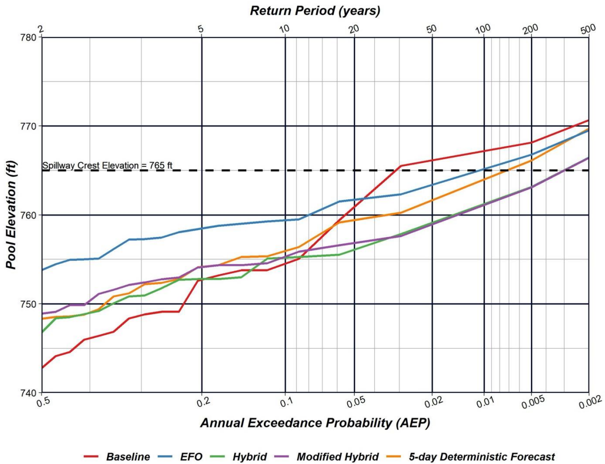
Figure 6.3. Frequency of annual maximum pool elevation for Lake Mendocino. Results from the evaluation are reported in Section 3.
