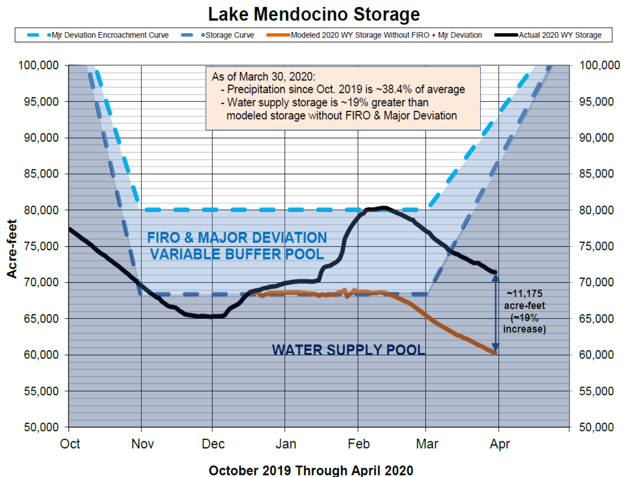
Figure E.2. Lake Mendocino storage increased by 19 percent (more than 11,000 acre-feet) during major deviation operations in WY 2020.
