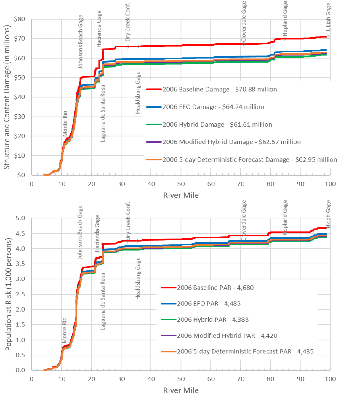
Figure 5.8. Damage and population-at-risk values along the Russian River for the baseline (red) and each FIRO WCP alternative for the historical January 2006 flood event.
