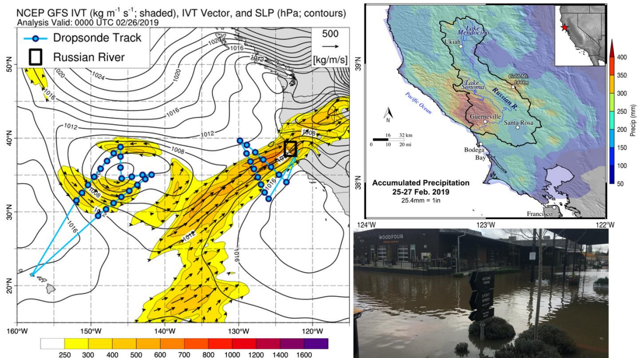
Figure 1.8. AR impacting the Russian River basin in February 2019. The left panel shows integrated water vapor transport (IVT), a measure of the AR's strength, along with the aircraft flight tracks. The top-right panel shows the 48-hr rainfall totals observed between Sunday, February 25, at 4 a.m. and Tuesday, February 27, at 4 a.m., reported by the California-Nevada River Forecast Center (CNRFC). The bottom-right panel is a photograph of flooding in the town of Sebastopol on February 27 (courtesy Nina Oakley).
