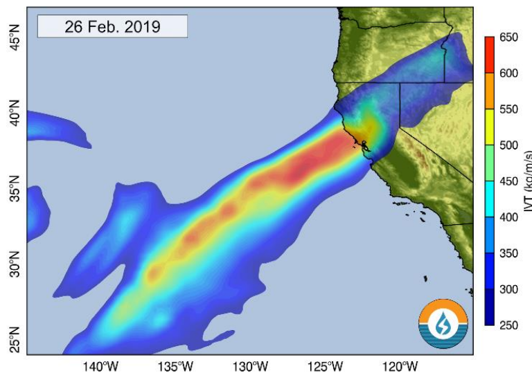
Figure E.1. An AR making landfall in the Russian River area on February 26, 2019. Shading represents integrated water vapor transport (IVT), which indicates the strength of the AR.
