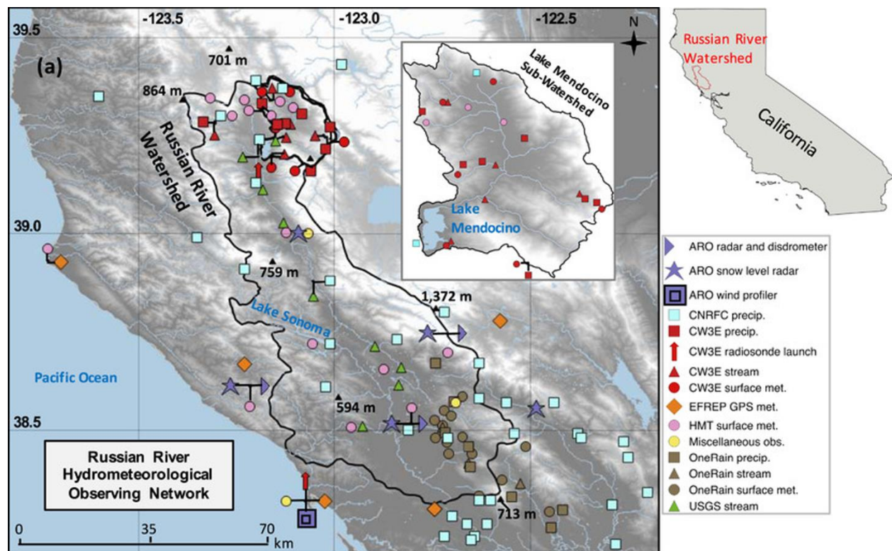
Figure 5.6. RHONET in and around the Russian River watershed (from Figure 1, Sumargo et al. 2020b).
