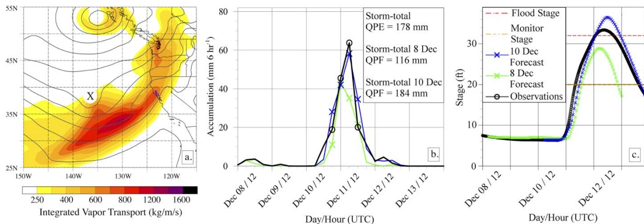
Figure 5.2. Reanalysis of the AR conditions at 0000 UTC on December 11, 2014. The left panel shows integrated water vapor transport (IVT) ( \text{kg m}^{-1} \text{s}^{-1} ) and sea-level pressure (hPa; contours every 4 hPa from 974 to 1018 hPa). The “X” marks the location of a mesoscale frontal wave that modified AR conditions over the Russian River Watershed. The center panel shows the six-hourly accumulated RRW-mean areal QPF issued by CNRFC at 1200 UTC on December 8 (mm; green) and 1200 UTC on December 10 (mm; blue) and the CNRFC Quantitative Precipitation Estimate (QPE) (mm; black). Time on the x-axis refers to QPE valid time. The right panel shows the Guerneville river-stage forecast issued by CNRFC near 1200 UTC on December 8 (mm; green) and near 1200 UTC on December 12 (mm; blue), as well as observations from the river gauge (mm; black).
