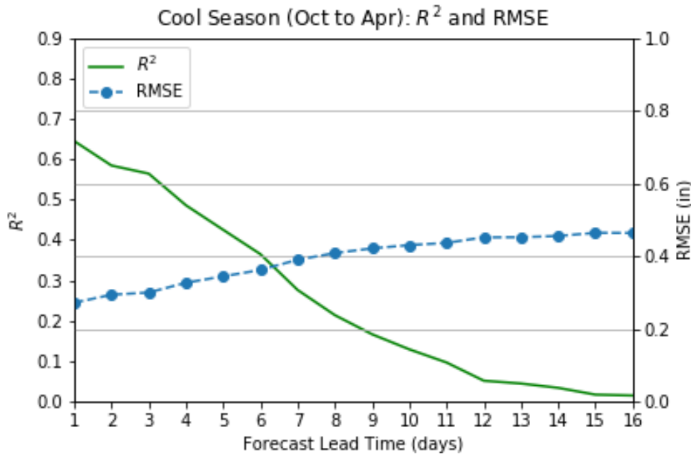
Figure 2.4. 1985–2010 GEFSv10 six-hour ensemble mean precipitation R^2 and RMSE in inches for the Lake Mendocino watershed.
