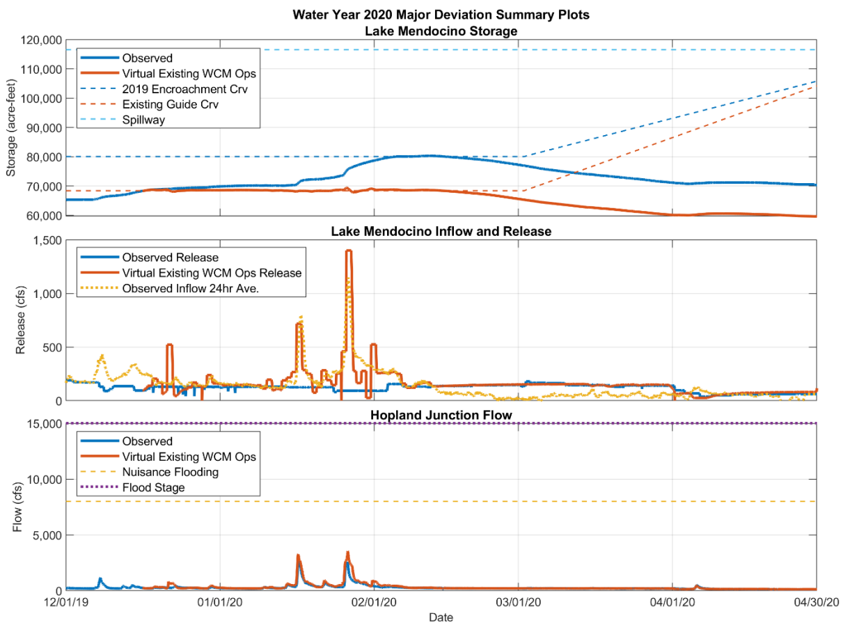
Figure 4.3. Reservoir storage for Lake Mendocino during major deviation operations of WY 2020.
