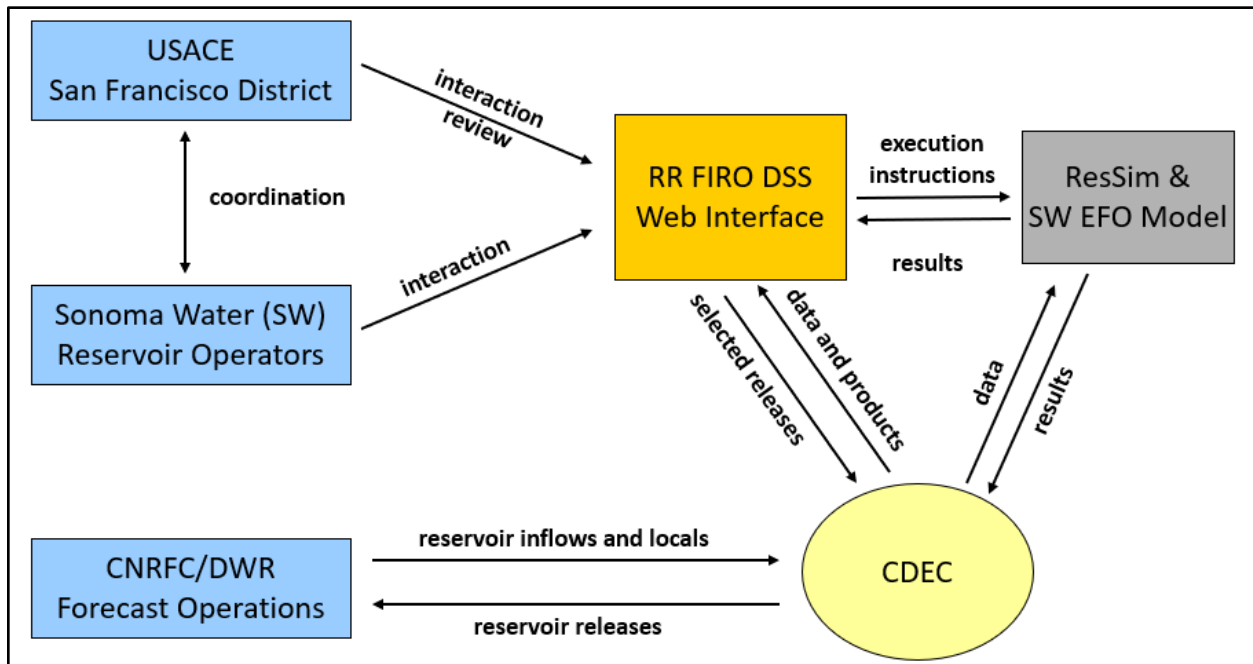
Figure 4.4. Data and information flow for the CDEC FIRO interface.
