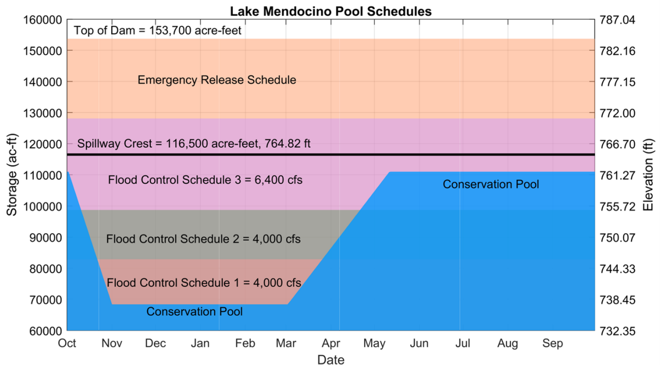
Figure 1.3. Lake Mendocino operations guide curve.
