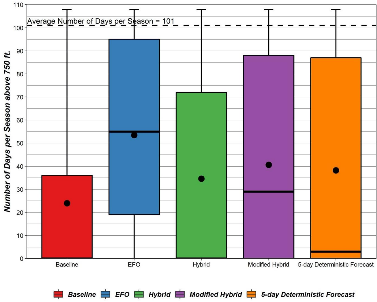
Figure 3.14. Number of days per recreation season during which access to Bushay Campground is limited (pool elevation 750.0 feet is exceeded). (Lower is better.)
