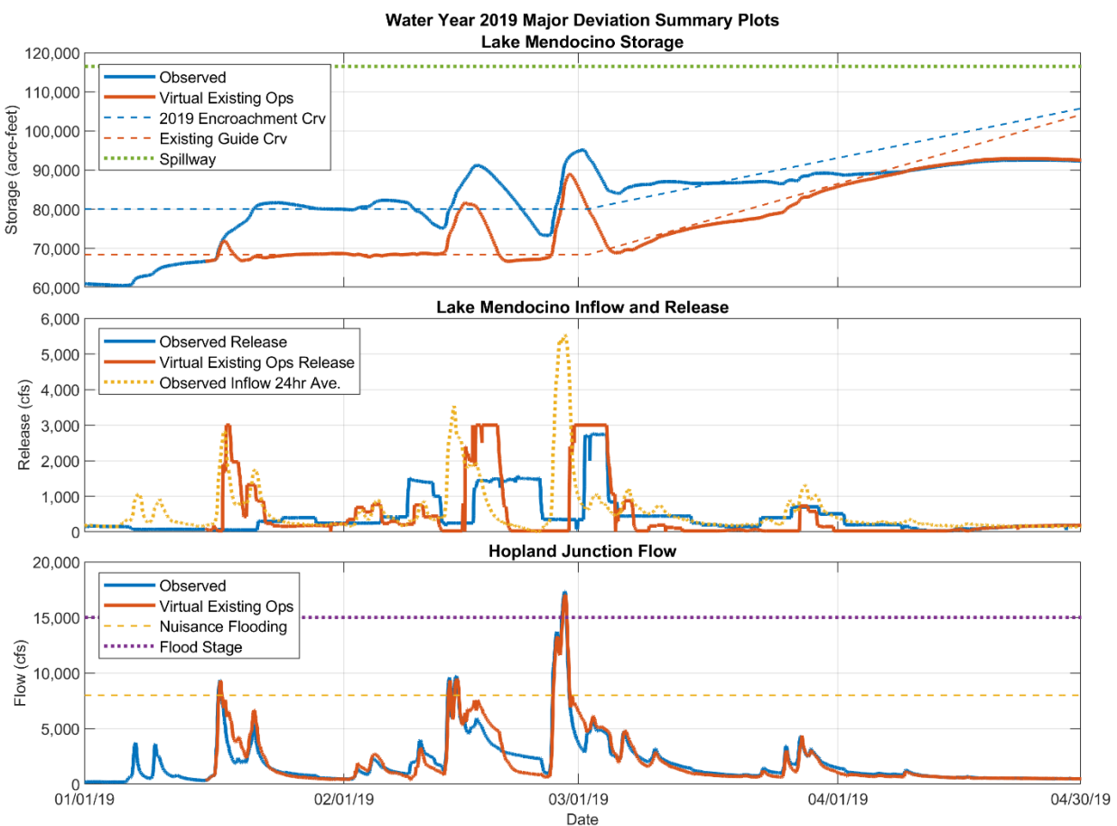
Figure 4.2. Reservoir storage for Lake Mendocino during major deviation operations of WY 2019.
