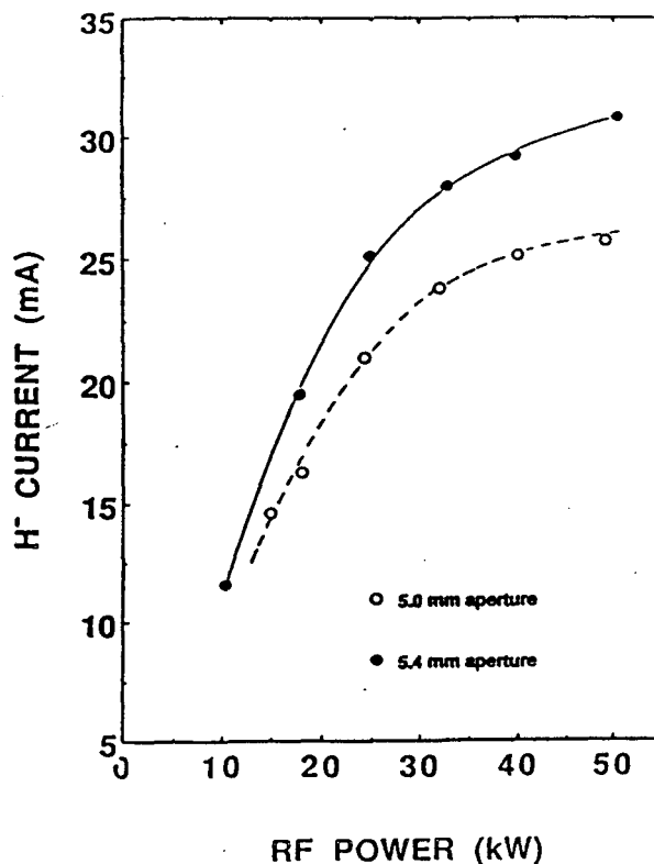
Fig. 5 H^- current versus rf input power for two different extraction aperture sizes.
