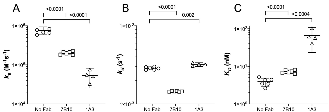
Fig 2. Kinetic parameters of Fab-mediated binding of FH to FHbp determined by surface plasmon resonance. (A) Association rate constant, k_a . (B) dissociation rate constant, k_d . (C) apparent dissociation constant, K_D . For all three panels, the means and 2 SE of four to six replicates are shown. The p -values for two-tailed t -tests comparing the parameters of FH binding in the presence versus the absence of Fab were calculated with Prism 8.3 (GraphPad).
