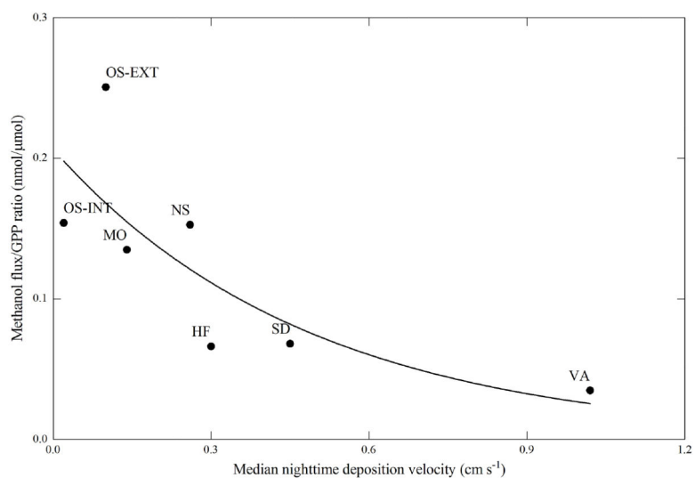
Figure 6. Methanol flux to GPP ratio as a function of the median nighttime deposition velocity. The solid line represents an exponential fit ( r^2 = 0.77 ).
