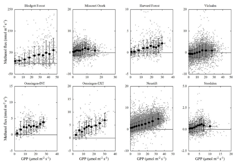
Figure 5. Relationship between gross photosynthesis (GPP) and methanol flux. Small grey symbols represent half-hourly flux measurements, black closed symbols 10 bin averages with equal numbers of data. Error bars refer to one SD. Note different x and y scales in different panels.
