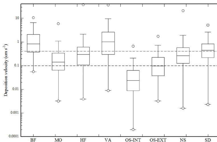
Figure 4. Box-plots of nighttime methanol deposition velocities at the eight study sites. Horizontal dashed lines indicate the range of deposition velocities ( 0.1\text{--}0.4\text{ cm s}^{-1} ) used in global budgets (see also Table 2). Box plots show minima/maxima (circles), 5 and 95 % quartiles (whiskers), the interquartile range (box) and the median (horizontal line).
