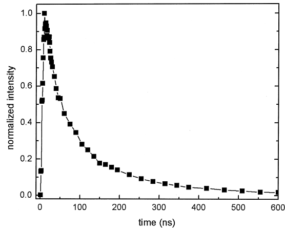
Fig. 4. Temporal evolution of the brightness taken from the images with time elapsed after the onset of spark. The spark emission peaked around 11 ns after the onset of plasma formation.
