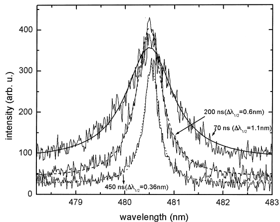
Fig. 7. Stark-broadened profile of Ar^+ transition at 480.6 nm at different times after the onset of spark. The FWHM of this line is used to infer electron density. The smooth curves represent the fitted Lorentzian curves. The measured Stark widths are also given.
