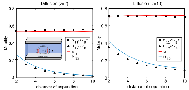
Figure 9: Diffusivity of Ellipsoidal Particles near a Wall. For two interacting ellipsoidal particles, the correlated diffusivity tensor components are compared to the hydrodynamic mobility components. Good agreement is found both for particles near the channel center z = 10\text{nm} and near the wall z = 2\text{nm} . For more details see [8].
