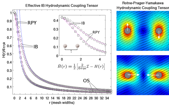
Figure 7: Hydrodynamic interactions. (IB) immersed boundary coupling for the parallel and perpendicular components of the pair-mobility tensor (data points), (RPY) Rotne-Prager-Yamakowa tensor [45], (OS) Oseen tensor [2].
