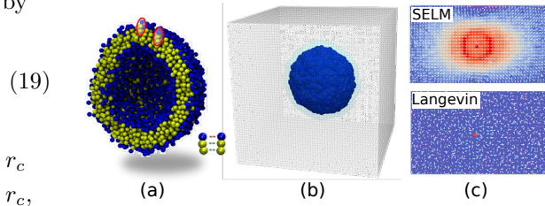
Figure 12: Vesicle Lipid Bilayer Membrane Model. (a) self-assembled vesicle and three bead lipid model, (b) mesh of the SELM fluctuating hydrodynamics coupling the vesicle lipids, (c) lipid pair correlations.
