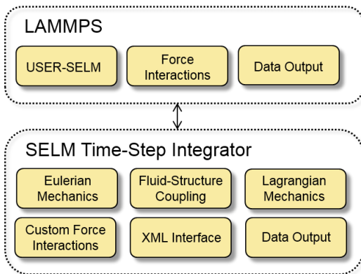
Figure 5: The package USER-SELM and the SELM time-step integrator classes coordinate the simulation. Shown are the broad categories of C++ classes and the interactions between SELM and LAMMPS .
