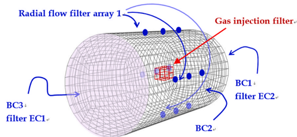
Fig. 34. NCU/TPC-V model. Locations where boundary conditions for experiment 2 are prescribed.
