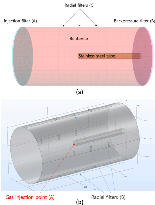
Fig. 32. KAERI-D model. Boundaries where boundary conditions are prescribed for (a) experiment 1 and (b) experiment 2.
