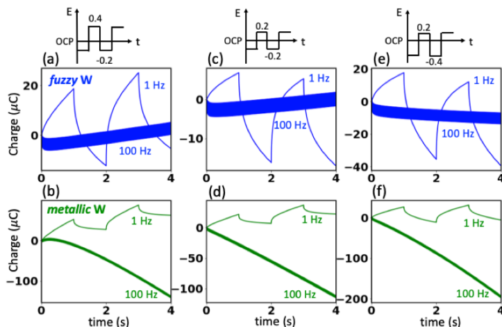
Figure 4.7: Charging characteristics of fuzzy W (a), (c) and (e) and metallic W (b), (d) and (f) based electrodes probed through chronocoulometry (CC) at a pH of 7. Here, the voltage was modulated between V_1 and V_2 , where V_1 ( V_2 ) is a voltage positive (/negative) to the PZC potential. The voltage-time profiles are inset. For illustration, the response at low frequency (1 Hz) and high frequency (100 Hz) are indicated.
