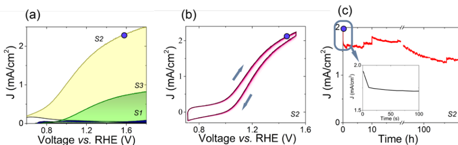
Figure 3.4: Photocurrent, in linear sweep voltammetry (LSV) of samples S1, S2 and S3 in 0.1M K_2SO_4 , the blue dot indicates the current density @ 1.56 V_{RHE} . (b) Cyclic voltammetry (CV) based characterization of sample S2 over ten cycles indicates behavior characteristic of nano-/micro-scale electrodes, due to hierarchical electrode sub-structure as well as charge storage proportional to the area enclosed between the forward and reverse voltage scans, (c) OER related photocurrent stability test (@1.56 V vs. RHE) of S2 for the first twenty hours and subsequently extended another ninety hours. The inset indicates an expected current decay over the first few seconds due to Cottrell diffusion limitations.
