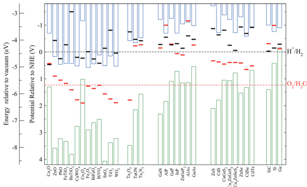
Figure 2.2: Calculated oxidation potential (red bars) and reduction potential (black bars) relative to the NHE and vacuum level for a series of semiconductors in solution at pH = 0[21]
