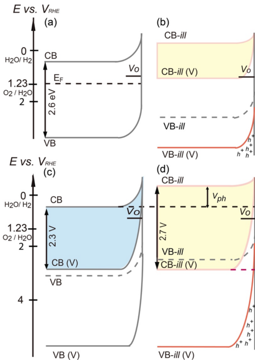
Figure 3.7: (a) Schematic band structure (CB: conduction band and VB: valence band) diagram of WO_{3-x} interfaced with a K_2SO_4 electrolyte, and voltage/energy levels considered with respect to the reversible hydrogen electrode (RHE). The bandgap of 2.6 eV along with the oxygen vacancies ( V_o ) are indicated. (b) Under illumination, the photo-generated charges reduce the band bending, implying an upward band shift (i.e., CB-ill and VB-ill) compared to (a). Under application of a positive bias voltage (V), the CB and VB move downwards (i.e., CB-ill (V) and VB-ill (V)), with respect to the original band positions indicated in (a), (c) The band positions at the voltage of 2.3 V corresponding to the R_{ct} peak of Figure 4(b), (d) The band positions at the voltage of 2.7 V corresponding to the R_{ct} peak of Figure 4(d). A critical oxygen vacancy and h^+ concentration at the surface, as in S2, has been found to be necessary for enhanced photoelectrochemical current density. The V_{ph} refers to the photovoltage.
