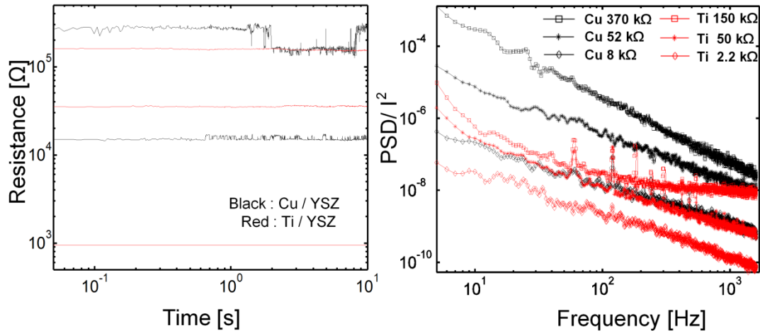
Figure. 3.22. (a) Resistance sampling for both Cu/YSZ and Ti/YSZ devices at different resistance states. (b) Normalized noise power spectrum density for both types of devices at different resistance states.
