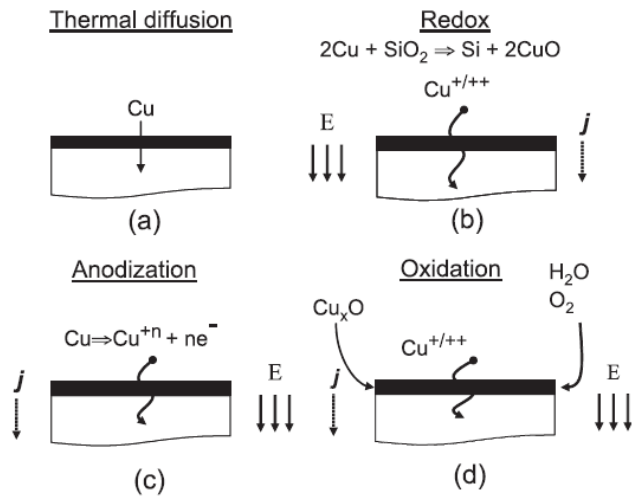
Figure 2.4. Four possible ways of copper injection into SiO 2 [11]
