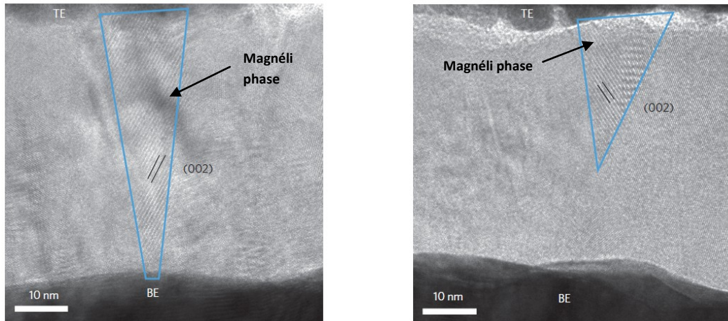
Figure 1.26. TEM image of Magnéli phase after the forming process inside of Pt/TiO 2 /Pt cell (Left) and a discontinued Magnéli phase (Right) [44]
