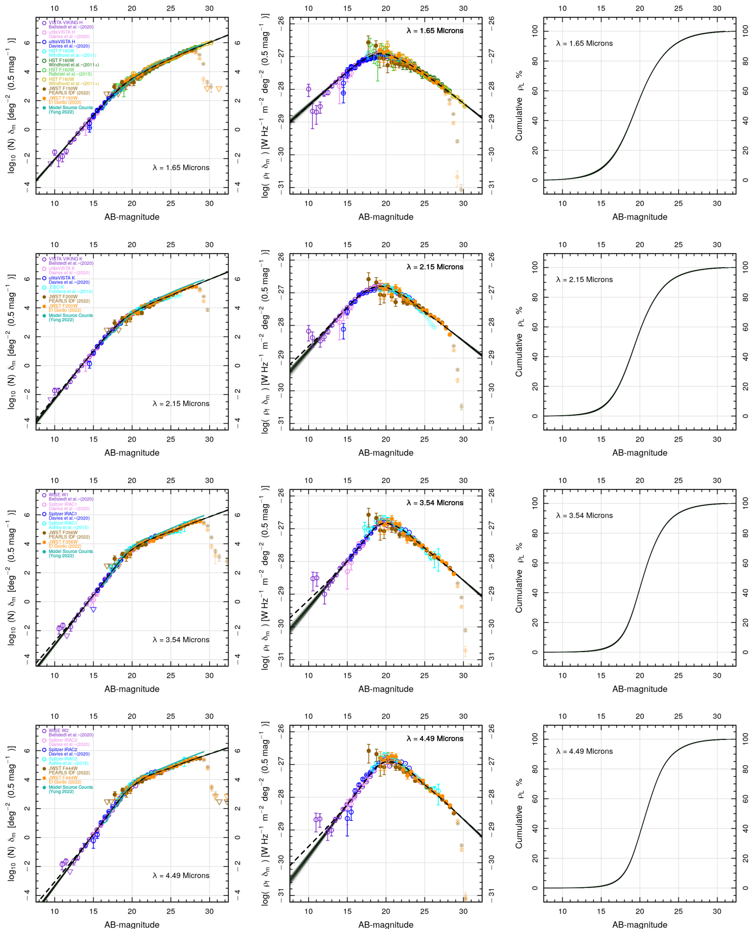
Figure 10. Same as Figure 9 for the ground-based+HST 1.6 & 2.2 \mu\text{m} and Spitzer 3.5 & 4.5 \mu\text{m} counts with JWST NIRCcam counts in F150W, F200W, F356W and F444W as brown/olive filled circles in the JWIDF and El Gordo non-cluster module.
