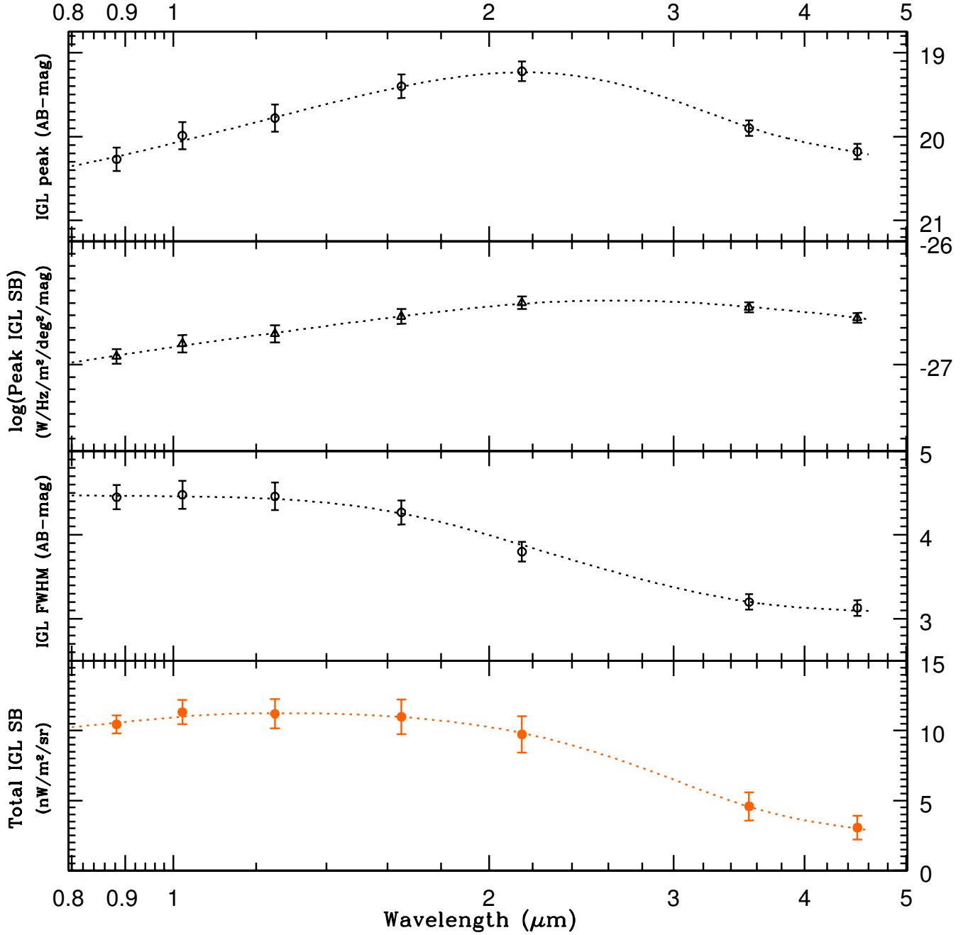
Figure 11. Parameters of the 0.9–4.5 \mu\text{m} galaxy counts and integrated galaxy light (IGL) as derived from Figures 9–10. Top panel shows the AB-magnitude level at which the normalized differential counts peak (see middle panels in Figures 9–10). This is where most of the discrete IGL is generated at each wavelength. Second panel shows the peak SB-value of the IGL derived from the middle panels of Figures 9–10. Third panel shows the width around the peak magnitude or interquartile ( i.e. , 25%–75%) range where 50% of the discrete IGL is generated. We refer to this range as the “IGL FWHM.” The bottom panel shows the total IGL values (in units of \text{nW m}^{-2} \text{sr}^{-1} ) of the converging integrals in the right panels of Figures 9–10. Error bars were determined by combining the NIRCam ZP uncertainties of Appendix B.1 with the uncertainties in transforming the NIRCam flux scale to the fiducial flux scale of the VISTA/IRAC filters in Appendix B.2 (see Sections 4.5–4.6).
