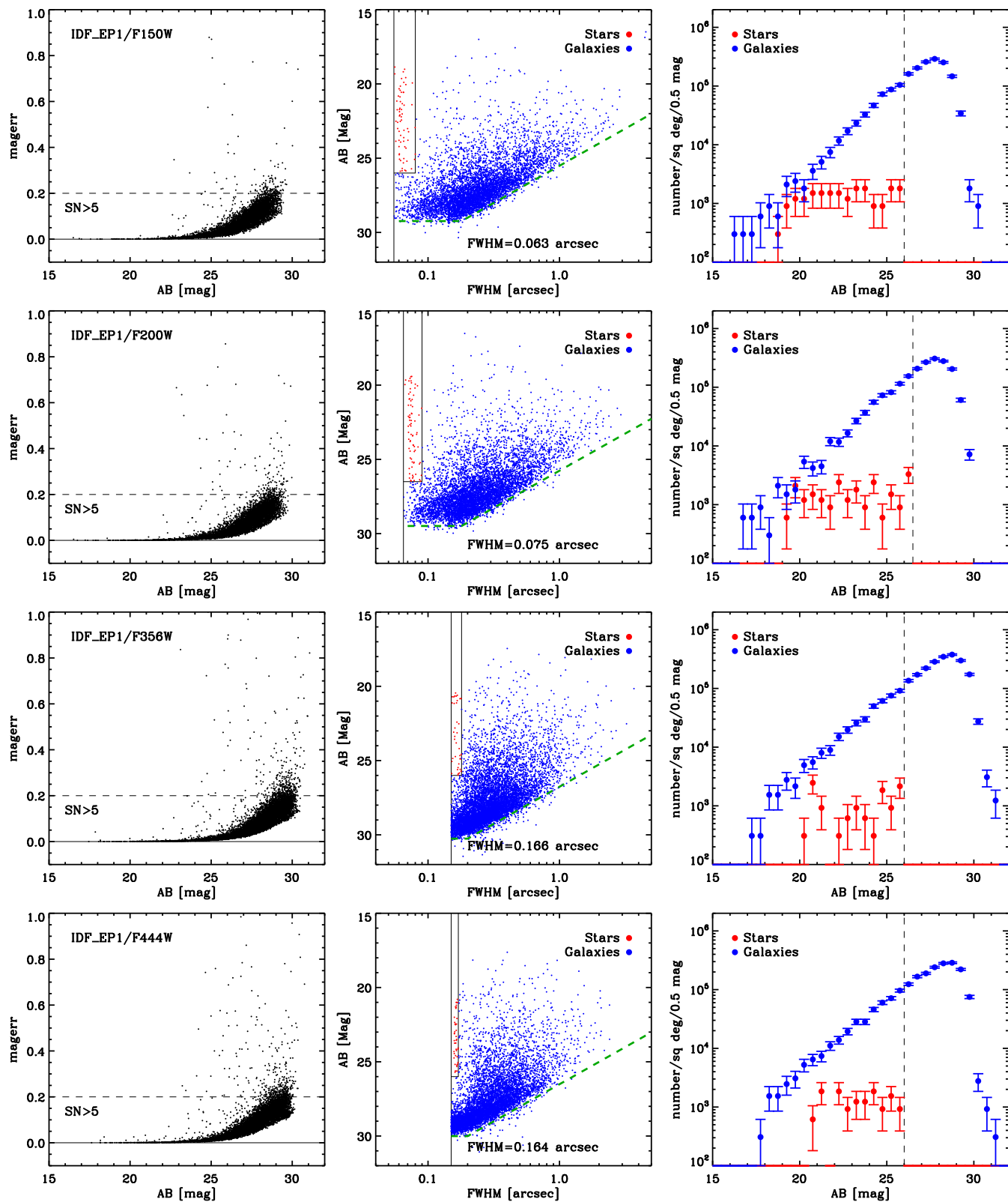
Figure 8. Same as Figure 6 for the object detection, classification, and counts for all detectors covering the JWIDF in the F150W, F200W, F356W, and F444W filters. (Please magnify these figures to see all data points.)
