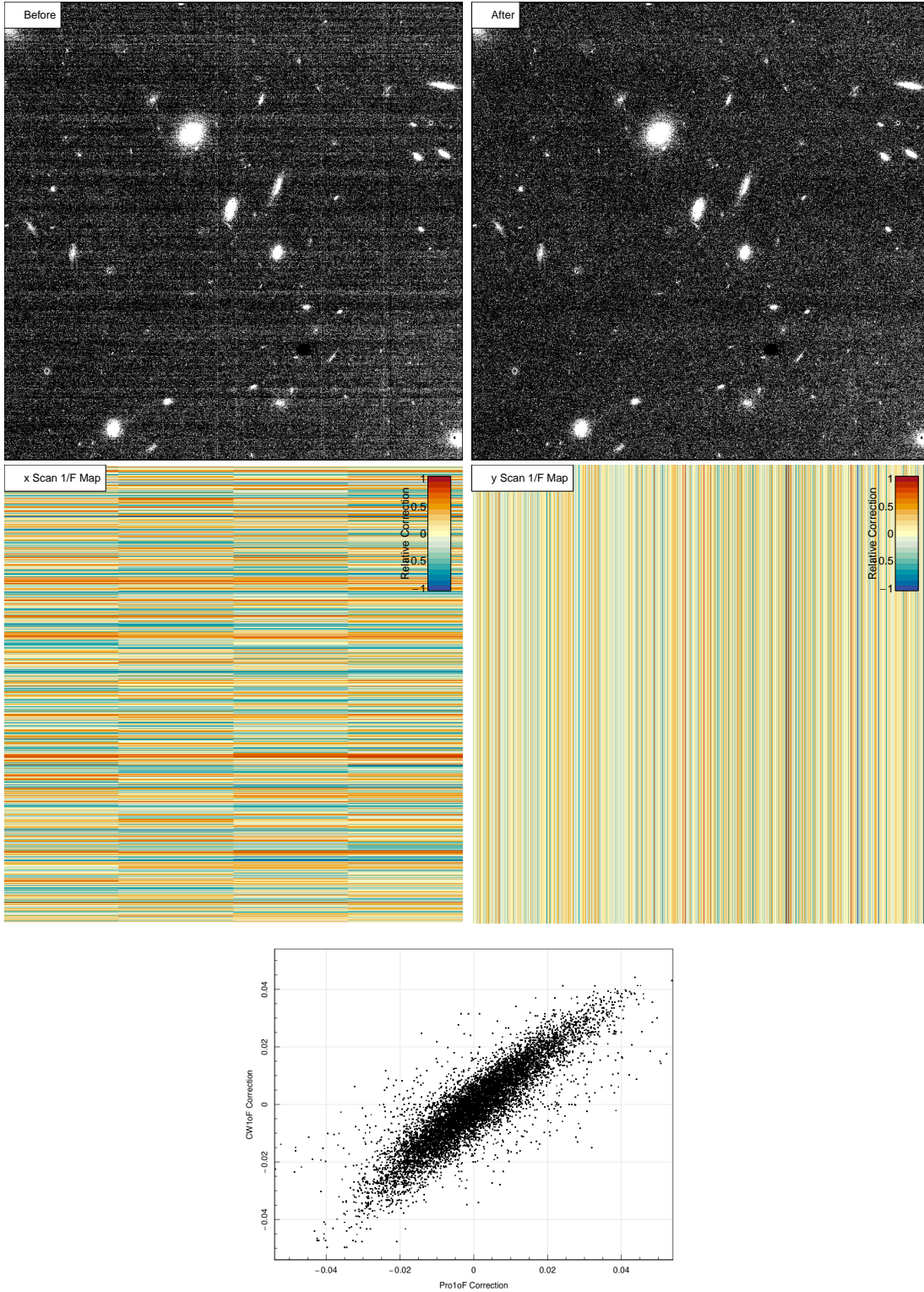
Figure 14. [(a) Top Left ]: Part of the JWIDF image before 1/f removal; [(b) Top Right ]: Same part of the JWIDF image after 1/f removal with the ProFound-based 1/f subtraction code. (Please magnify these figures to see the details); [(c) Middle Left ]: Row-wise 1/f pattern subtracted in the x -direction. The inset color bars show the relative level of the corrections applied. The imprint of the four 5512 \times 2048 pixel sections read by the ASIC is apparent; [(d) Middle Right ]: Column-wise pattern subtracted in the y -direction; [(e) Bottom ]: Comparison of the Willott 1/f-removal algorithm compared to the ProFound-based 1/f subtraction. The two algorithms leave similar noise imprints on the resulting sky-SB at the level of \lesssim 0.02\text{--}0.04 MJy/sr, where 1.0 MJy/sr typically corresponds to a 5\sigma source of AB \sim 28 mag.
