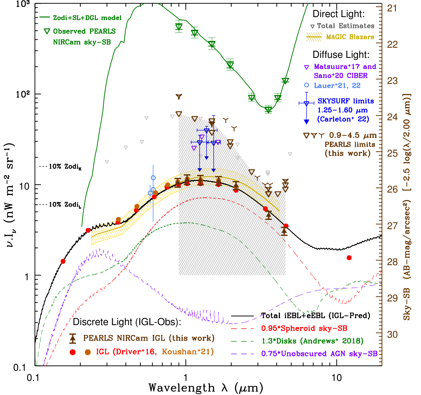
Figure 13. Summary of astrophysical foreground and background energy relevant to PEARLS. Dark brown filled upward-pointing triangles with error bars indicate the PEARLS NIRCam 0.9–4.5 \mu\text{m} IGL measurements of Section 4 (Discrete Light), and are lower limits to the total EBL. Dark brown downward-pointing triangles with the grey error wedge indicate our current JWIDF and El Gordo non-cluster 0.9–4.5 \mu\text{m} upper limits to Diffuse Light, with all known components subtracted (see error budget in Section 5 and Appendix C), and are in line with previous limits to Diffuse Light. (Brown starred and tripod symbols indicate the less accurate VV191 and TNJ limits). Green triangles show our 0.9–4.5 \mu\text{m} PEARLS NIRCam sky-SB observations in the El Gordo non-cluster module compared to the models of Section 5 and Figure 12 (green solid line). The left scale indicates the total energy \nu \cdot I_\nu in \text{nW m}^{-2} \text{sr}^{-1} , and the right scale shows the corresponding sky-SB in \text{AB-mag/arcsec}^{-2} at 2.00 \mu\text{m} (which can be scaled to other wavelengths as indicated). Filled circles show previous IGL counts of Driver et al. (2016b) (red) and Koushan et al. (2021) (orange). Solid and dashed colored lines show the (component and total) discrete EBL models from Andrews et al. (2018). The orange line and hashed area show \gamma -ray Blazar EBL constraints from the MAGIC TeV experiments (see e.g., Dwek & Krennrich 2013, for a summary), and light grey triangles indicate total EBL estimates that require accurate modeling of DGL and ZL and still include the IGL (Direct Light). Purple triangles show the Matsuura et al. (2017) and Sano et al. (2020) CIBER estimates of Diffuse Light in excess of the Kelsall et al. (1998) model prediction. Dark blue upper limits are the SKYSURF 1.25–1.6 \mu\text{m} Diffuse Light limits from 34,000 WFC3/IR images of Carleton et al. (2022) and Windhorst et al. (2022). Light blue circles with error bars at 0.61 \mu\text{m} are the Lauer et al. (2021, 2022) Diffuse Light estimates with New Horizons at 43–51 AU. All Diffuse Light estimates plotted in color have the IGL (=iEBL+eEBL) already subtracted. See Carleton et al. (2022) for a discussion of possible causes of any remaining Diffuse Light.
