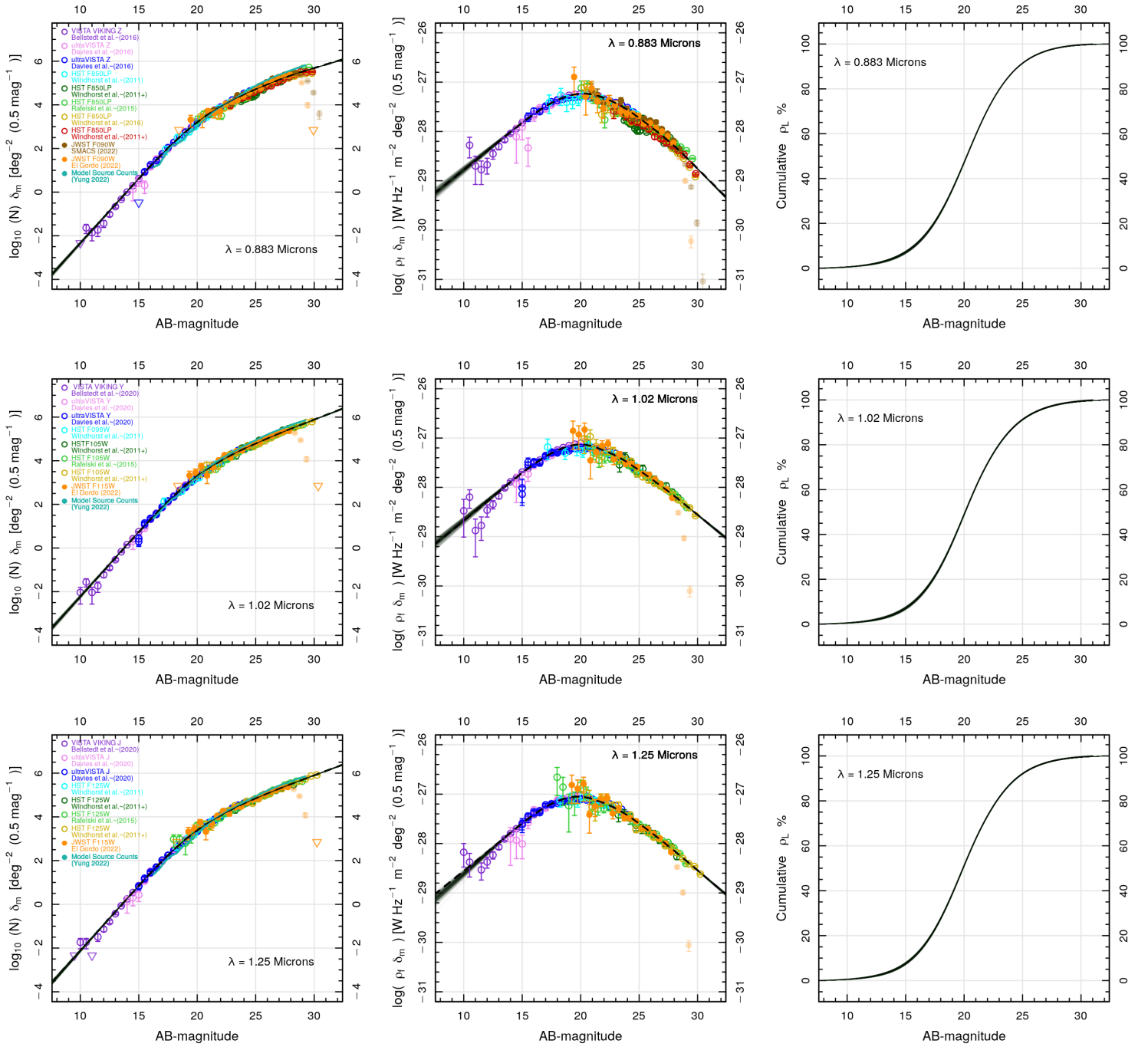
Figure 9. NIRCam galaxy counts in the JWIDF and the El Gordo non-cluster module (orange and brown filled circles, respectively). Each row of three panels shows one wavelength as indicated in the panels. (a) [Left panels]: Differential galaxy counts in 0.5-mag bins. Open diamonds show a combination of previous ground-based, HST, and Spitzer/WISE counts (Driver et al. 2016b; Koushan et al. 2021) with different surveys shown in different colors as indicated in the legends. The green lines represent the hierarchical-model predictions for the 0.9–4.5 \mu\text{m} galaxy counts of Yung et al. (2022). When broad-band filters in different instruments are similar but not identical, small corrections for effective wavelength differences may be needed (Koushan et al. 2021; Robotham et al. 2020, see Appendix B.2 here). (b) [Middle panels]: Energy counts after dividing the left panels by a 0.40 dex/mag slope. Units used are described in Section 4 and Koushan et al. (2021). Triangles without error bars indicate bins having only a single object. The brightest bins of the PEARLS counts at 18 \lesssim \text{AB} \lesssim 20 mag show Cosmic Variance (Section 2 & 4.5), but do not weigh into the IGL fits, which at these flux levels are dominated by the faint end of the brighter surveys. PEARLS counts beyond the respective 80% completeness limits (as derived in Table 1 from a best-fit power-law extrapolation) are plotted as lightly shaded points, and are not included in the spline extrapolations to estimate the total IGL. (c) [Right panels]: Integral of the middle panels normalized to 100% of the IGL energy received.
