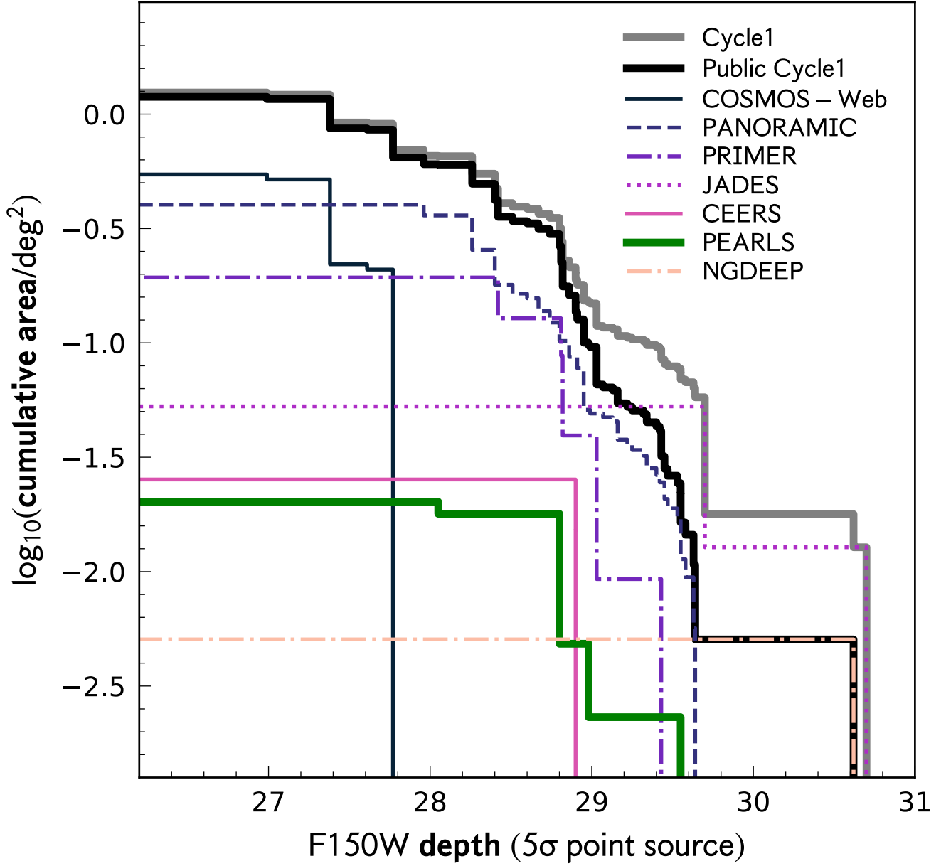
Figure 1. Summary of the area and depth covered by JWST Cycle 1 surveys. Data came from G. Brammer’s website https://erda.ku.dk/vgrid/Gabriel_Brammer/JWST-Cycle1/full_timeline.html . Colors and line types identify seven GO and GTO surveys as shown in the legend, and the order in the legend matches the maximum survey area as shown along the left ordinate. The thick black line shows the total area–depth of all public Cycle 1 surveys, and the thick grey line shows the same including surveys with proprietary data. The thick green line indicates PEARLS, which combines a smaller area of significant depth with a much larger area of 16 shallower fields to significantly average over Cosmic Variance (Section 2 & 4.5), and include 7 lensing clusters.
