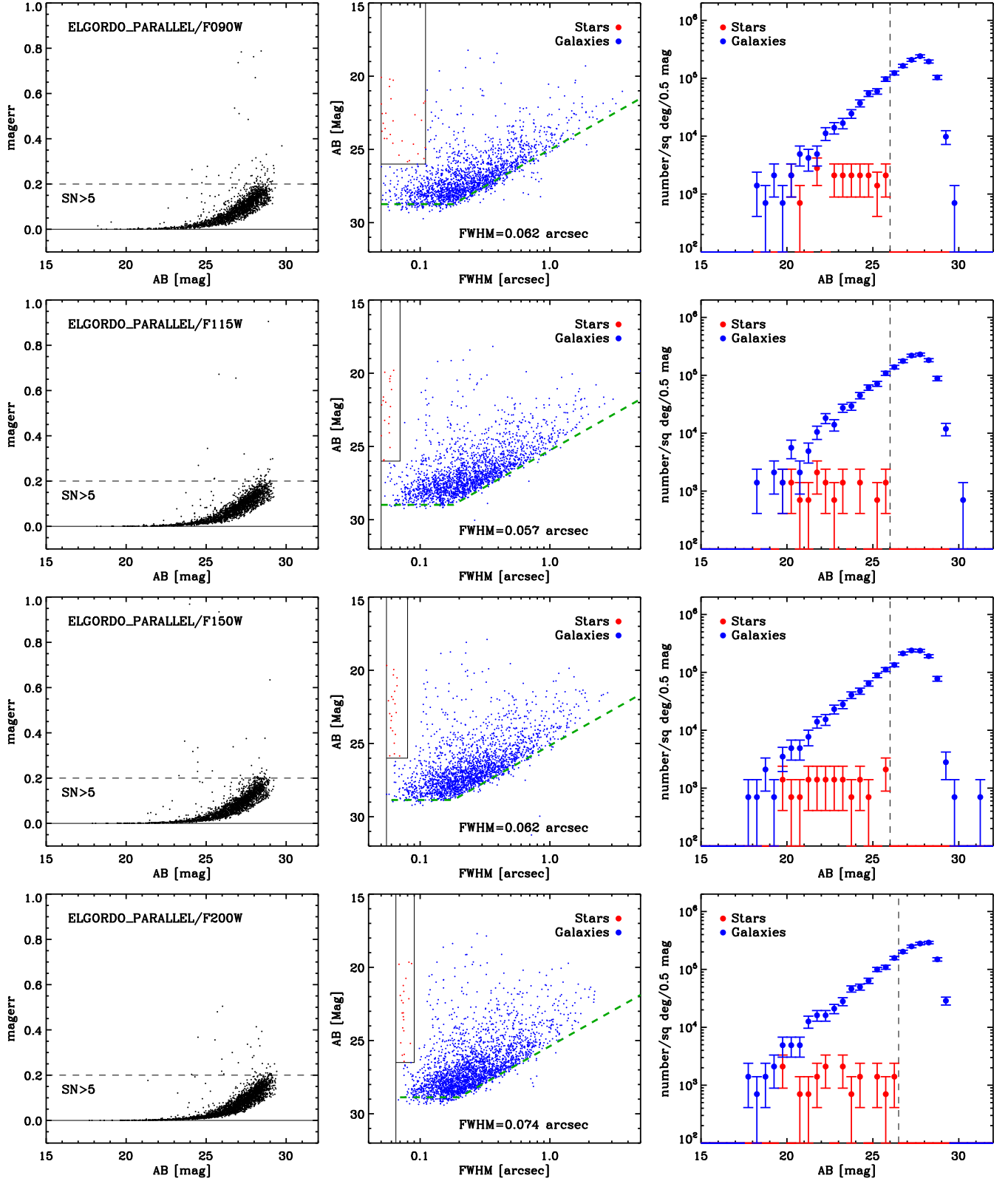
Figure 6. Object detection, classification, and counts in the El Gordo non-cluster module in the F090W, F115W, F150W, and F200W filters. (a) [Left]: SourceExtractor AB-magnitude error bars vs. MAG_AUTO AB-mag resulting from the adopted SourceExtractor-parameters (Section 3.1). Horizontal dashed lines show the adopted 5\sigma point-source detection limits (Table 1). (b) [Middle]: Star-galaxy classification diagram based on SourceExtractor MAG_AUTO AB-magnitudes vs. image FWHM. Left solid vertical lines indicate the NIRCcam diffraction limit for each image with its current sampling. Blue points represent galaxies. The box to the right of the vertical line identifies objects classified as stars (red points). Objects with \text{FWHM} < \text{FWHM}(\text{PSF}) have been flagged and removed from this plot as spurious detections or border imperfections. The green dashed lines indicate for each image the effective point source (horizontal) and SB (slanted) detection limits. (c) [Right]: Resulting star counts (red) and galaxy counts (blue). The vertical dashed line is the limit to which stellar objects are defined.
