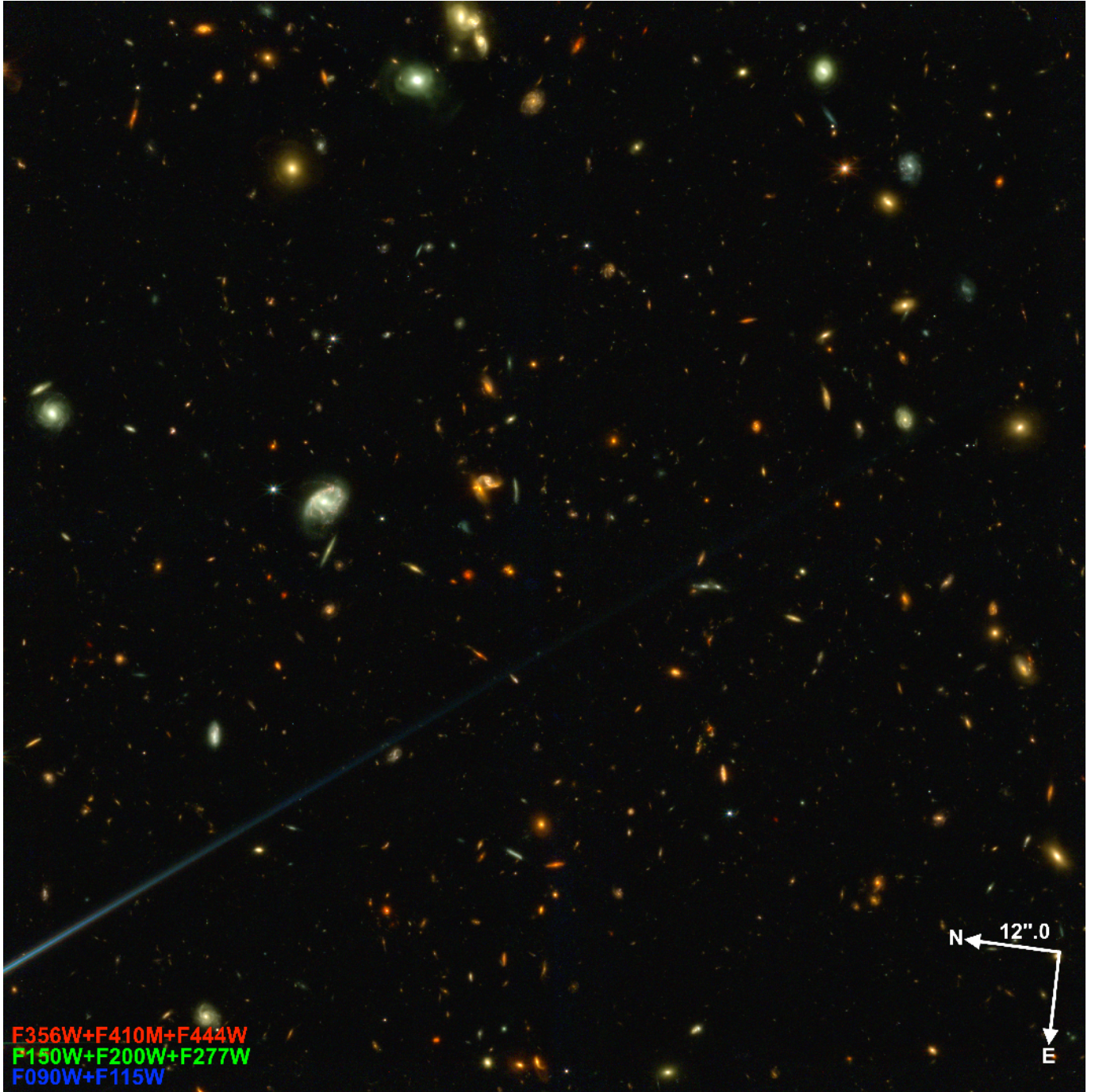
Figure 3. PEARLS NIRCам image of the El Gordo module 3' away from the cluster. Filters F090W+F115W are rendered as blue, F150W+F200W+F277W as green, and F356W+F410M+F444W as red. This El Gordo 4466×4424 pixel section covers 134".0×132".7, and image orientation is shown by the labeled arrows. Areas with remaining detector border effects and bright-star diffraction spikes ( e.g. , the blue spike from a bright star just outside the lower-left FOV) were masked before making object catalogs and counts.
