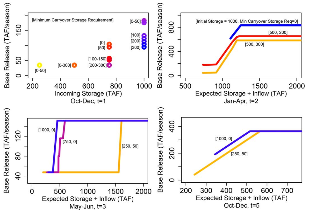
Figure 7. Each line (or point as in the case of t = 1 ) is a base release planning schedule with the optimized release policy given each period's water availability (equation (2)) for each of 28 initial and carryover storage cases.
