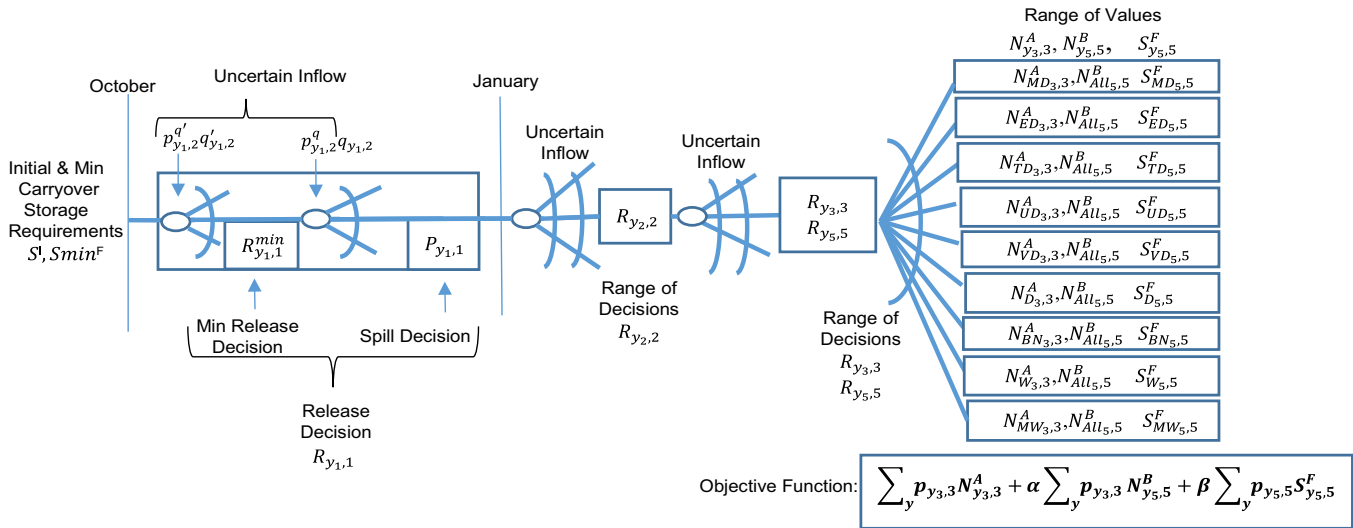
Figure 2. Decision tree for a three-stage optimization model for maximizing fish survival. Each release decision R_{y,t} includes a drought management decision R_{y,t}^{\min} and a flood management decision P_{y,t} .
