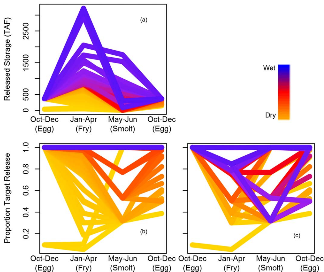
Figure 8. Each line represents expected releases over time for a range of inflow states (a) as a proportion of the release target (b) with and (c) without spill, over time, with initializing model storage conditions of 500 TAF and minimum carryover storage requirements of 200 TAF. Planning release schedules exclude spill.
