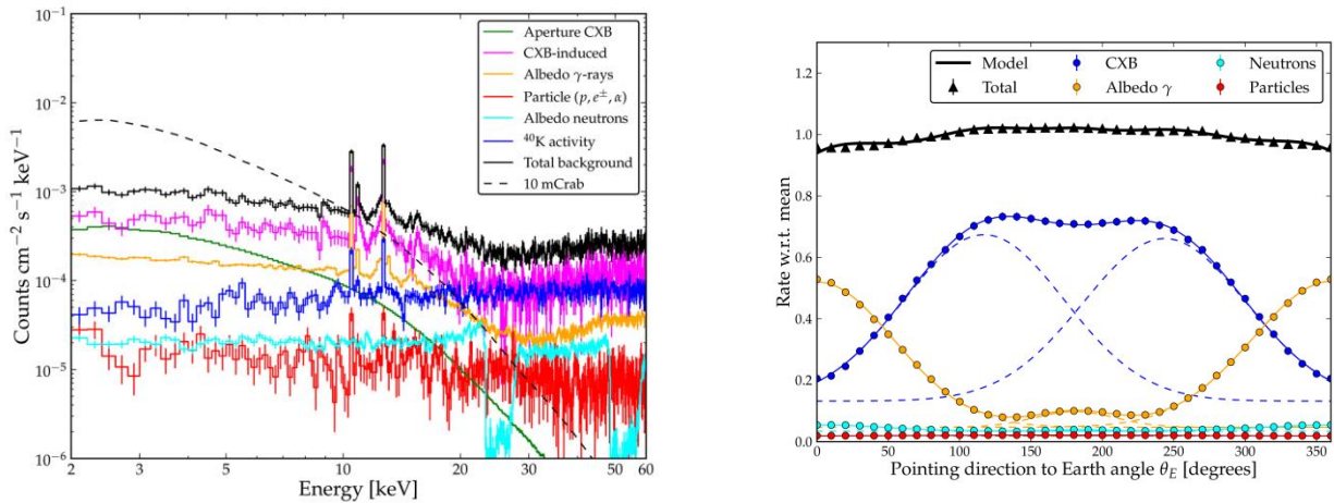
Figure 7: the background estimation for the LAD experiment, as derived by a detailed Monte Carlo simulation including a full geometrical description. Left : The black solid line shows the total background (sum of all components). The dashed line reports the energy-dependent requirement. Right : the orbital modulation of the total background rate (black line) and the individual components.
