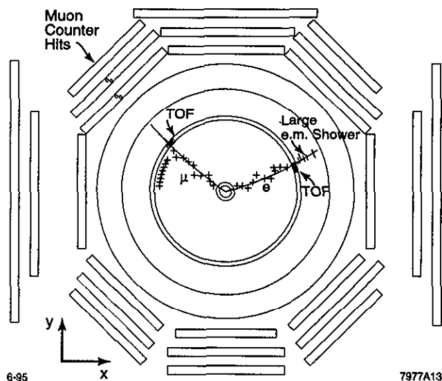
FIG. 13. A typical e\mu candidate event in x - y projection. The MDC hits provide dE/dx information on each track; in addition, both tracks activate the barrel TOF counters as indicated, and hence have associated velocity measurements. The electron track ends in a large shower in the electromagnetic calorimeter, which contributes significantly to its identification as an electron, while the muon track penetrates the shower counter, the magnet coil, and two layers of the muon system.
