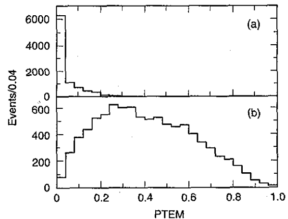
FIG. 7. The distribution in the variable PTEM for (a) the \tau^+\tau^- candidate sample after the application of the particle identification criteria and (b) \tau^+\tau^- events from the Monte Carlo simulation selected by the same criteria.
