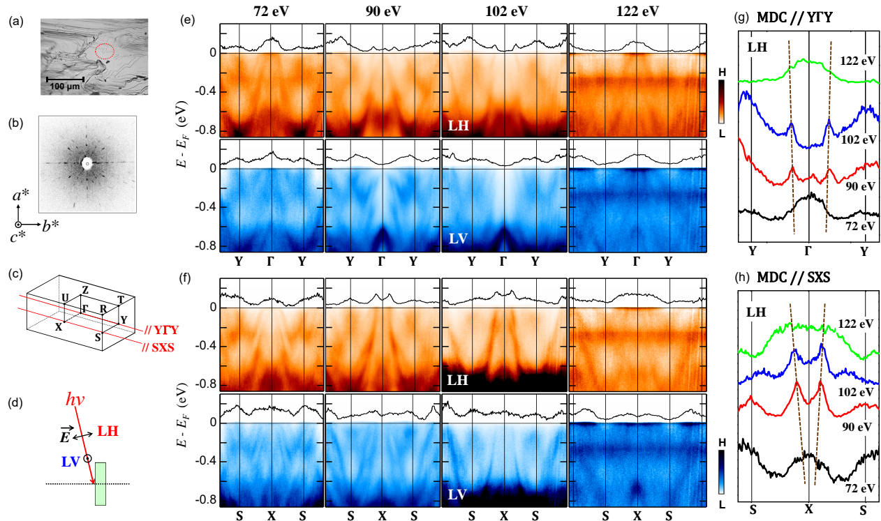
FIG. 2. (Color online) ARPES data of CeNiSn for different h\nu 's. (a) The optical-microscopy (OM) image of a typical surface, which was measured after ARPES measurements were done. The size of the incident photon beam is drawn as a red dotted ellipse. (b) The Laue pattern of the (001) surface, for which ARPES measurements were done. (c) The 3D BZ of the orthorhombic CeNiSn with the YTY and SXS symmetry lines being marked in red, along which ARPES data shown in (e) and (f) are obtained. (d) The schematic drawing of the ARPES measurement geometry with the linear horizontal (LH) polarization and the linear vertical (LV) polarization. (e),(f) The measured ARPES image plots of CeNiSn along YTY and SXS, respectively, obtained with various h\nu 's of 72 eV, 90 eV, 102 eV, and 122 eV. The data in the top and bottom panels were obtained with the LH and LV polarizations, respectively. These data were obtained at T \sim 20 K. On top of each ARPES, the corresponding momentum distribution curve (MDC) at E_F is displayed. (g) Stack of the MDCs of the E_F -states along YTY from 72 eV to 122 eV, obtained with the LH polarization. (h) Similarly for the MDCs along SXS.
