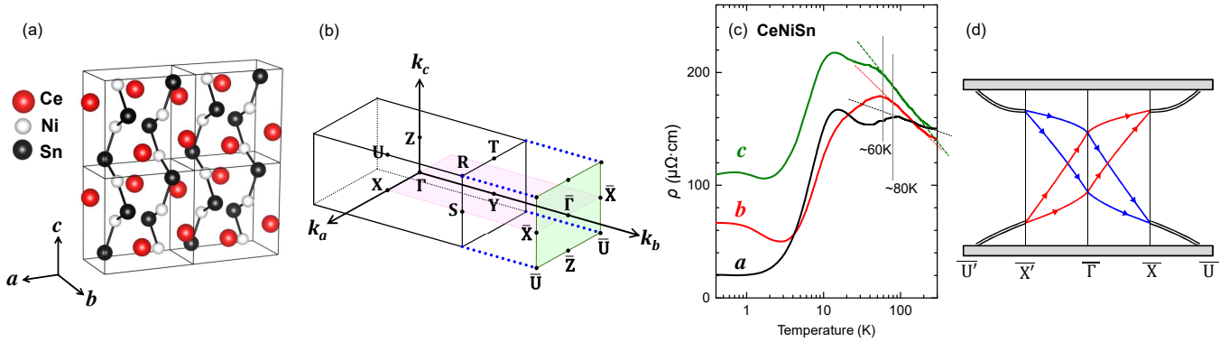
FIG. 1. (Color online) Crystal structure and electrical resistivity of CeNiSn. (a) \epsilon -TiNiSi-type orthorhombic crystal structure of CeNiSn. (b) The Brillouin zone (BZ) for the orthorhombic crystal structure, where the (010) surface BZ projected along k_b is marked in green. (c) T -dependent electrical resistivity \rho(T) data of the purified single crystal of CeNiSn along a , b , and c directions [21, 24]. (d) Two-dimensional (2D) plot of a pair of Möbius-twisted surface states on the (010) surface BZ, which is adopted from Ref. [12]. Here red and blue lines denote the states with positive and negative glide eigenvalues, respectively. Double lines along \bar{X}\bar{U} and \bar{X}'\bar{U}' denote the doubly degenerate surface states.
