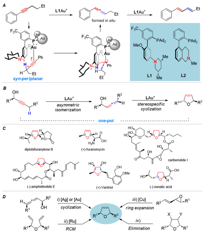
Scheme 1. Soft Propargylic Deprotonation and Chiral 2,5-Dihydrofuran Synthesis
