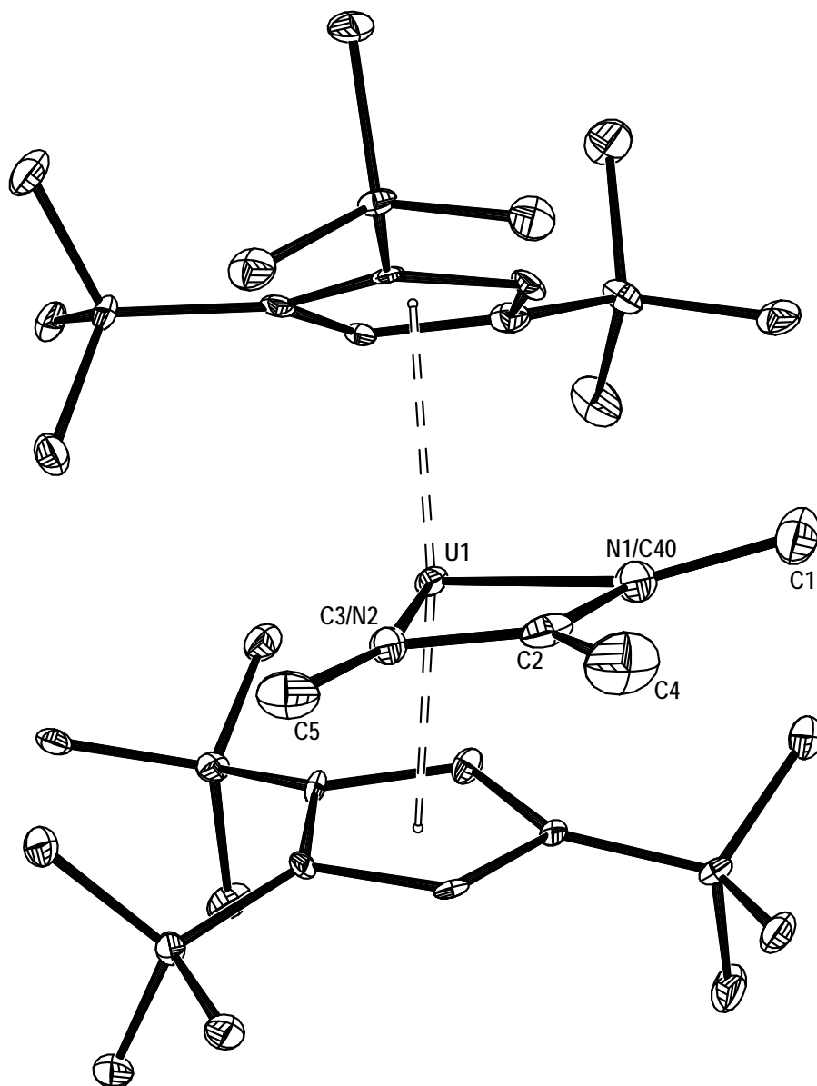
Figure 3. ORTEP drawing of [\eta^5\text{-}1,2,4\text{-(Me}_3\text{C)}_3\text{C}_3\text{H}_2]_2\text{U}[\text{N}(\text{Me})\text{C}(\text{Me})=\text{C}(\text{Me})] ( 15 ) with 35% thermal ellipsoids. Selected bond lengths (Å) and angles (°): Cp'(cent)-U1 2.55 and 2.56, U1-N1/C40 2.202(6), U1-C3/N2 2.270(6), C2-N1/C40 1.410(9), C2-C3/N2 1.390(9), Cp'(cent)-U1-Cp'(cent) 138.7, N1/C40-U1-C3/N2 65.1(2), N1/C40-C2-C3/N2 118.5(7).
