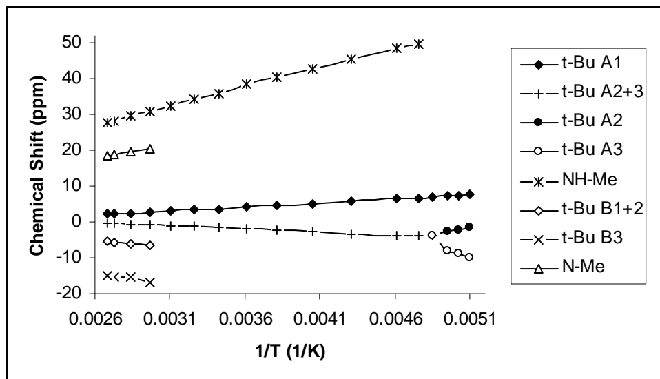
Figure 1. Plots of \delta versus 1/T for [\eta^5\text{-}1,2,4\text{-(Me}_3\text{C)}_3\text{C}_5\text{H}_2]_2\text{U(NHMe)}_2 ( 8 ) in \text{C}_7\text{D}_8 (for \text{Me}_3\text{C} , \text{NH-Me} and \text{N-Me} groups).
