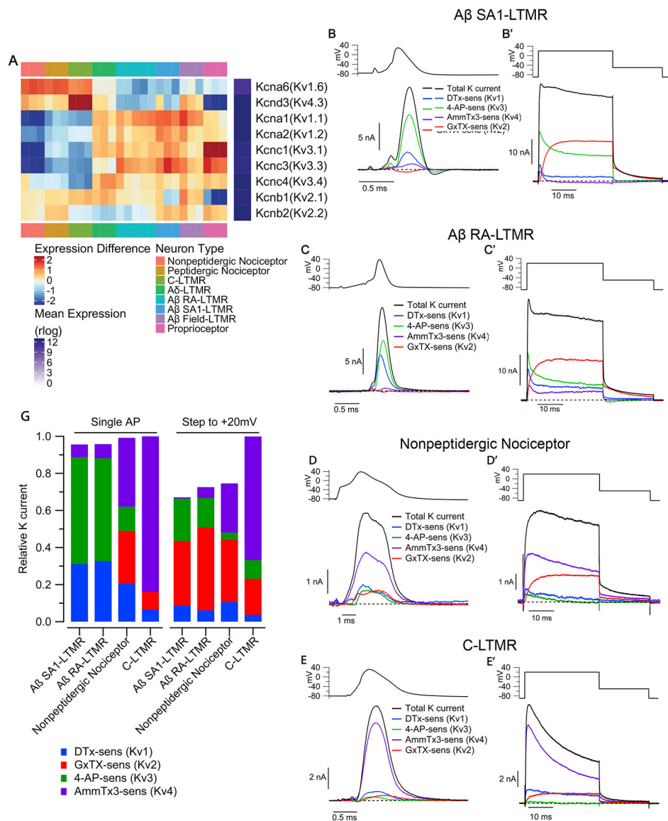
Figure 5. Kv channel families differentially contribute to outward current in sensory neuron subtypes
