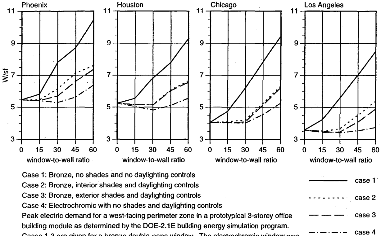
Figure 1. Peak electric demand ( W/ft^2 ) for a west-facing perimeter zone
