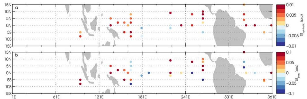
Figure 9. (a) Salinity at the time of the local ascending Aquarius pass (around 18:00) minus salinity at the time of the local descending Aquarius pass (around 06:00). Salinities are taken from the fits to 1 m mooring salinities (Figure 3); only sites with statistically significant fits are plotted. (b) Mean difference between Aquarius descending-node and ascending-node salinities based on Aquarius measurements made within 100 km of each mooring site. Note the different color scales in Figures 9a and 9b.
