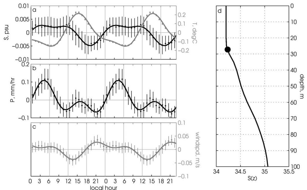
Figure 4. As in Figure 2, but for the mooring at 147E,2N. Evaporation and MLD were not available at this site, so they are not shown.
