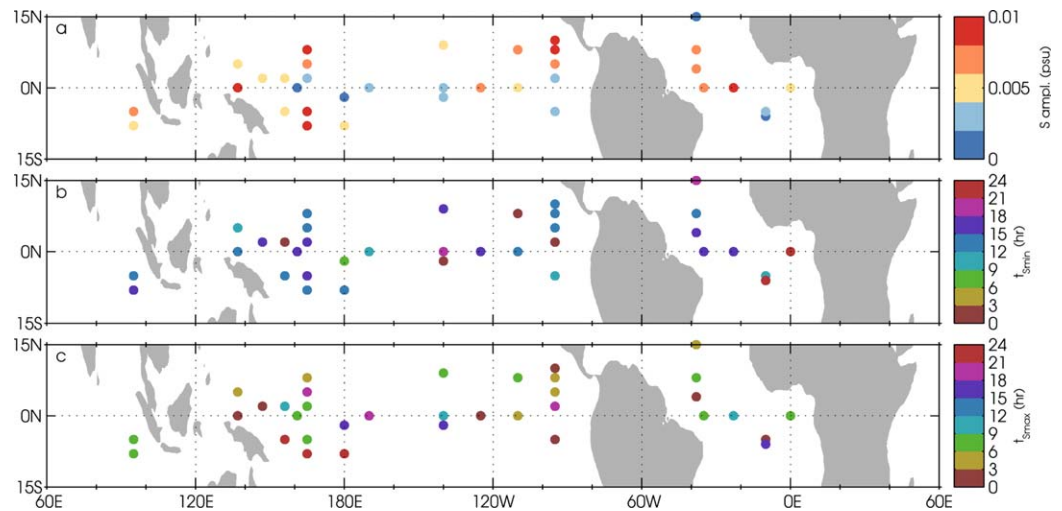
Figure 3. Characteristics of the daily salinity cycle, obtained by fitting diurnal and semidiurnal harmonics to high-passed 1 m depth salinity anomalies at each mooring site: (a) amplitude, computed as half the maximum minus minimum salinities; (b) time of minimum daily salinity (local hour); and (c) time of maximum daily salinity (local hour). Diurnal amplitudes at all sites are statistically significant.
