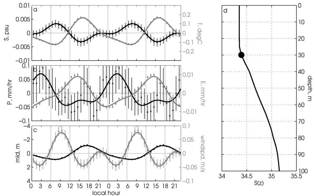
Figure 2. Daily cycles from mooring observations in the western Pacific warm pool: (a) 1 m salinity (black) and temperature (gray); (b) precipitation (black) and evaporation (gray); (c) MLD (black; note the inverted y axis, i.e., positive values indicate deeper mixed layers) and wind speed (gray). The markers and vertical lines represent the average and standard error of all daily anomalies within a given hourly time bin, where daily anomalies were computed by filtering hourly data with a 3 day high-pass filter and then smoothed with a 1-2-1 triangle filter. The solid lines represent the diurnal plus semidiurnal fits to the binned data, and the dotted lines represent the uncertainty on these fits (negligible for the SST signal). All data are plotted as anomalies with respect to the mean, so positive values of a given variable indicate more of that variable at a given hour of day, and negative values indicate less of that variable. Two diurnal cycles (48 h) are shown. (d) Climatological salinity profile (line) and MLD (circle) at the mooring site, from the MIMOC data set. As in Figure 1, all measurements were made at the 156E,2N mooring site, except evaporation, which was made at the 165E,0N mooring, and MLD, which was made at the 154E,0N site.
