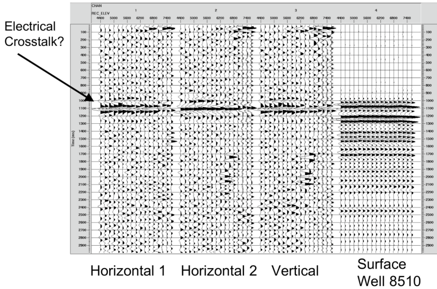
Figure 3: Stacked Data Monitor Well 7545 Source Well 8510
