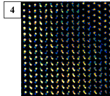
FIG.4 EW phase image in color code of an InGaN QW. Higher phase values (yellow) show the GaN region. More In content leads to lower phase values (darker).
