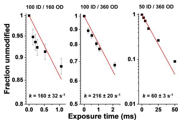
Figure 2. Dose-response plot consisting of microsecond to millisecond irradiation of 10 \mu\text{M} Alexa in 10 mM phosphate buffer (pH 7) using various ID capillary flow exposures. The length of the X-ray window was set to 2 mm for 50 \mu\text{m} , 100 \mu\text{m} , and 200 \mu\text{m} ID capillary flow to obtain the range of exposure times as indicated in Table S1. The solid red line represents a single exponential fit and rate constants are shown. Individual points represent the mean of three independent measurements with standard error. R-squared values for the fit as calculated via Origin® Version 7.5 are 0.44, 0.88, and 0.99 for the left, middle and right plots, respectively. The flow velocity inside the 50 \mu\text{m} and 100 \mu\text{m} tubing are within the jetting regime and up to 100 fold faster than that of the flow velocity inside the 200 \mu\text{m} tubing used for the standard capillary flow method at the unfocused X-ray beamline. (Table S1)
