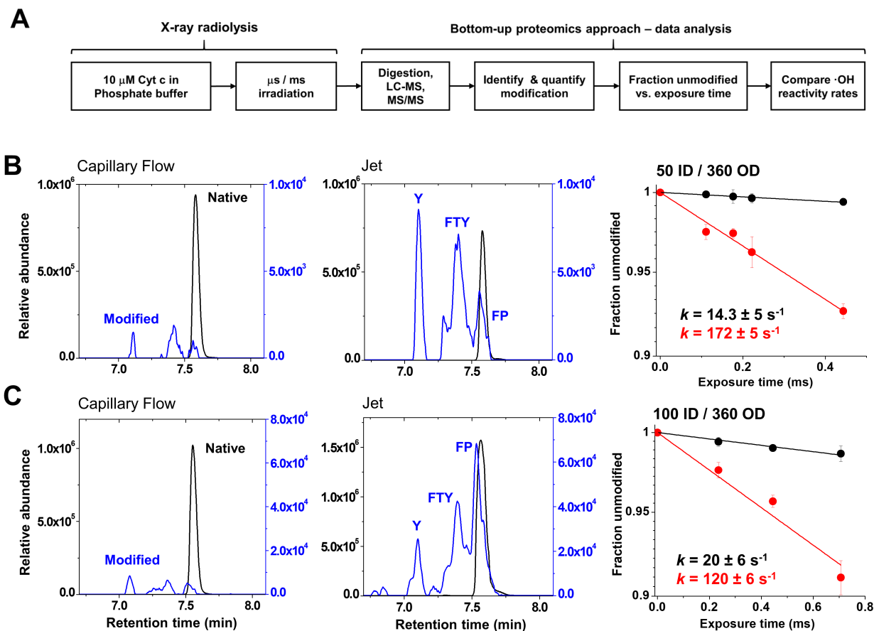
Figure 6. Liquid jet and capillary flow comparison. (A) Experimental scheme. (B) and (C) The left and middle panel show the extracted ion chromatogram of the doubly protonated native (black), and the doubly protonated +16 Da modified products (blue) of the cyt c peptide ^{40}\text{TGQAPGFTYTDANK}^{53} . The modification products eluted as three peaks between 7 and 7.7 min and are shown for the exposed sample at 200 \mu\text{s} using capillary flow or jet with tube ID/OD of 50/360 (B) and 700 \mu\text{s} with tube ID/OD of 100/360 (C). Figure 6. The right panels show the fraction of unmodified peptide, which is calculated as the unmodified peak area divided by the sum of unmodified and modified peak areas at a given exposure. The solid line represents a single exponential fit to determine the hydroxyl radical reactivity k ( \text{s}^{-1} ), with individual points representing the mean of three independent measurements with standard deviation, for both jet (red) and capillary (black) data. R-squared values for the fit as calculated via Origin® Version 7.5 are between 0.97 and 0.99 for all fits. The site of modification at Y48, F46, T47, and P44 were identified by MS/MS according to the standard MS/MS m/z assignment method (Figure S5) 3,19 .
