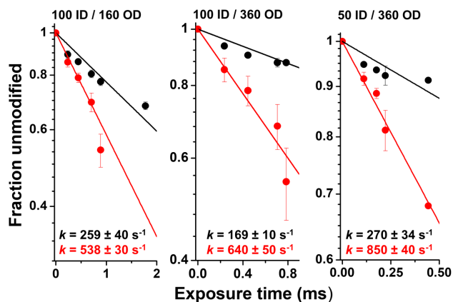
Figure 5. Liquid jet results in a higher dose in the Alexa assay. Dose-response plot consisting of microsecond irradiation of 10 \mu\text{M} Alexa in 10 mM phosphate buffer (pH 7) using microfluidic capillary flow (black) and liquid jet (red) exposure set-up at high flow rates in the jetting regime. The length of the X-ray window was 2 mm and two types of tube ID were used as indicated. The solid line represents a single exponential fit to initial data points and determines the rate constant ( k \text{ s}^{-1} ), with individual points representing the mean of three independent measurements with standard error. R-squared values for the fit as calculated via Origin® Version 7.5 are 0.88, 0.91 and 0.59 (from left to right panel) and 0.96, 0.94, and 0.98 for the capillary and jet respectively.
