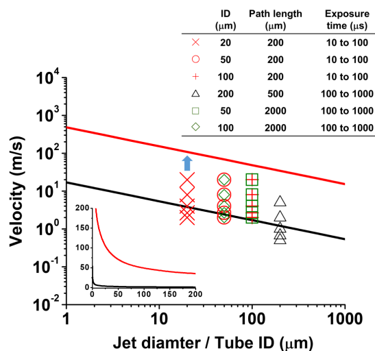
Figure 1. The XFMS jetting regime is defined by flow velocity, exposure time, and area of exposure. Jetting regime is shown within the lower (black) and upper (red) limit of flow velocity determined from the Weber number (Equations 3 and 4) as a function of jet diameter. The individual points represent the optimum range of velocities for a given sample diameter and beam size for sample exposure. The green set of points indicate the flow velocity selected for the current study at the unfocused beamline. The black set of points were those used in actual XFMS experiments at the ALS and NSLS II using high-flux density focused X-ray beamlines. The red set of points are the estimated range, based on Alexa dose response and protein side chain modification, used for the development of microsecond XFMS at the ALS. Blue arrow indicates a region of higher flow velocity that will provide shorter exposure, which will be useful to minimize sample damage as well as effectively use the higher flux density at a micro-focused beamline. The inset is the jetting regime plotted in linear scale in order to better show that a much wider choice of flow velocity is available with narrower jets.
