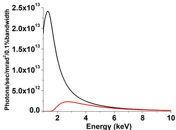
Figure 3 Removal of glass increases photon absorption by the sample. Calculation of photon spectrum for a sample path-length of 50 \mu\text{m} through a 180 \mu\text{m} glass capillary wall (red) and no glass capillary (black), which corresponds to 50 \mu\text{m} ID – 360 \mu\text{m} OD capillary-flow set-up and 50 \mu\text{m} ID liquid jet set-up respectively. Integration of the plots show >5 fold increase in integrated flux by removing the glass wall. A 1 cm path-length in the air was assumed prior to sample exposure. The calculation used an ALS bend magnet spectrum and transmission/absorption coefficients as given by the Center for X-Ray Optics website (cxro.lbl.gov) calculator. In the case of a 20 \mu\text{m} droplet with and without an 80 \mu\text{m} glass wall, total integrated photons are 10-fold higher than with glass.
