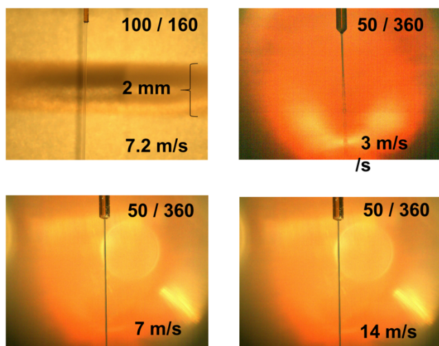
Figure 4. Snapshots of Rayleigh liquid jets for XFMS. The impression of X-ray beam of vertical length \sim 2\text{mm} is shown with the 100 \mu\text{m} ID jet (top left panel). A sample flow velocity lower than in the jetting regime produces unstable jets with breakups (top right panel). Stable jets were seen to travel more than 10 cm distance vertically.
