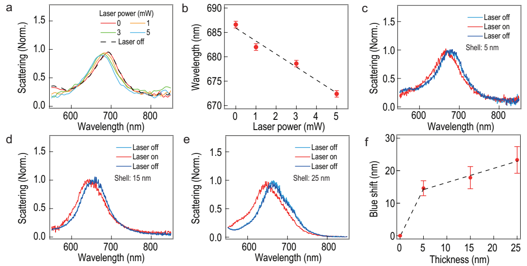
Figure 4. Power- and thickness-dependent plasmon shift of Au@Cu 2-x S NPoMs. (a) Scattering spectra of Au@Cu 2-x S NPoM at different irradiation power. (b) Change in plasmon resonance with irradiation power. (c)–(e) Scattering spectra of Au@Cu 2-x S NPoMs of different shell thickness: (c) 5 nm, (d) 15 nm, (e) 25 nm. Pumping power: 5 mW. (f) Change in blue-shift magnitude with shell thickness. All the error bars are the averaged and squared deviation based on five NPoMs.
