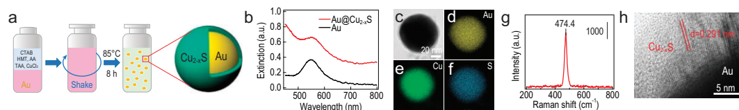
Figure 1. Synthesis of Au@Cu 2-x S core-shell NPs and their characterizations. (a) Synthetic procedure of Au@Cu 2-x S core-shell NPs. (b) Extinction spectra of Au and Au@Cu 2-x S core-shell NPs. (c) TEM and (d)–(f) elemental mapping of the Au@Cu 2-x S NPs. (g) Raman spectrum of Au@Cu 2-x S NPs. (h) HRTEM image of a typical Au@Cu 2-x S core-shell NP.
