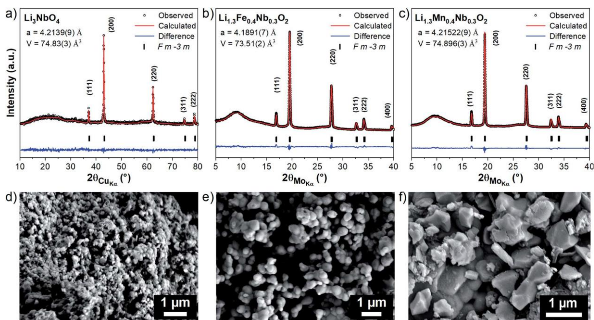
Fig. 2 Rietveld refinements of the XRD patterns and associated SEM images of (a and d) \text{Li}_3\text{NbO}_4 ; (b and e) \text{Li}_{1.3}\text{Fe}_{0.4}\text{Nb}_{0.3}\text{O}_2 ; and (c and f) \text{Li}_{1.3}\text{Mn}_{0.4}\text{Nb}_{0.3}\text{O}_2 obtained by using nano-sized precursors.
