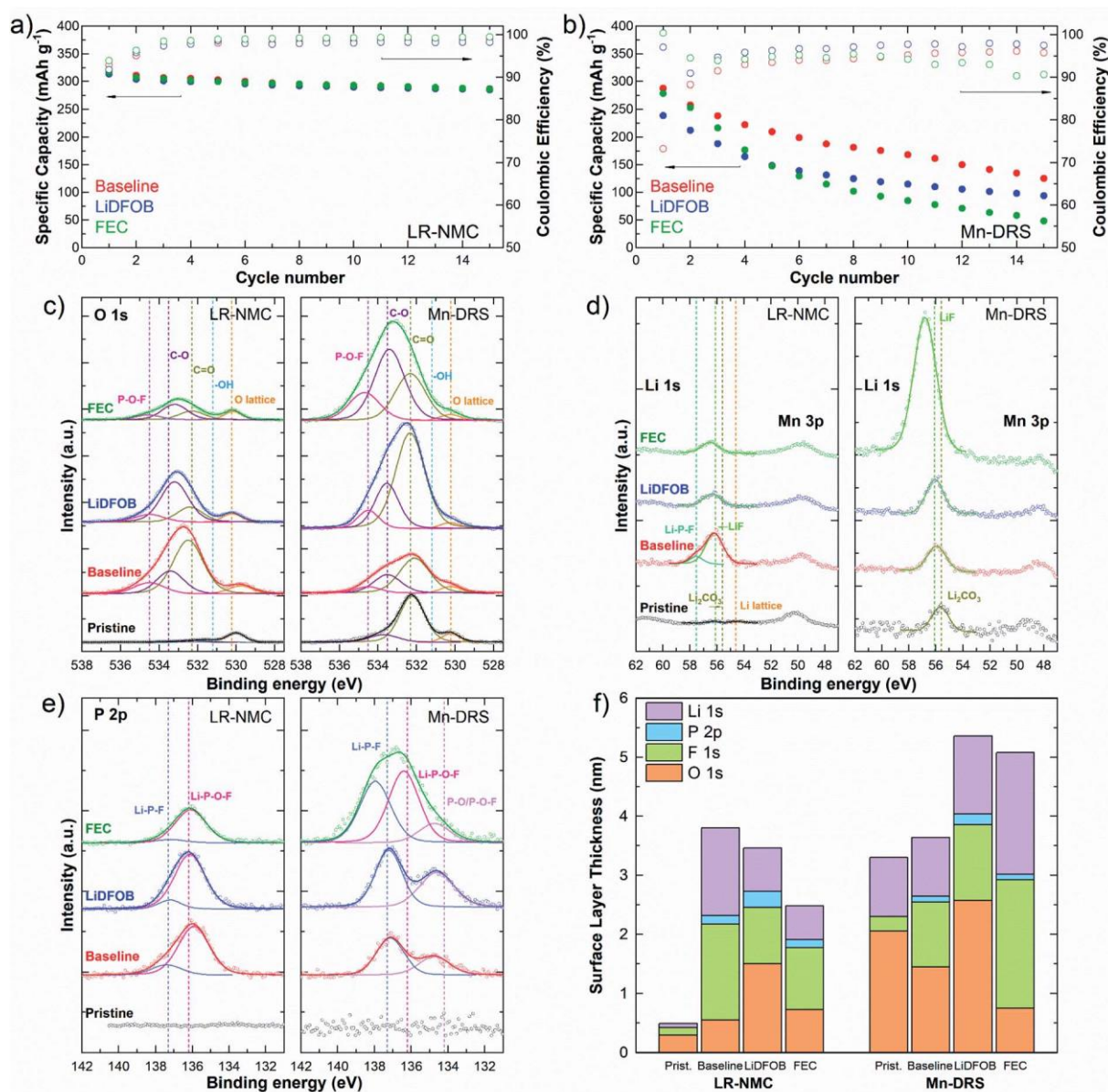
Fig. 6 Cycling stability of (a) [\text{Li}_{0.144}\text{Ni}_{0.136}\text{Co}_{0.136}\text{Mn}_{0.544}]\text{O}_2 (LR-NMC) and (b) \text{Li}_{1.3}\text{Mn}_{0.4}\text{Nb}_{0.3}\text{O}_2 (Mn-DRS) with the 3 different electrolytes studied. XPS spectra of the (c) O 1s, (d) Li 1s–Mn 3p, and (e) P 2p region of LR-NMC and Mn-DRS in the pristine state and after first discharge for the 3 electrolytes tested. (f) Surface layer thickness calculated from the XPS spectra with elemental contribution.
