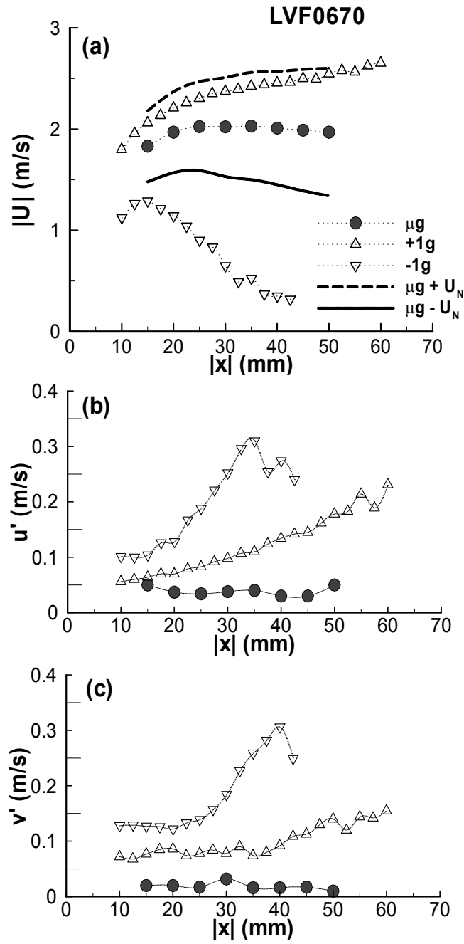
Figure 8 Mean and rms profiles on the centerline of +1g, -1g and \mu g LVF0670
