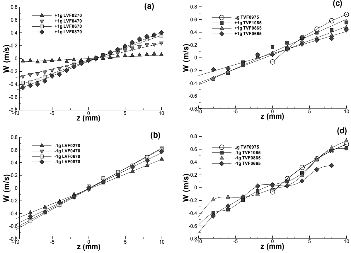
Figure 15 Mean W profiles laminar and turbulent v-flames in +1g and -1g.
