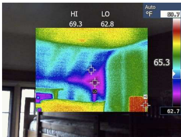
Figure 29 - P2 missing insulation and/or air leakage at bedroom
