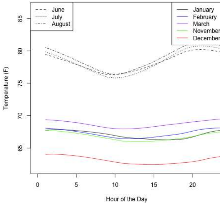
Figure 96 - P6 South, Monthly Living Room Temperature Profiles, Winter and Summer
