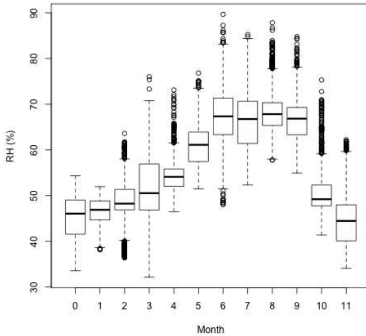
Figure 42 - P2 Summary of 2nd Floor RH
