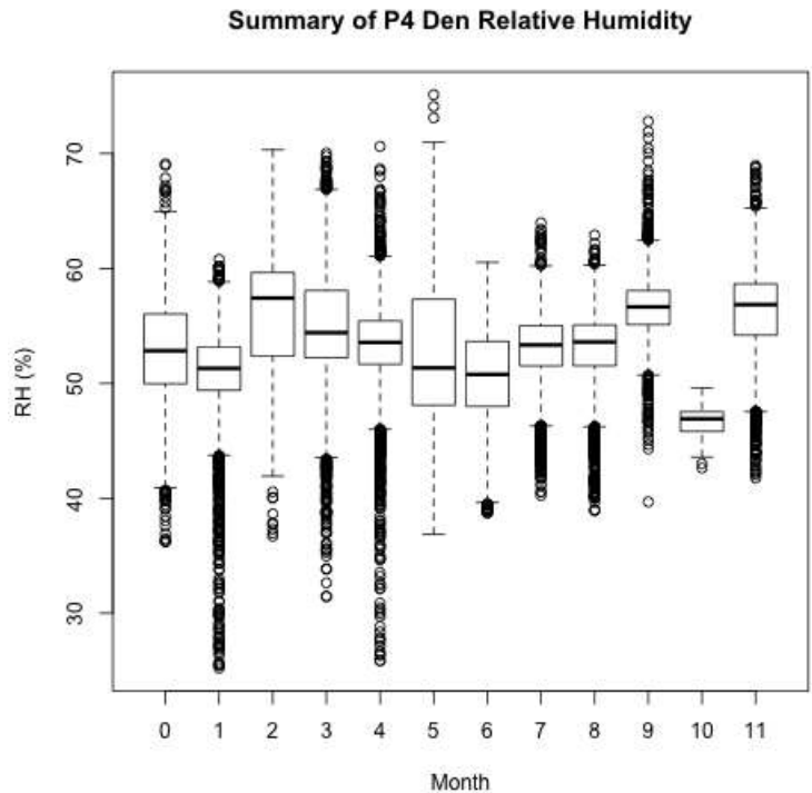
Figure 77 - P4 Summary of Den Relative Humidity
