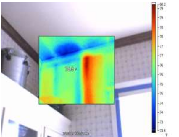
Figure 103 - P7 Pre-retrofit thermal bridges/air leakage in kitchen
