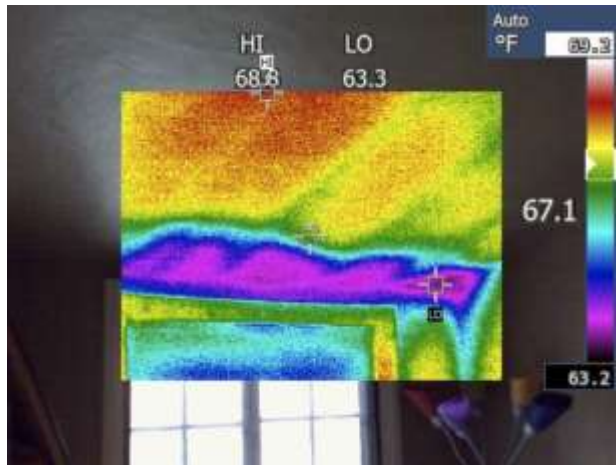
Figure 28 - P2 missing insulation and/or air leakage at bedroom window
