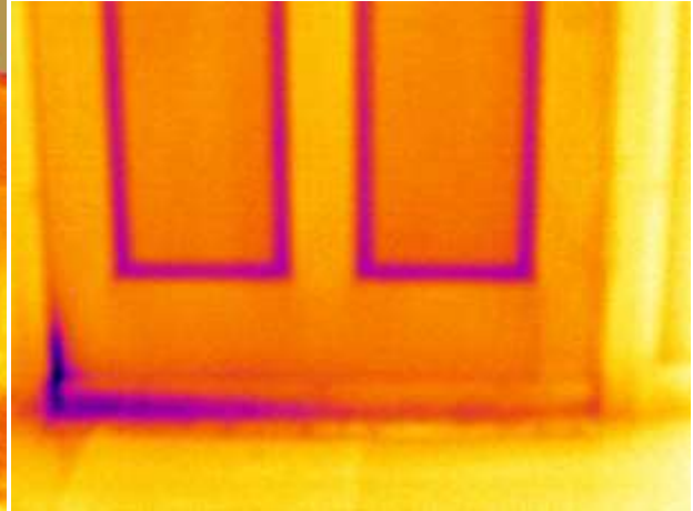
Figure 63 - P4 thermal leakage above honeycomb shade in living room Figure 64 - P4 air leakage around front door
