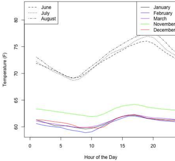
Figure 95 - P6 North, Monthly Living Room Temperature Profiles, Winter and Summer
