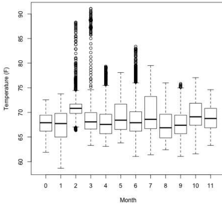
Figure 40 - P2 Summary of 2nd Floor Temperatures
