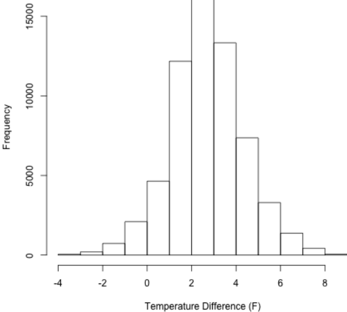
Figure 75 - P4 Histogram of Temperature Differences, Den to Basement Office
