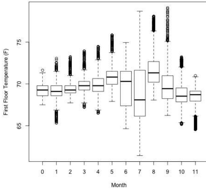
Figure 15 - P1 Boxplots of First Floor Temperatures by Month
