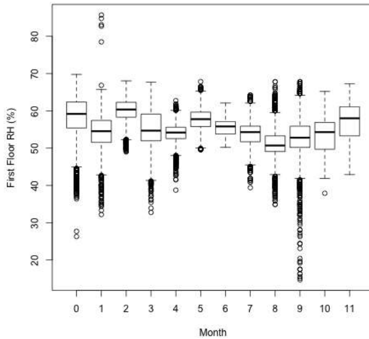
Figure 16 - P1 Boxplots of First Floor Relative Humidity by Month
