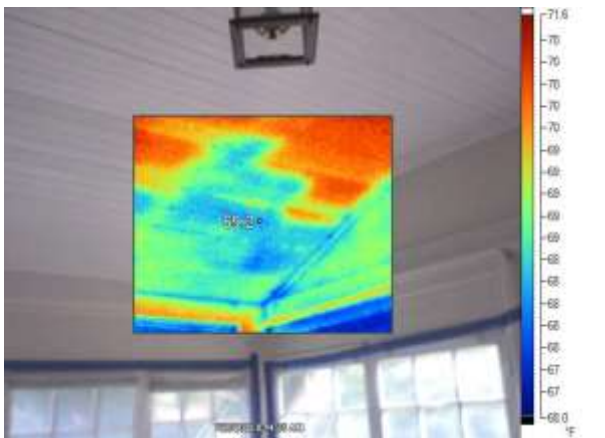
Figure 103 - P7 Pre-retrofit thermal bridges/air leakage in kitchen
