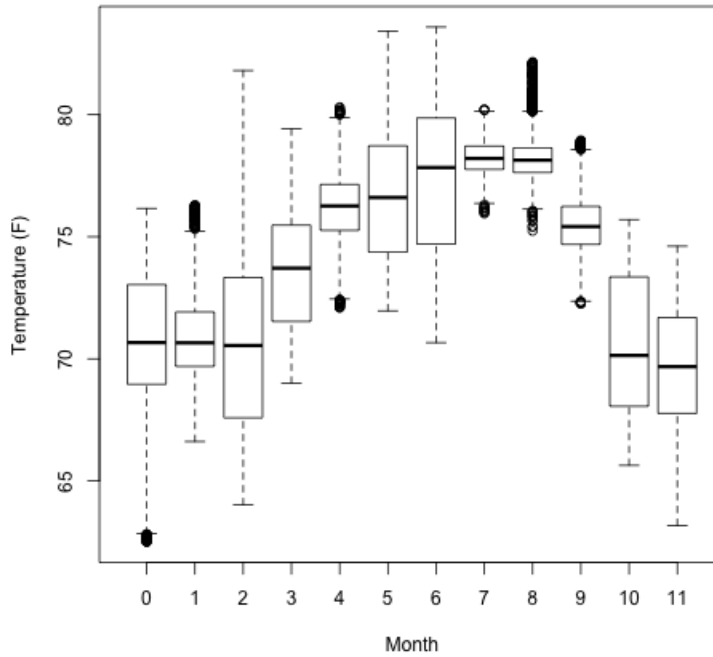
Figure 54 - P3 Summary of Master Bedroom Temperatures
