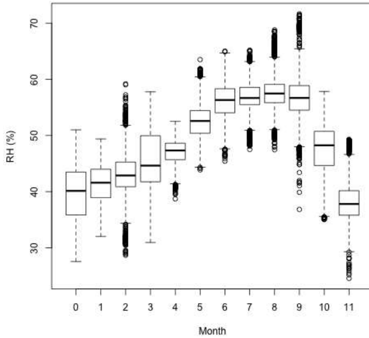
Figure 41 - P2 Summary of 1st Floor RH
