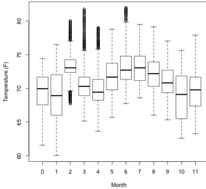
Figure 39 - P2 Summary of 1st Floor Temperatures
