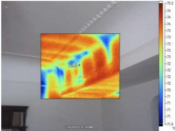
Figure 107 - P7 Pre-retrofit thermal leakage in master bedroom
