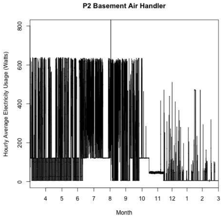
Figure 172 - P2 Basement Air Handler, Illustrating HRV Inconsistency
