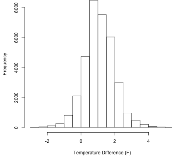
Figure 53 - P3 Histogram of Interior Temperature Differences
