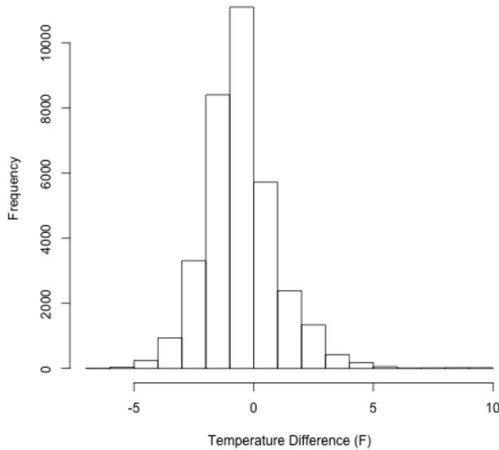
Figure 98 - P6-S Histogram of Temperature Differences
