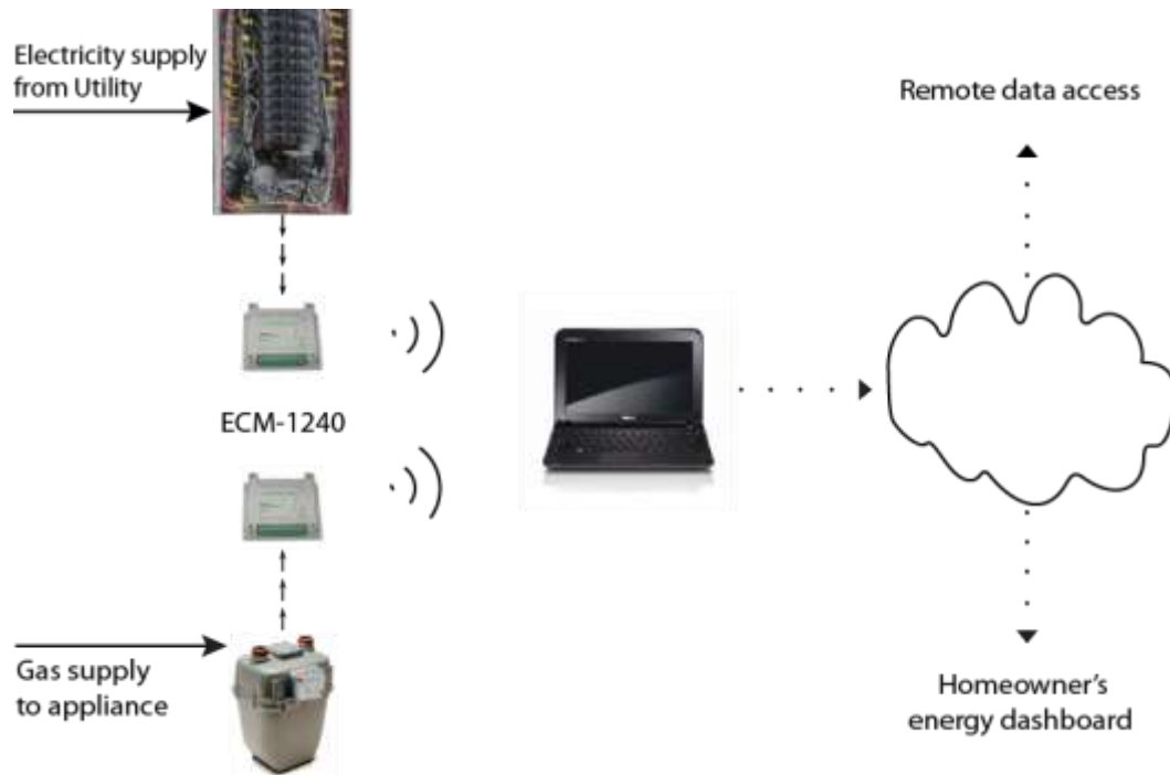
Figure 2 - Communication Schematic
