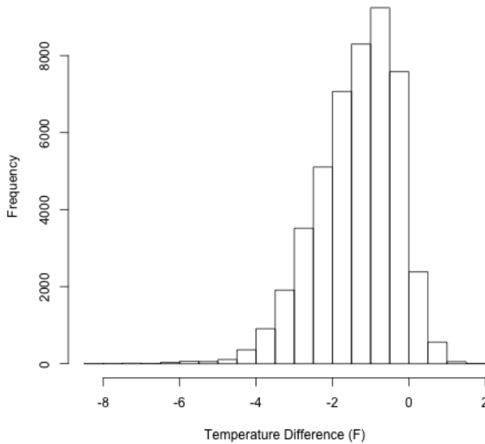
Figure 14 - P1 Histogram of Temperature Differences Between Floors
