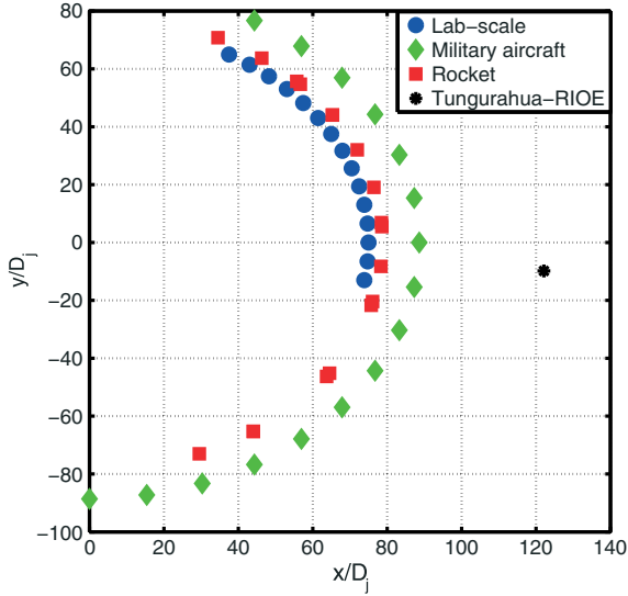
Figure 3. Measurement locations of jet noise directionality from a laboratory-scale jet, a full-scale military jet aircraft, and a full-scale rocket motor, as compared to a volcano acoustics field experiment at Tungurahua volcano. The measurement locations are scaled by the expanded jet diameter D_j . In the case of Tungurahua, D_j is assumed to be 300 m. The nozzle exit is at approximately (0,0) and the exhaust is pointed in the positive direction along the y axis.
