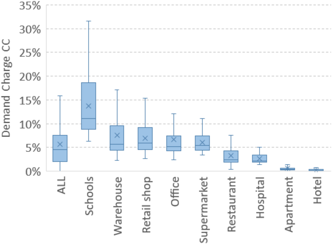
Range within each building type due to location and orientation.
