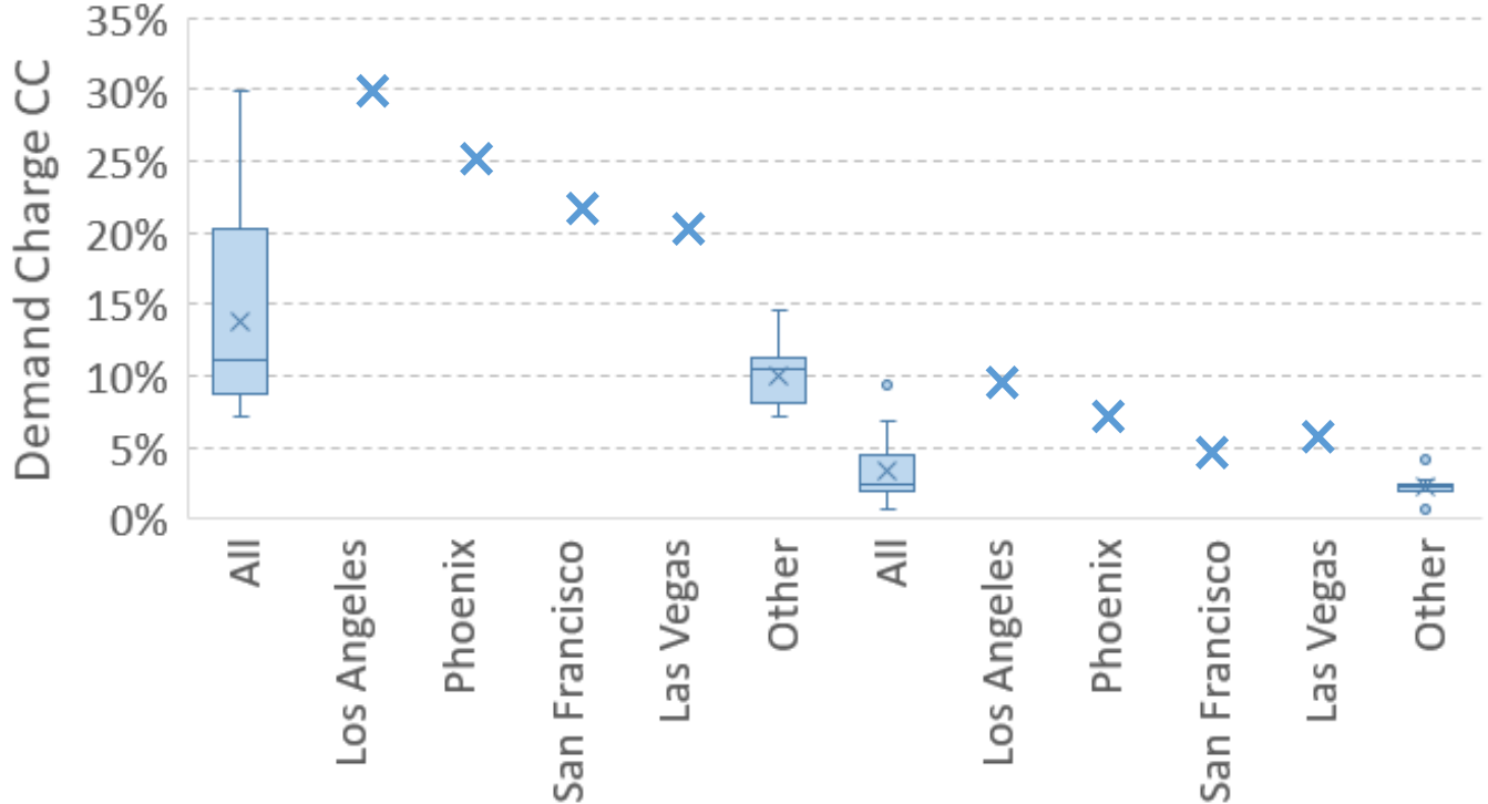
Demand charge capacity credit for schools (left) and restaurants (right) in various locations
