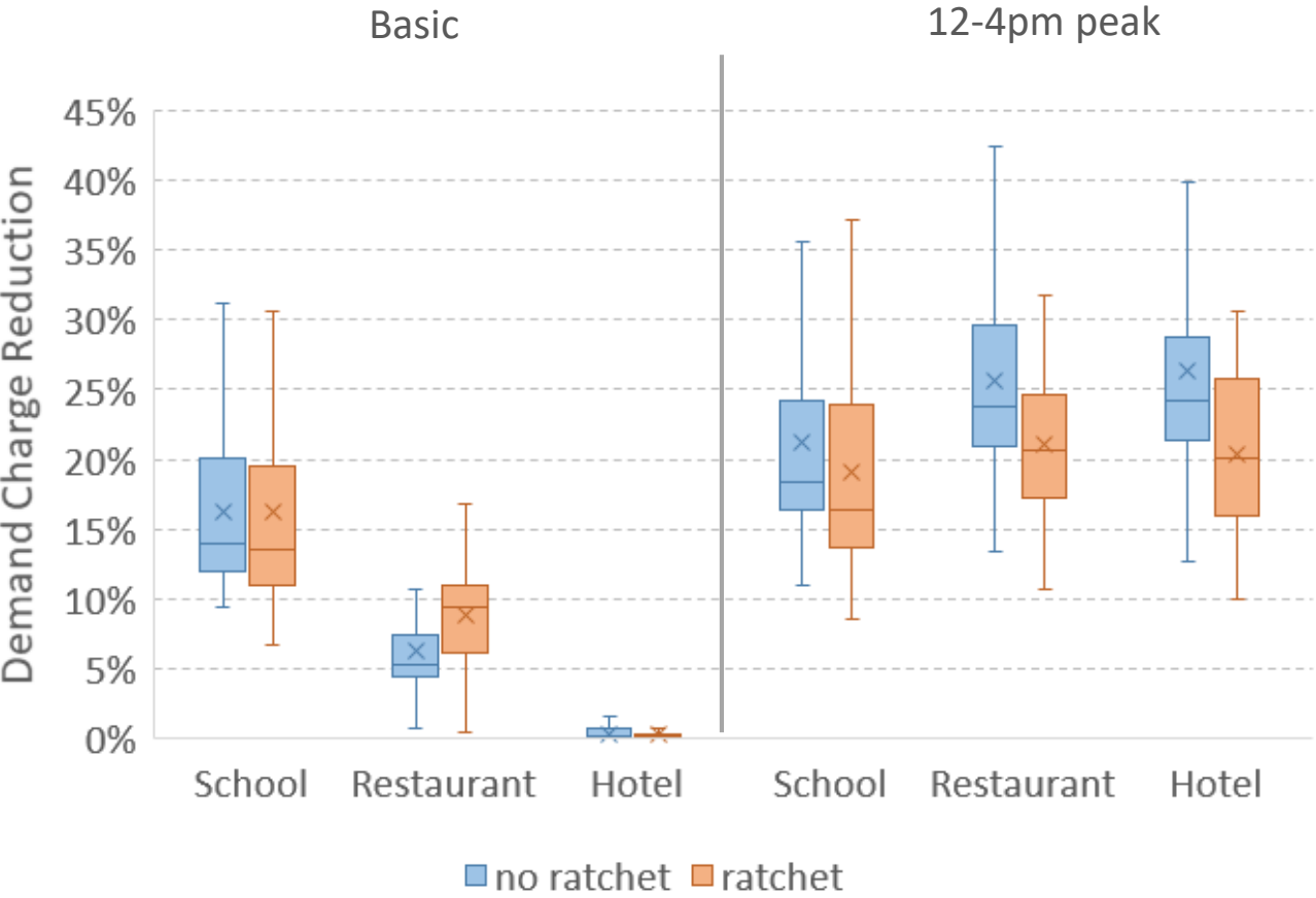
The figure shows the demand charge reductions for PV systems that generate half of the customer’s annual load (i.e. 50% PV-to-load ratio), to eliminate variability due to PV system size. Range within each building type is due to location and orientation.
