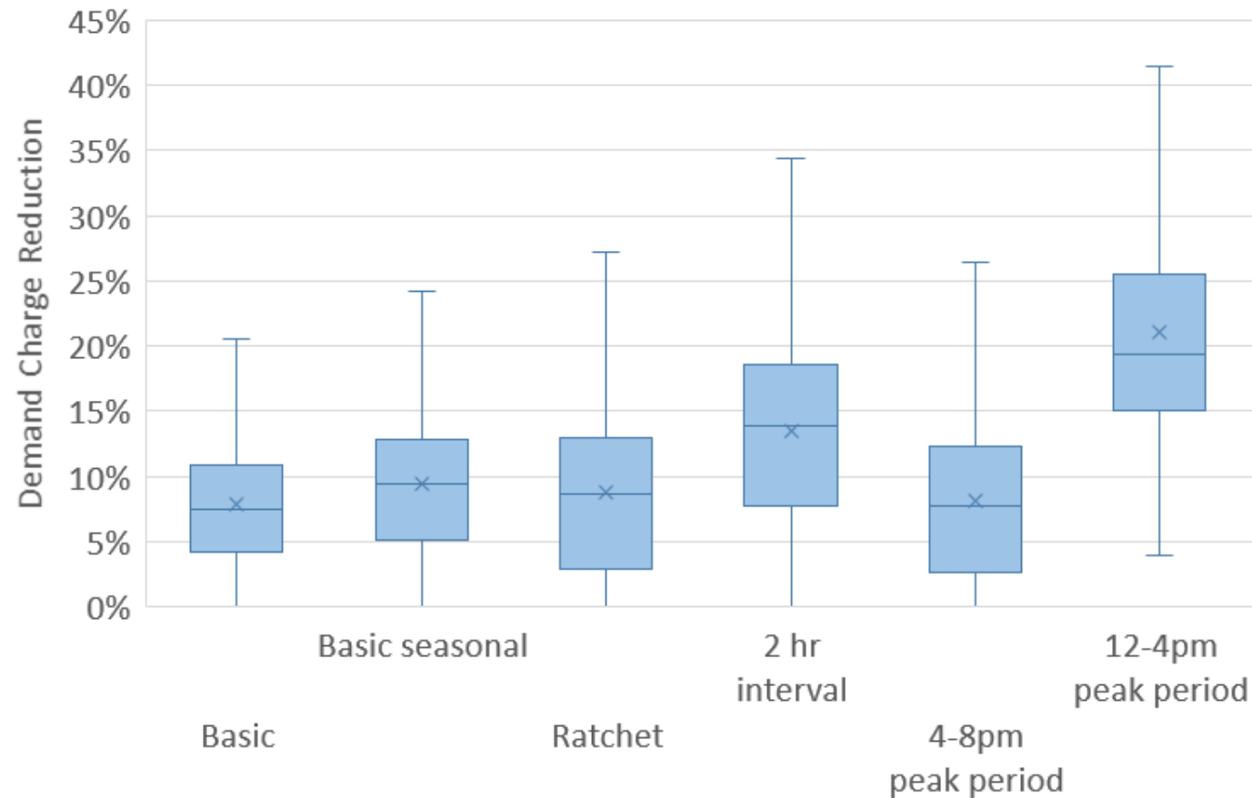
Distribution of demand charge reductions for various demand charge designs
