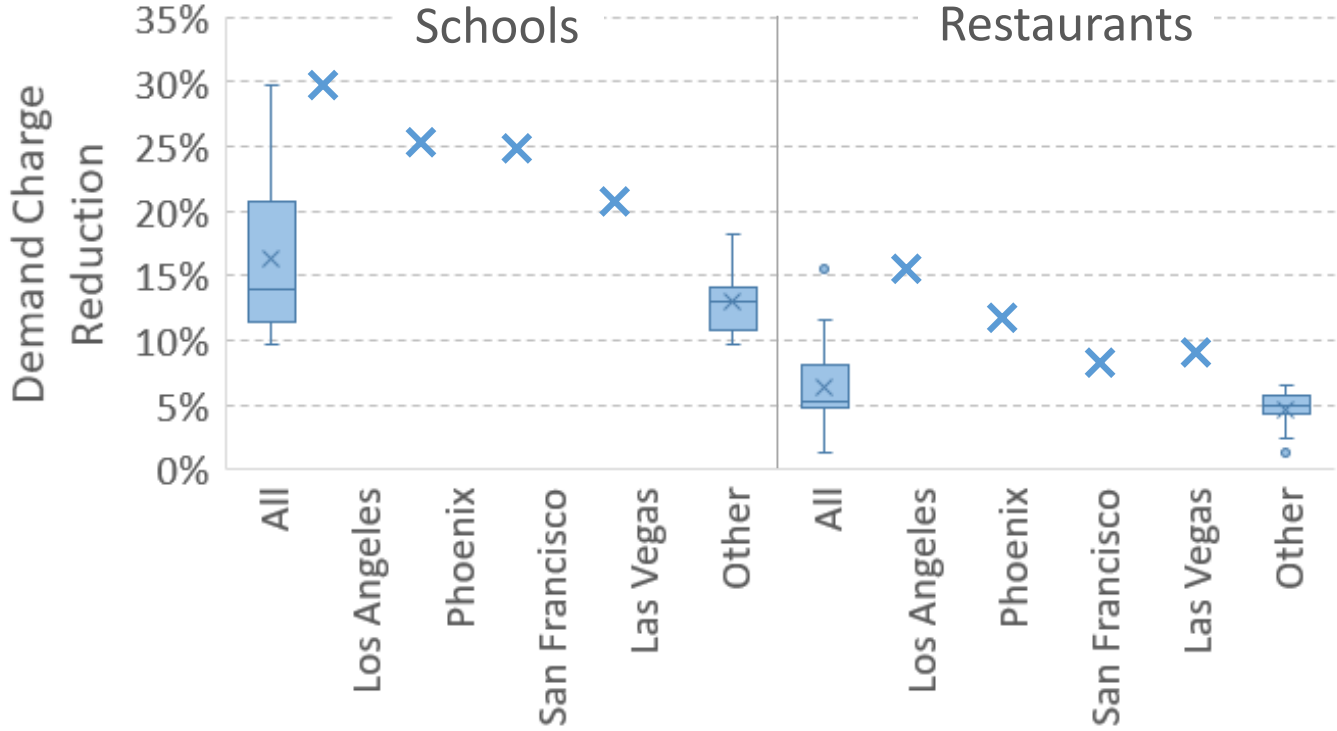
Percentage non-coincident demand charge reduction for schools (left) and restaurants (right) in various locations
