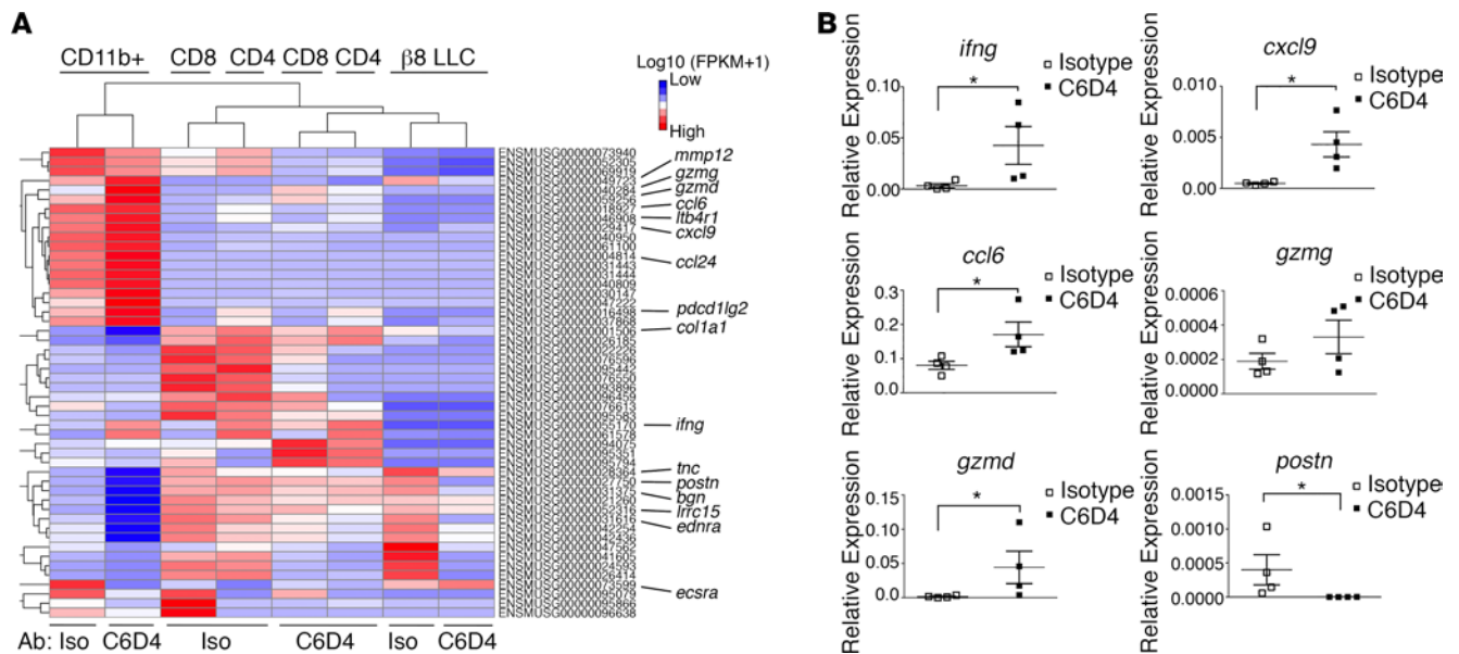
Figure 5. Differential gene expression by tumor cells, CD4 + T cells, CD8 + T cells, and CD11b + cells reveals a role for \beta 8 in suppression of a tumor-eliminating macrophage signature. (A) Heatmap of hierarchical clustering of differentially expressed (DE) genes determined by RNAseq across pooled CD11b + , CD4 + , CD8 + T cells, and \beta 8 LLC tumor cell samples isolated from mice ( n = 10 in each group) treated with isotype or C6D4 (7 mg/kg i.p.) on days 5 or 12 after \beta 8 LLC tumor cell injection. Tumors were harvested on day 15 after tumor cell injection. Hierarchical clustering analysis was carried out with the \log_{10} (FPKM+1) of union of DE genes. DE was defined by q < 0.005 and |\log_2(\text{fold change})| > 1 . Red represents highly expressed genes. Blue represents genes with low expression. Color gradient from red to blue reflects \log_{10} (FPKM+1) values from large to small. ENSEMBL IDs are shown, and select gene names are indicated. The majority (60%) of DE genes were found in macrophages (18 up; 12 down), which drives the clustering of T cells to be defined by antibody treatment rather than CD4 + or CD8 + lineage. (B) Validation of key macrophage DE genes from RNA isolated from pooled macrophage samples ( n = 4 pools) that had sorted for purity (CD45 + , F4/80, CD11b + ) and assessed by qPCR for ifng , cxcl9 , ccl6 , gzm , gzmd , and postn . Shown is expression ( 2^{-\Delta ct} ) relative to hprt . * P < 0.05 by unpaired Mann-Whitney U test.
