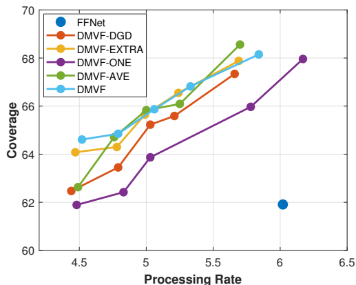
Figure 8: Comparison between DMVF with different consensus algorithms and FFNet.
