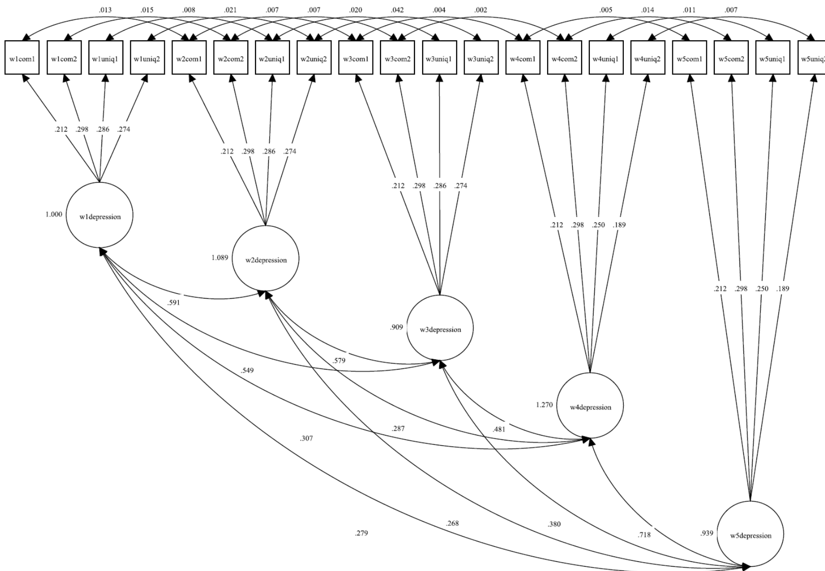
Figure 3. Partial strong factorial invariance model for youth's depressive symptoms with unstandardized parameter coefficients for Waves 1-5.
