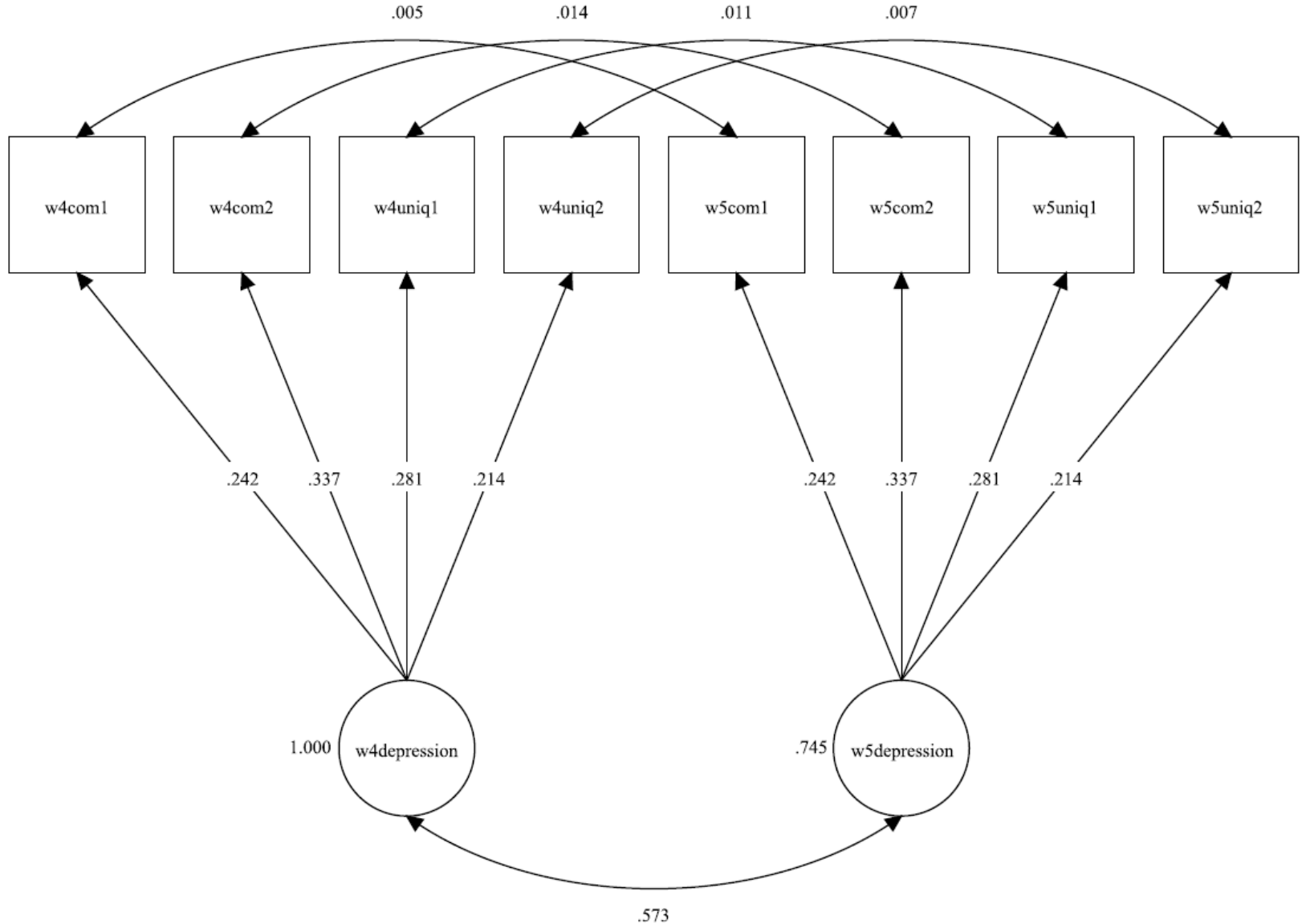
Figure 2. Strict factorial invariance model for youth's depressive symptoms with unstandardized parameter coefficients for Waves 4-5.
