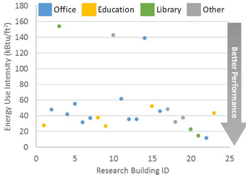
Figure 4: Individual building EUIs of the research building set color-coded by building type. n=23
