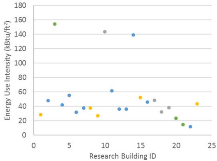
Figure 7: Total site building energy use of the research building dataset n=23
