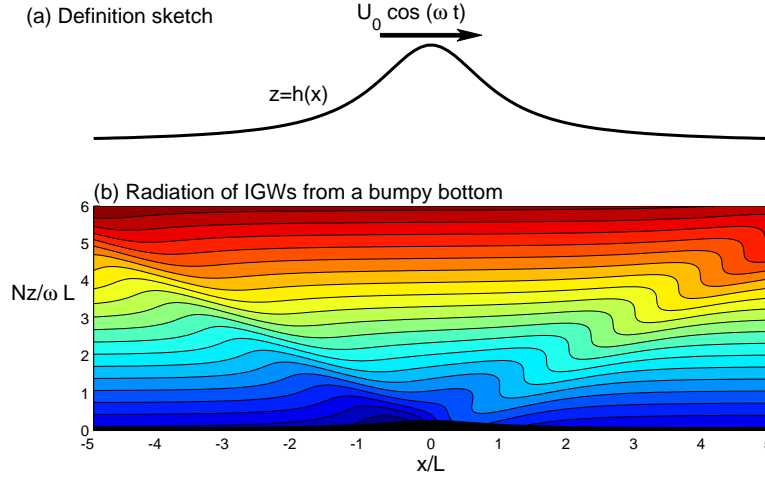
FIGURE 1. Model topography (a) and buoyancy field computed in WTA limit (b).
