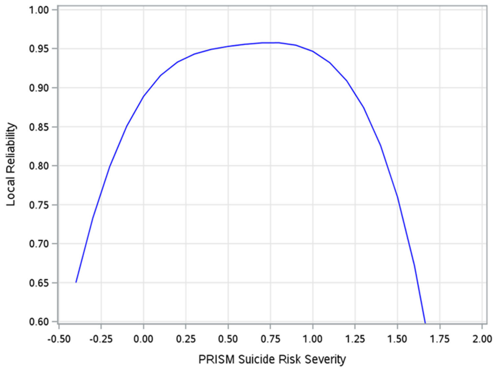
Figure 1. Local Reliability Plot: PRISM Suicidality IRT Scores
