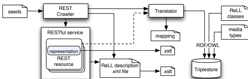
Figure 9: Implementation
