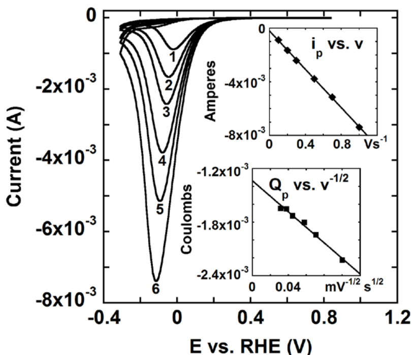
Figure 3. Cyclic voltammograms of oxygen saturated 0.5 mol dm -3 H 2 SO 4 solution recorded for 5.7% CoPC on Vulcan XC72. Total carbon loading 0.1 mg. Equilibration time 5 min at 400 rpm. R = 1.8. Scan rate (mV s -1 ): 100 (1), 200 (2), 300 (3), 500 (4), 700 (5), 1000 (6). Top inset: peak current vs. scan rate. Bottom inset: oxygen reduction charge plotted vs. inverse square root of the scan rate (see text for the charge determination methodology).
