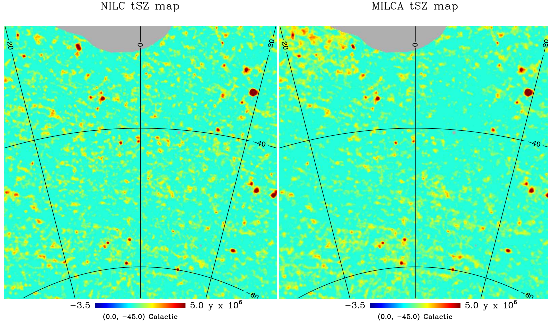
Fig. 2. A small region of the reconstructed Planck all-sky Compton parameter maps for NILC ( left ) and MILCA ( right ) at intermediate Galactic latitudes in the southern sky.
