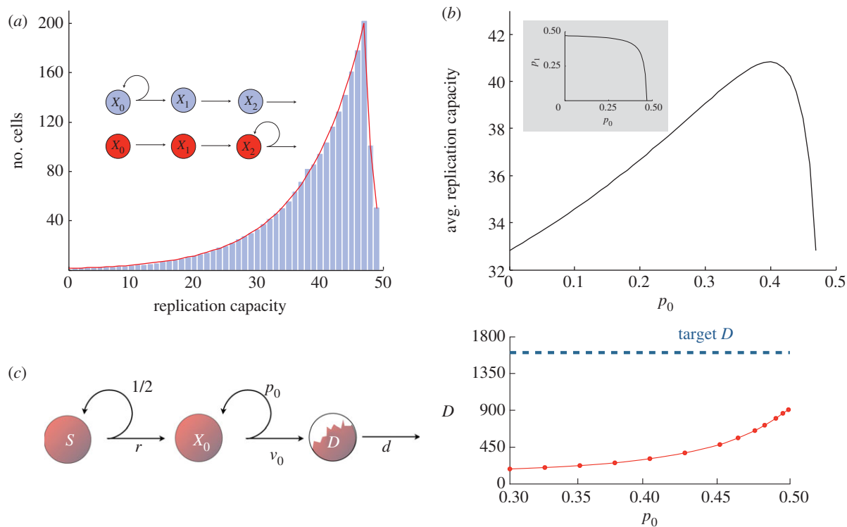
Figure 3. (a) Distribution of the replication capacity of dividing cells ( k = 2, r = 1, v_j = 1, S = 50, \rho = 50, p_0 or p_2 = 0.45 ). Here self-renewal occurs only in one transit-amplifying cell compartment. Bar plots are produced using the agent-based model and allowing for self-renewal only in compartment 0. Red line is produced using the analytical model allowing for self-renewal only in compartment 2. The distribution does not change when the non-zero self-renewal probability is switched from compartment 0 to compartment 2. See proposition 5.2. (Stem cell and differentiated cell compartments are not depicted in the inset.) (b) Replication capacity of the entire cell population at equilibrium as a function of p_0 ( k = 1, v = 1, dD - rS = 1716, \rho = 50 ). Given that dD - rS is fixed the value of p_0 = 0 determines the value of p_1 (see inset). Note that the minimum occurs when there is self-renewal in only one of the compartments (i.e. p_0 or p_1 is equal to zero). See lemma 5.4. (c) It is not always possible to reach a specified target number of divisions with only one intermediate compartment. Here, the number of differentiated cells produced by a system with a single intermediate compartment is incapable of producing the target number of differentiated cells (indicated by a half-filled compartment D ). In this case, rS = 50, D = 1600, d = 1 and \rho = 20 . Results were obtained using the agent-based model. (See text for discussion.)
