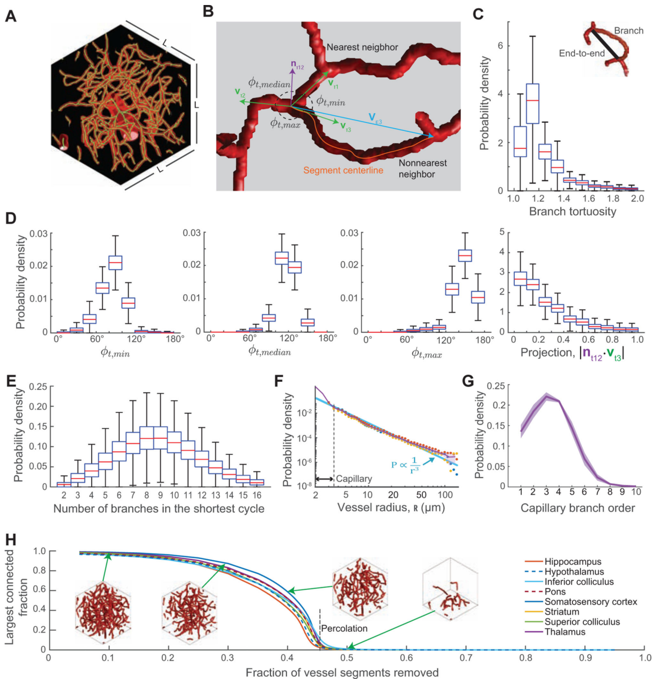
Figure 3. Common network topology and branch and node geometry across all brains.
