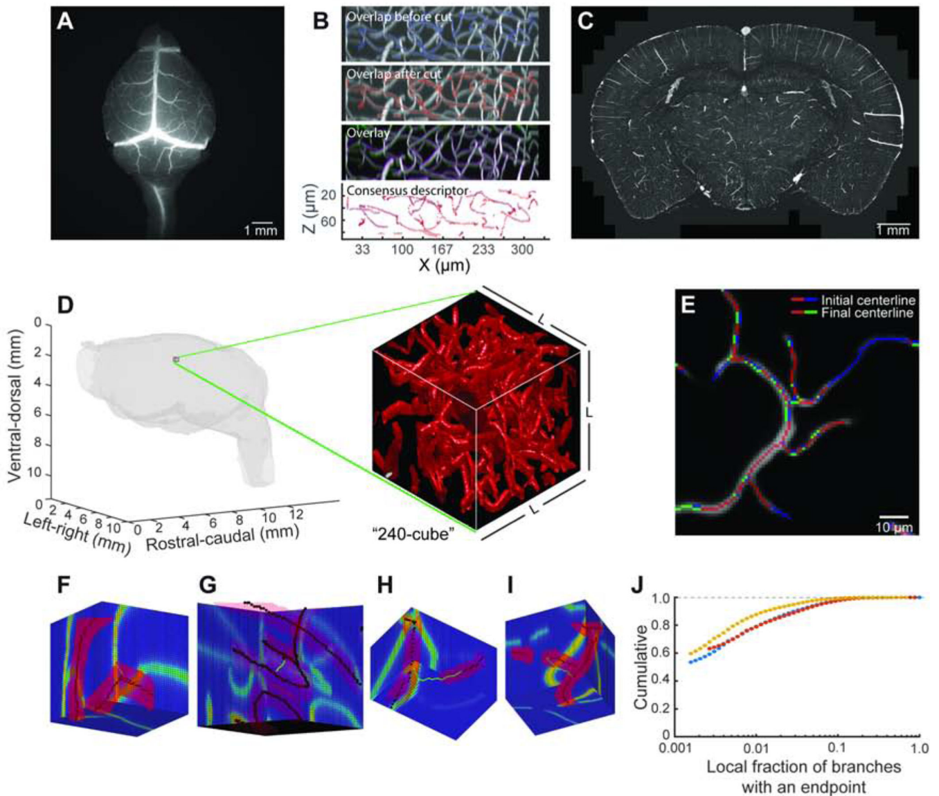
Figure 1. Sample preparation, imaging, image processing and vascular graph reconstruction.
