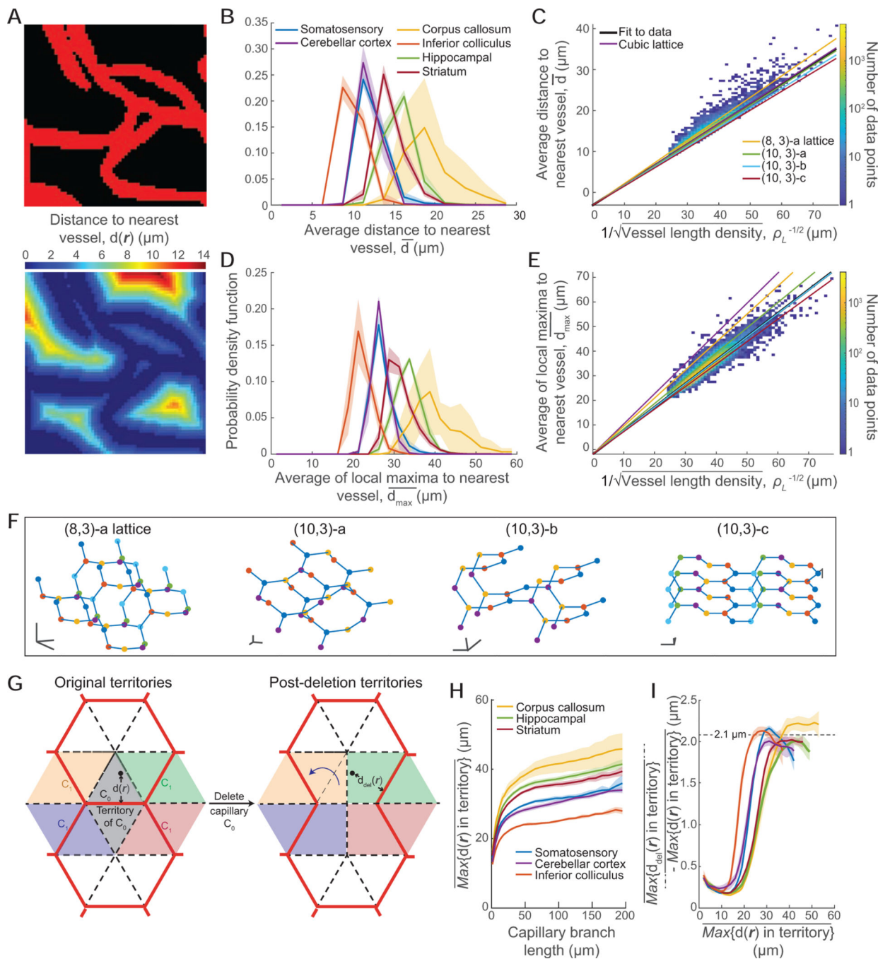
Figure 6. Scaling relations of space-filling networks.
