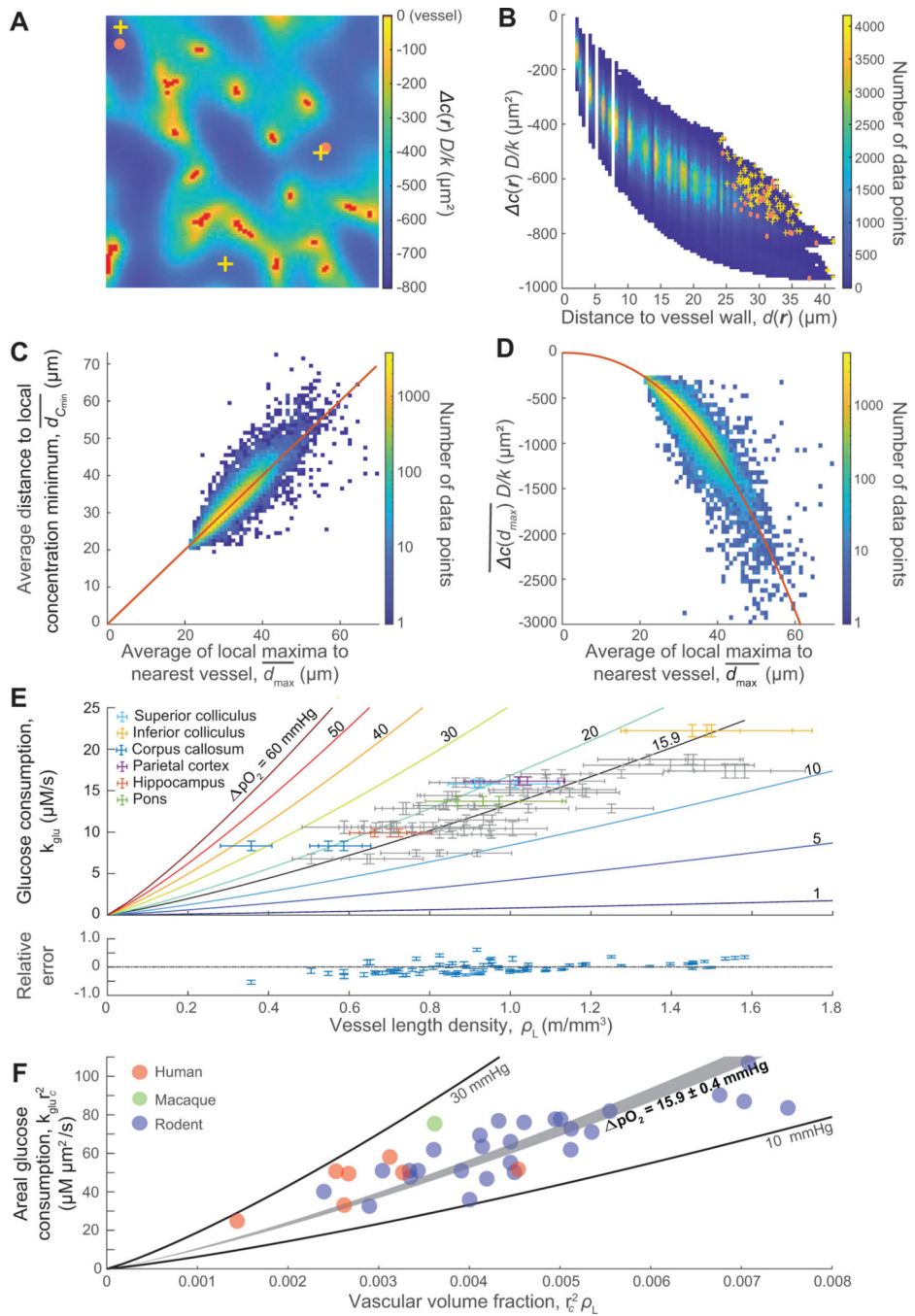
Figure 7. Numerical and analytical calculations of substrate diffusion and regional glucose metabolism in terms of vessel length density
