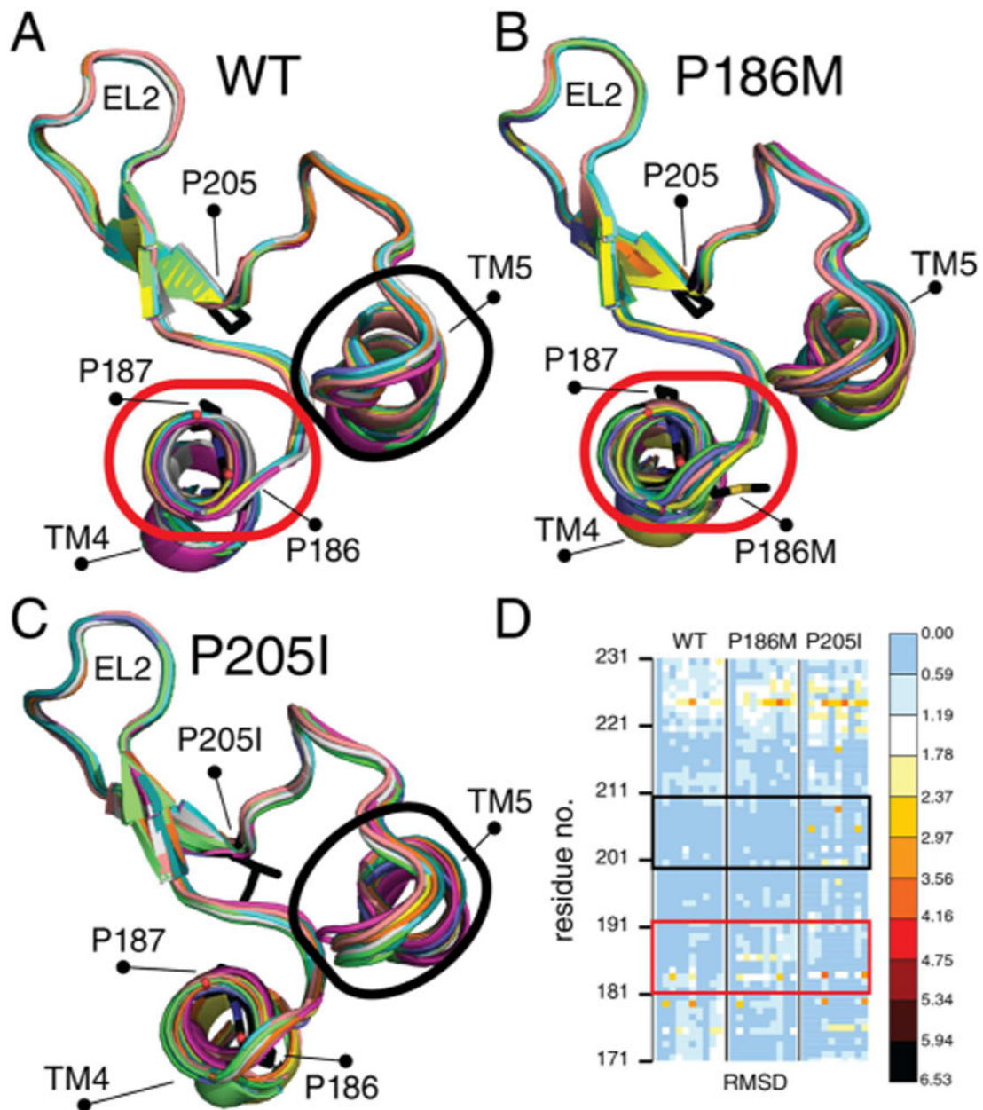
Figure 5. Structural models and RMSD analysis of EL2 in WT green opsin and its P186M and P205I substitutions. The 10 energetically favored structures were aligned and are displayed as cartoons from residue 180 to 224. (A) The Pro-Pro motif in the WT green opsin is highlighted with a red oval. The black oval indicates the region of variation in the structure caused by the P205I mutation. (B) Structures resulting from the P186M mutation. The red oval indicates a major variation in structure induced by the mutation (compare with the red oval region in panel A). (C) Major variations in structure are caused by the P205I mutation (black oval; compare to the black oval region in panel A). (D) Heat map of RMSD analysis of the 10 energetically favored structures shown in panels A–C. The red and black rectangles correspond to the ovals displayed in A–C.
