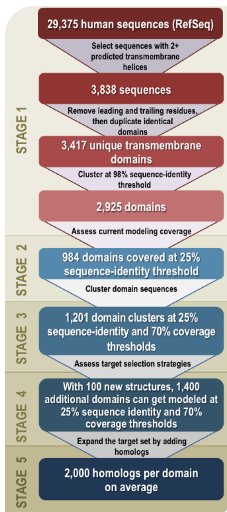
Figure 1. Flowchart of the analysis (Supplementary Notes 1 and 2)
