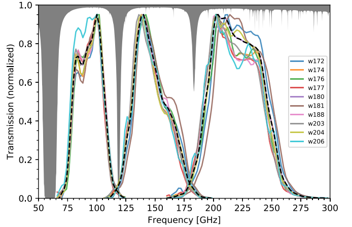
Figure 7. Frequency response, g(\nu) , of the SPT-3G receiver at 95, 150, and 220 GHz to a beam-filling, flat-spectrum source. The solid lines show the response averaged by detector wafer, and the dashed line is the average response across all ten wafers. The gray shaded region indicates atmospheric absorption for 0.25 mm precipitable water vapor at the South Pole. The frequency response has been arbitrarily normalized. The power on the detector, P , for a source with a spectrum, I(\nu) , would be P = \int \eta_g g(\nu)I(\nu)d\nu , where \eta_g is the optical efficiency.
