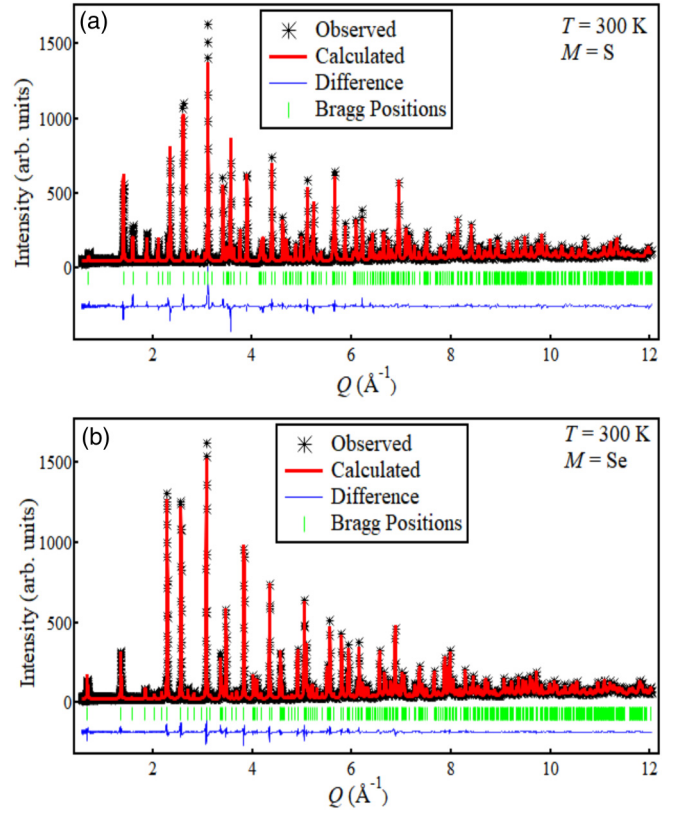
FIG. 2. Neutron Rietveld refinement of the nuclear model of (a) M = \text{S} and (b) M = \text{Se} at 300 K as a function of momentum transfer Q . The details of the fit are provided in the text.
