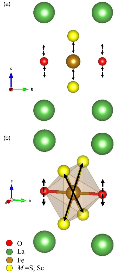
FIG. 6. Panel (a) shows possible Fe and Se/S atomic movement within the \text{La}_2\text{O}_2\text{Fe}_2\text{O}(\text{S}, \text{Se})_2 octahedra that result in the bucking of the \text{Fe}_2\text{O} plane. (b) The dashed lines show Fe atom movement in the \text{Fe}_2\text{O} plane and the solid lines show Fe movement with respect to M .
